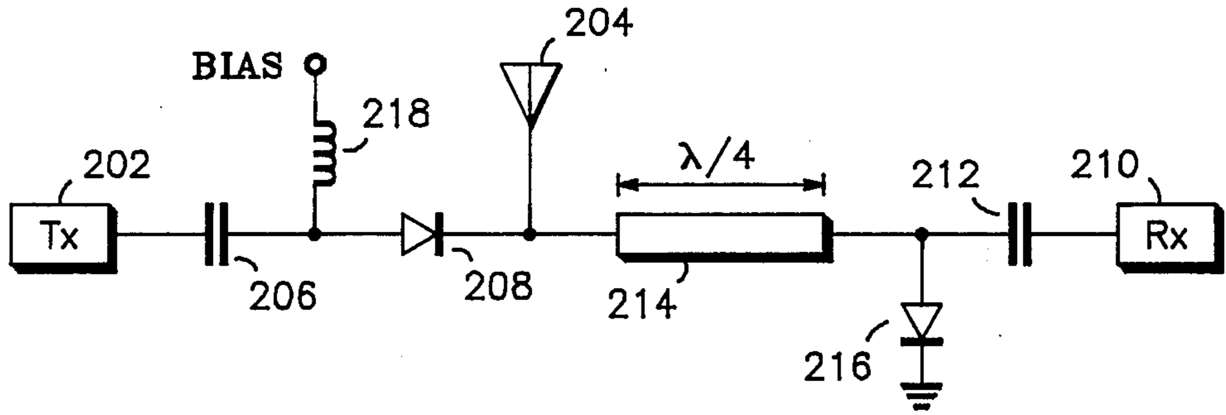
FIG. 2 -PRIOR ART-
