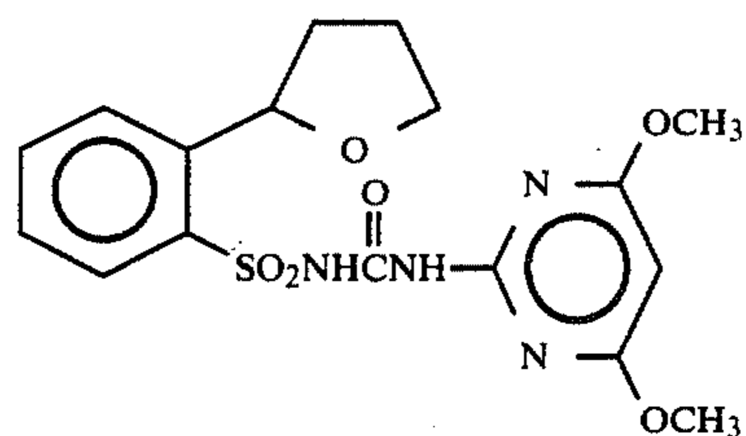
Compound 2 5
