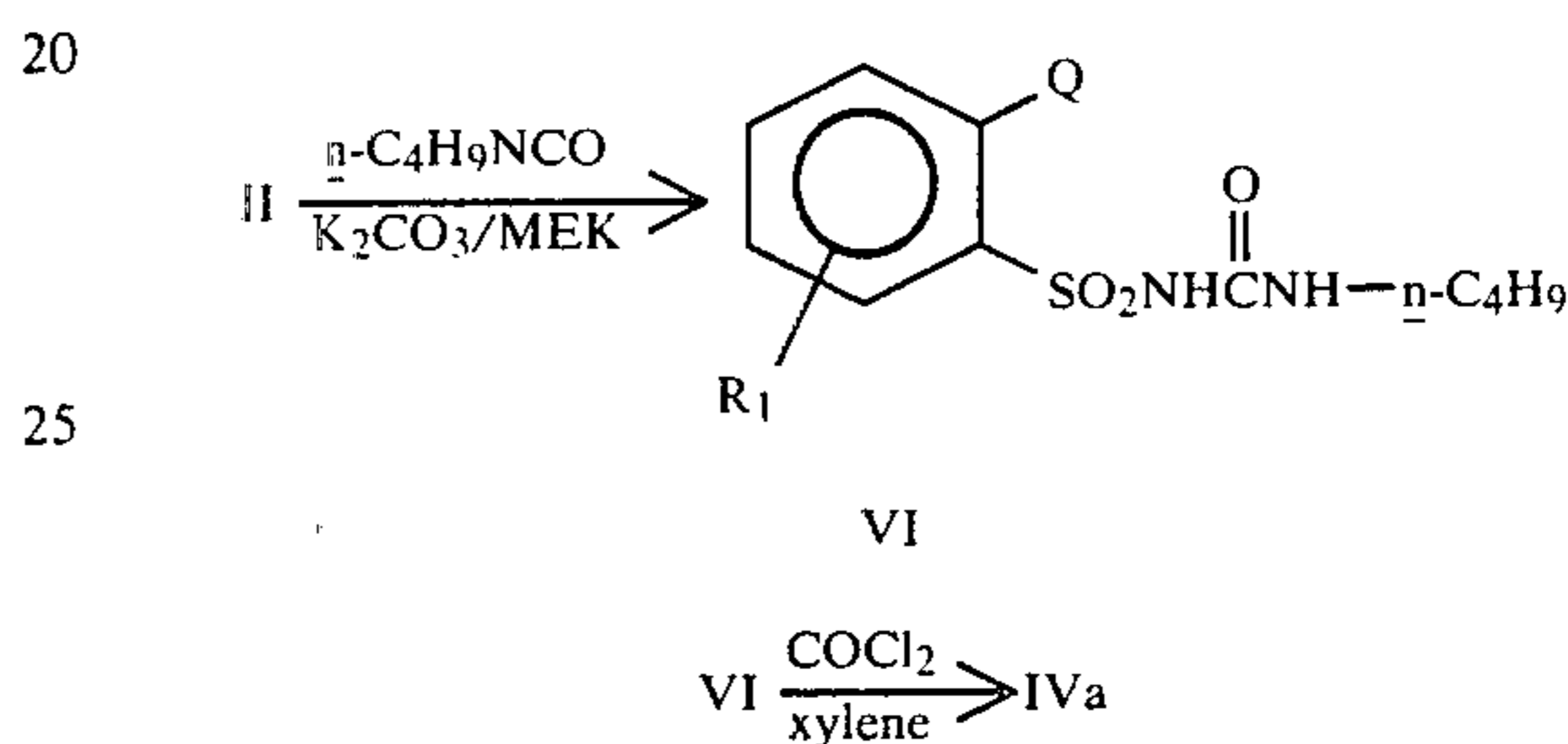
EQUATION 4
