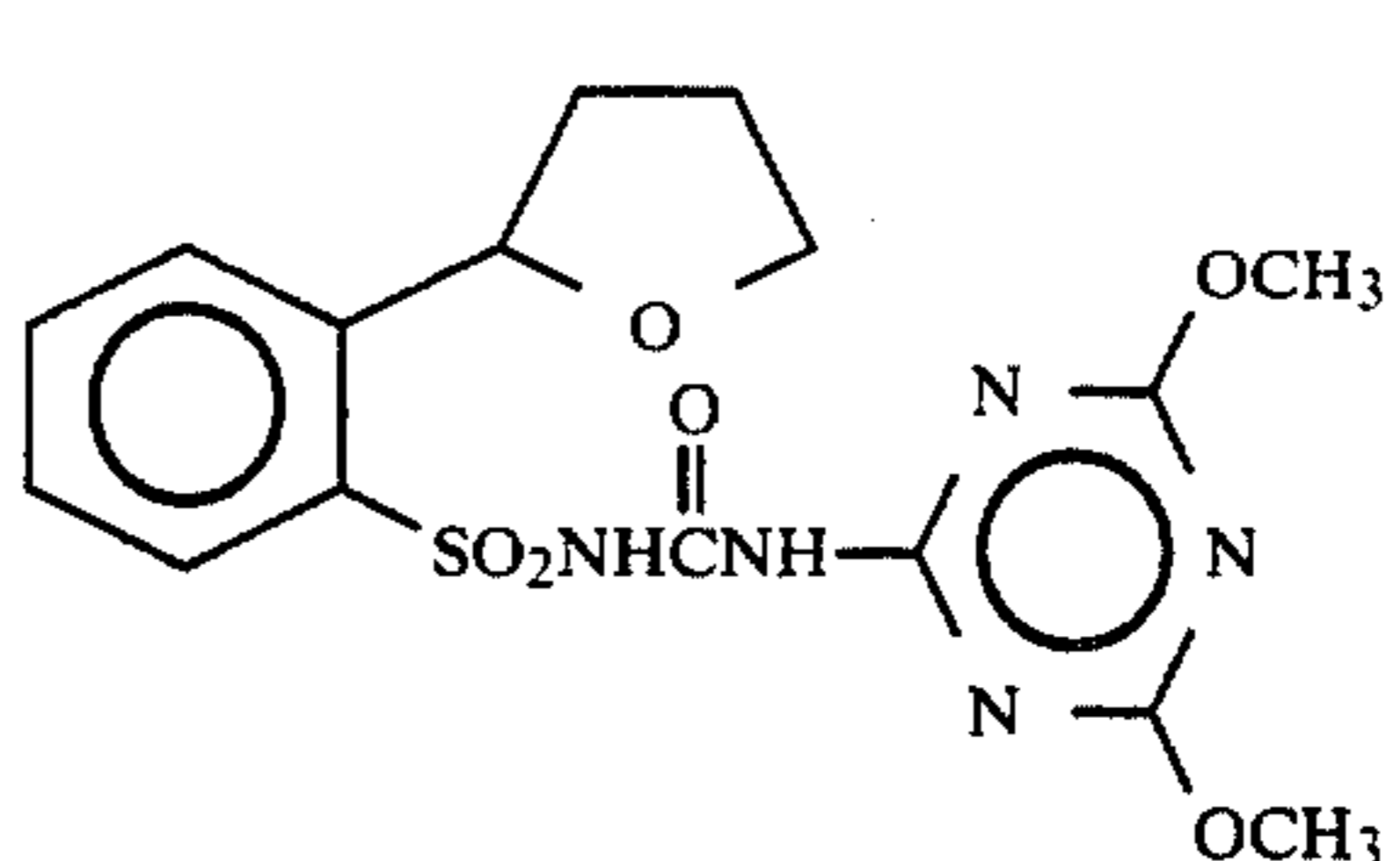
Compound 11 60
