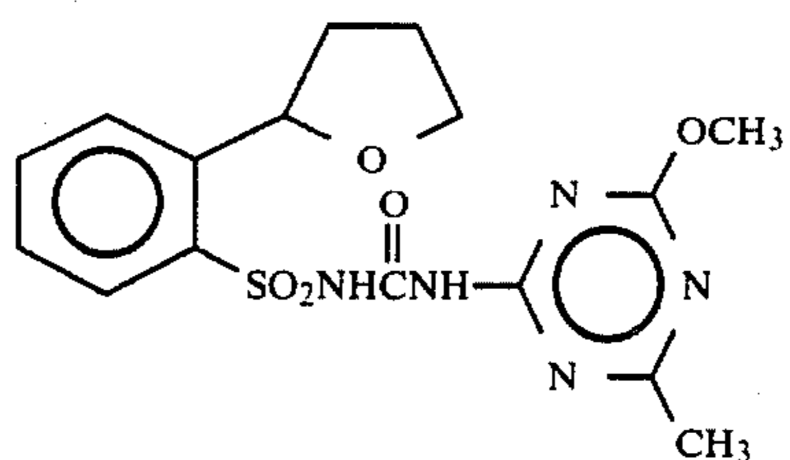
Compound 10 55
