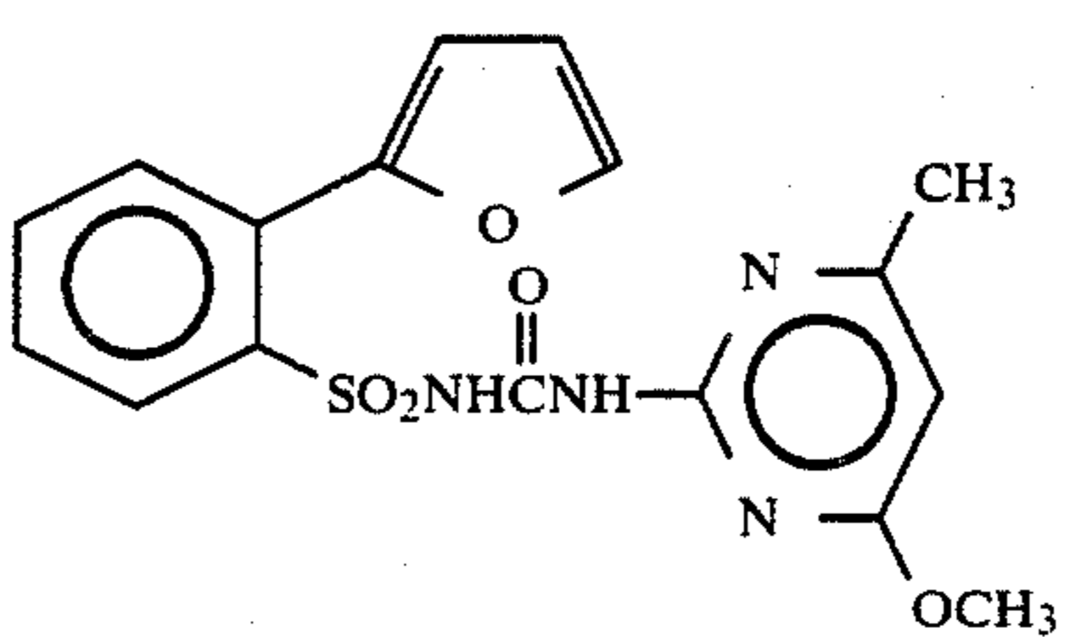
Compound 13 70
