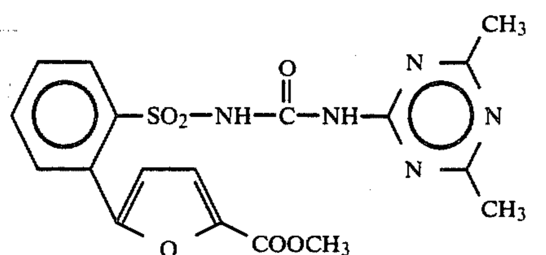
Compound 6 35
