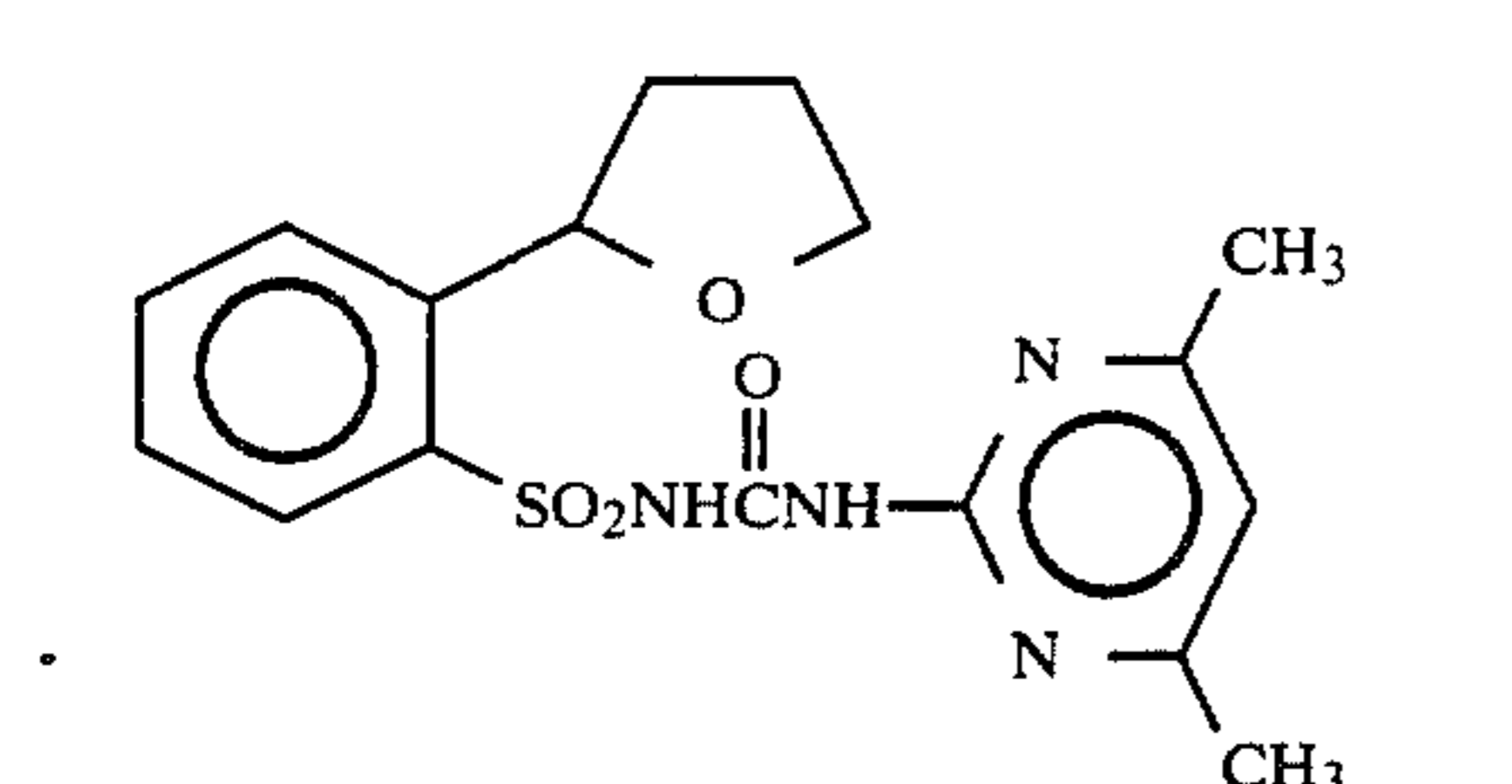
Compound 7 40
