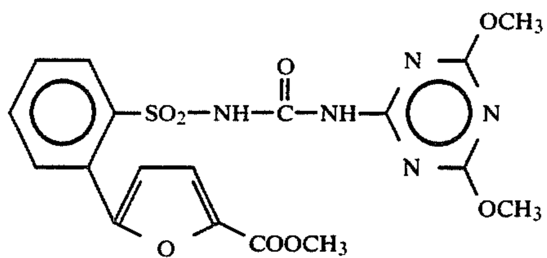
Compound 2 5
