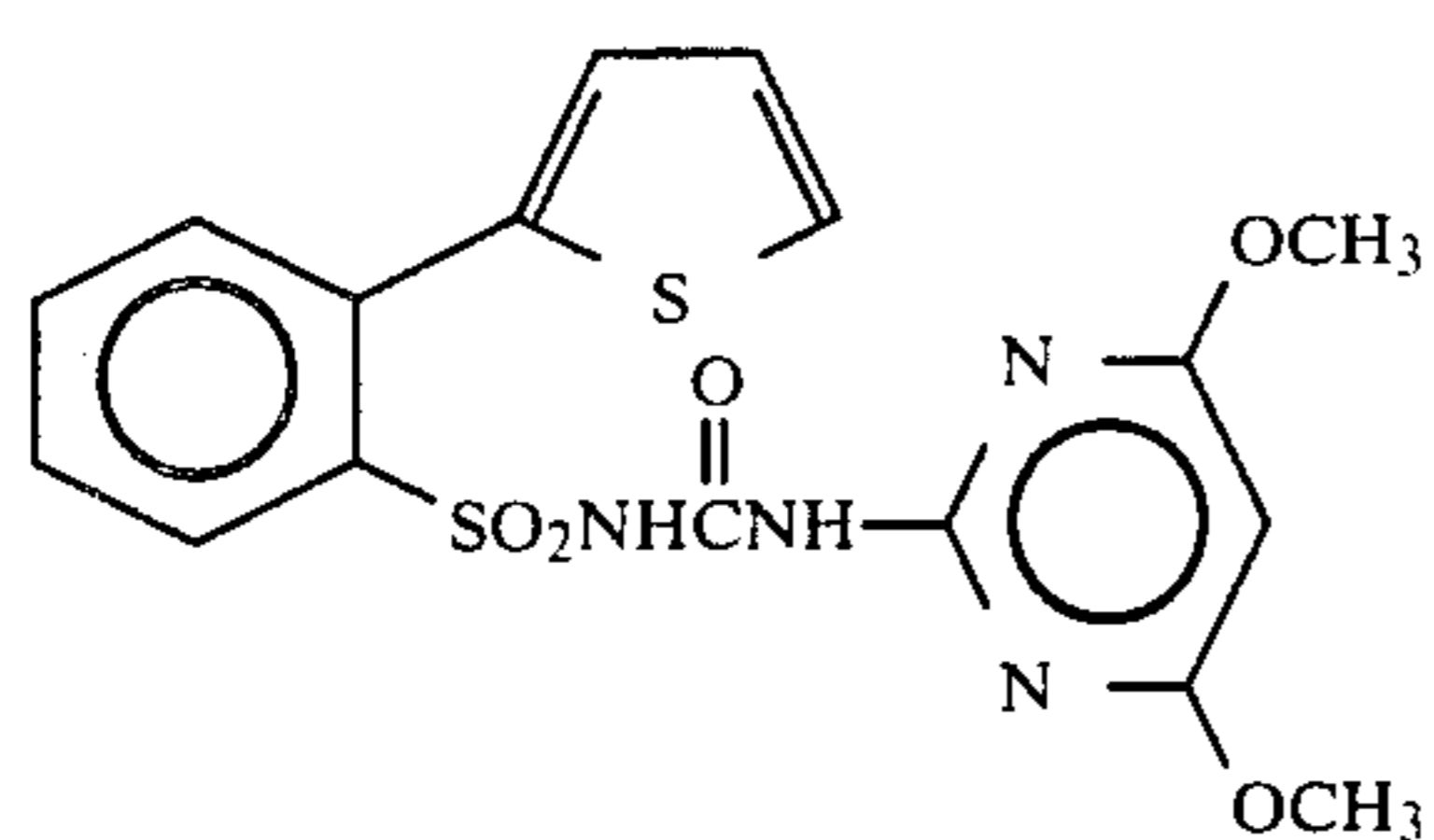
Compound 19 35
