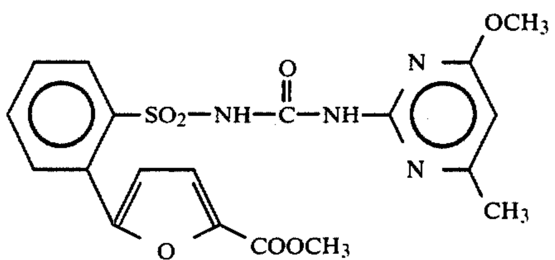
Compound 3 15
