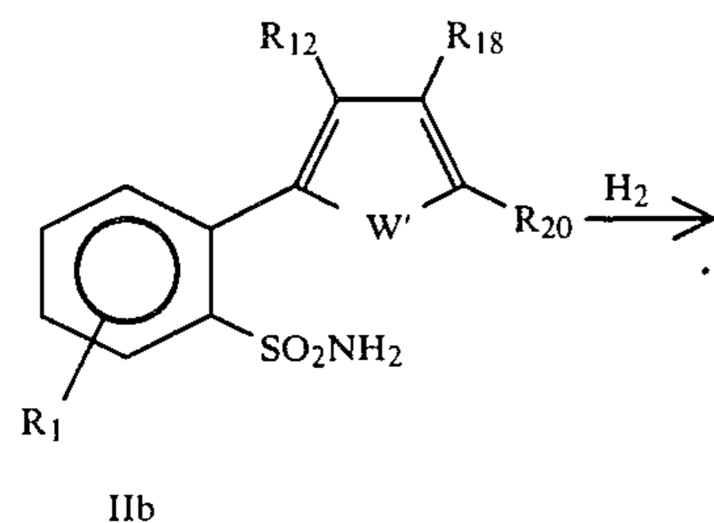
EQUATION 8
