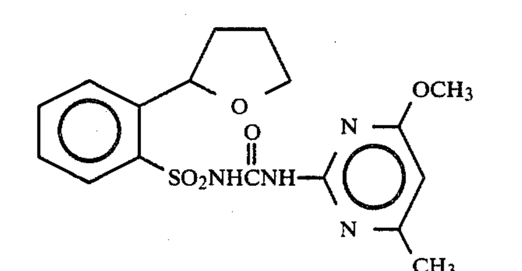
Compound 8 45
