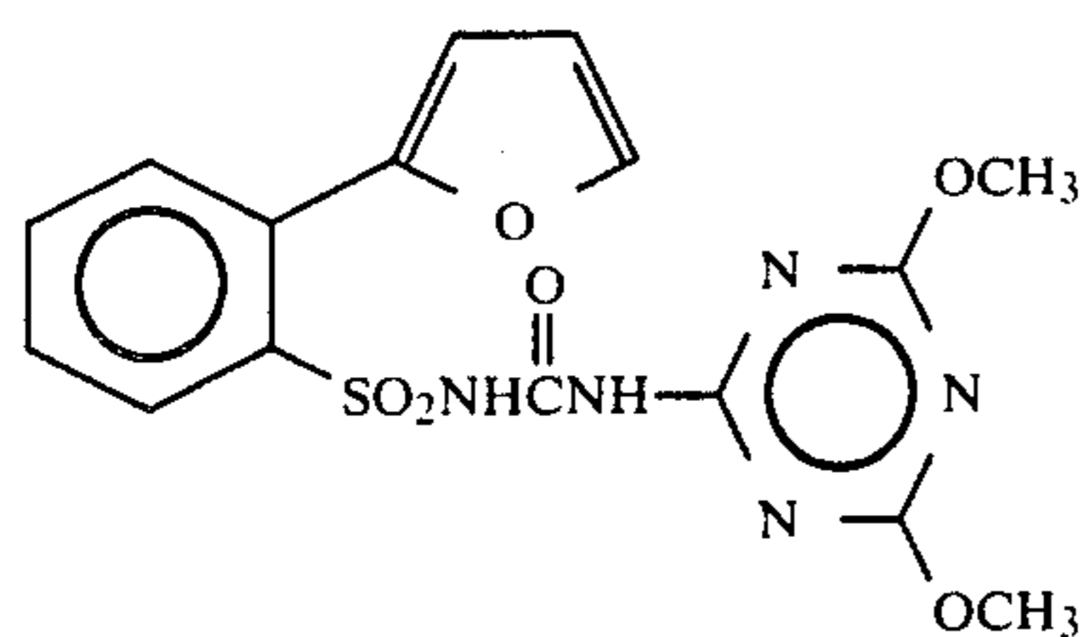
Compound 16 5
