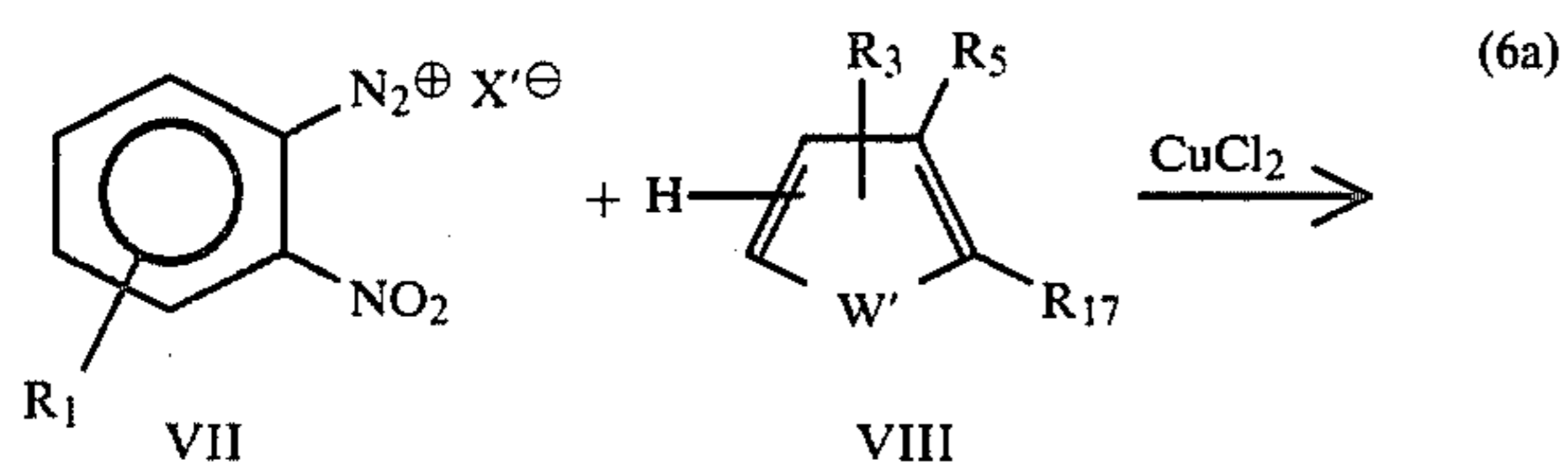
EQUATION 6
