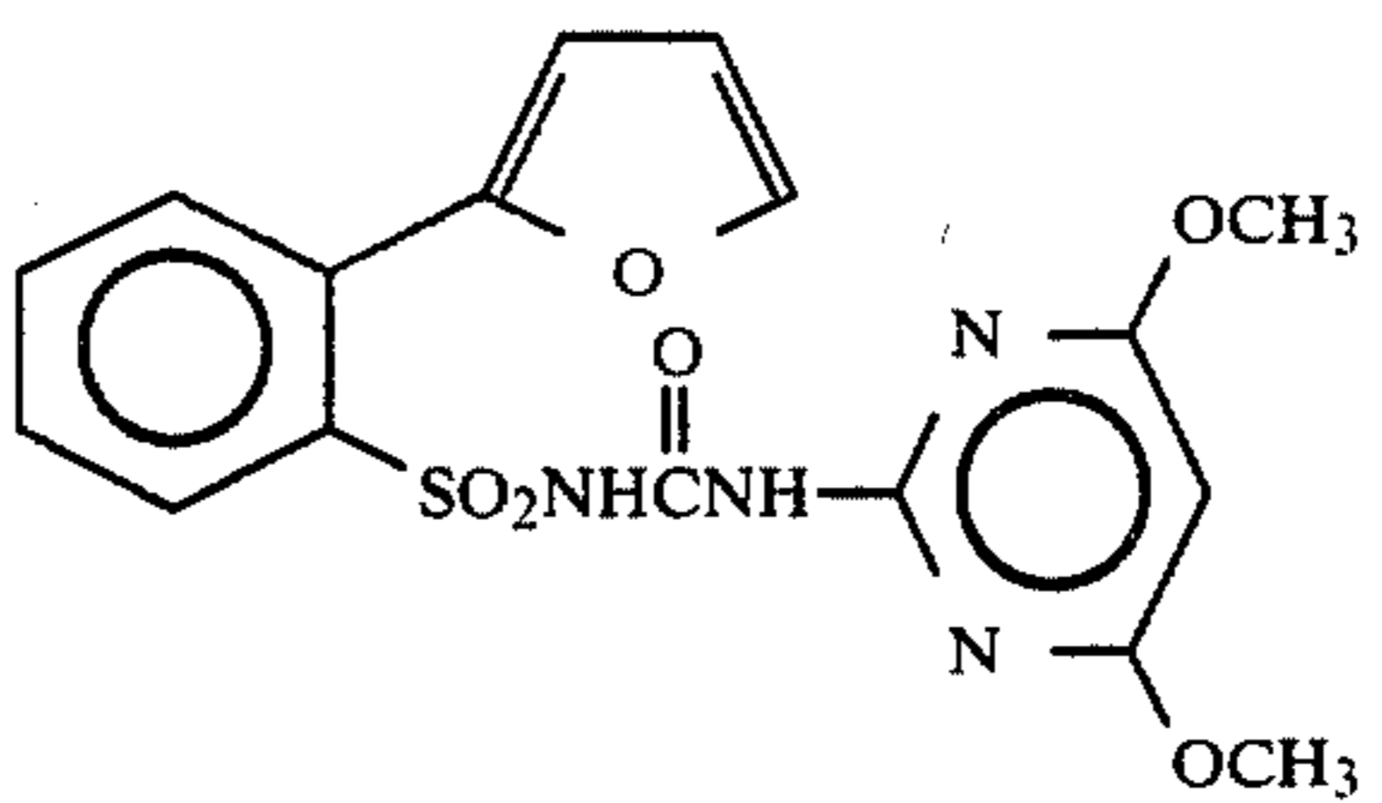
Compound 14 75
