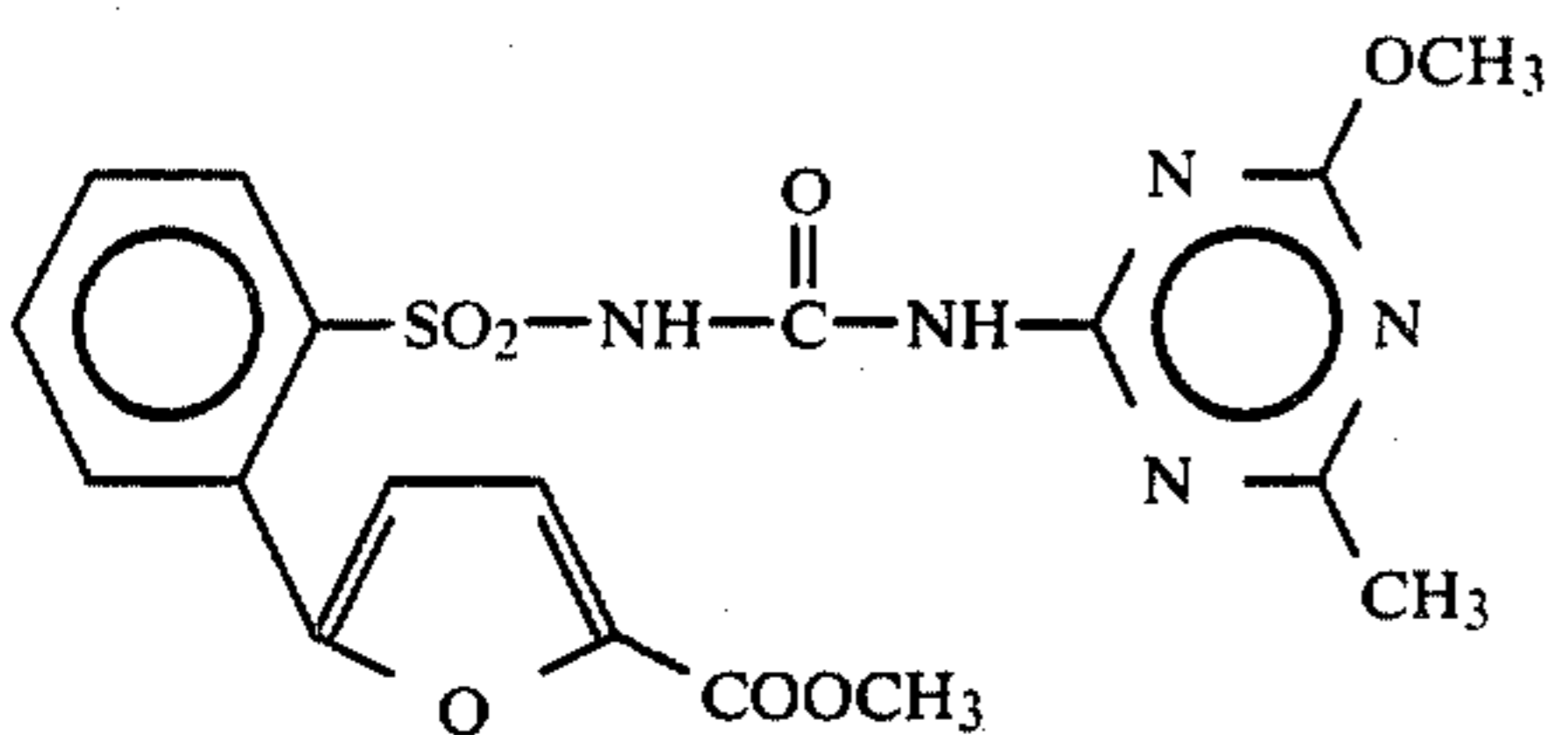
Compound 4 25
