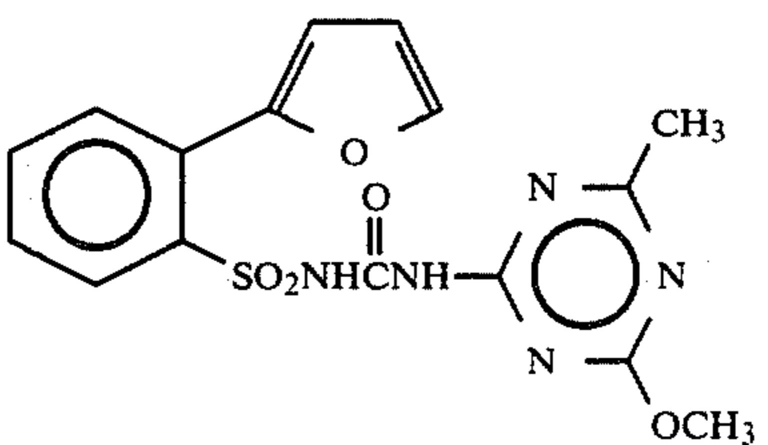
Compound 15 80
