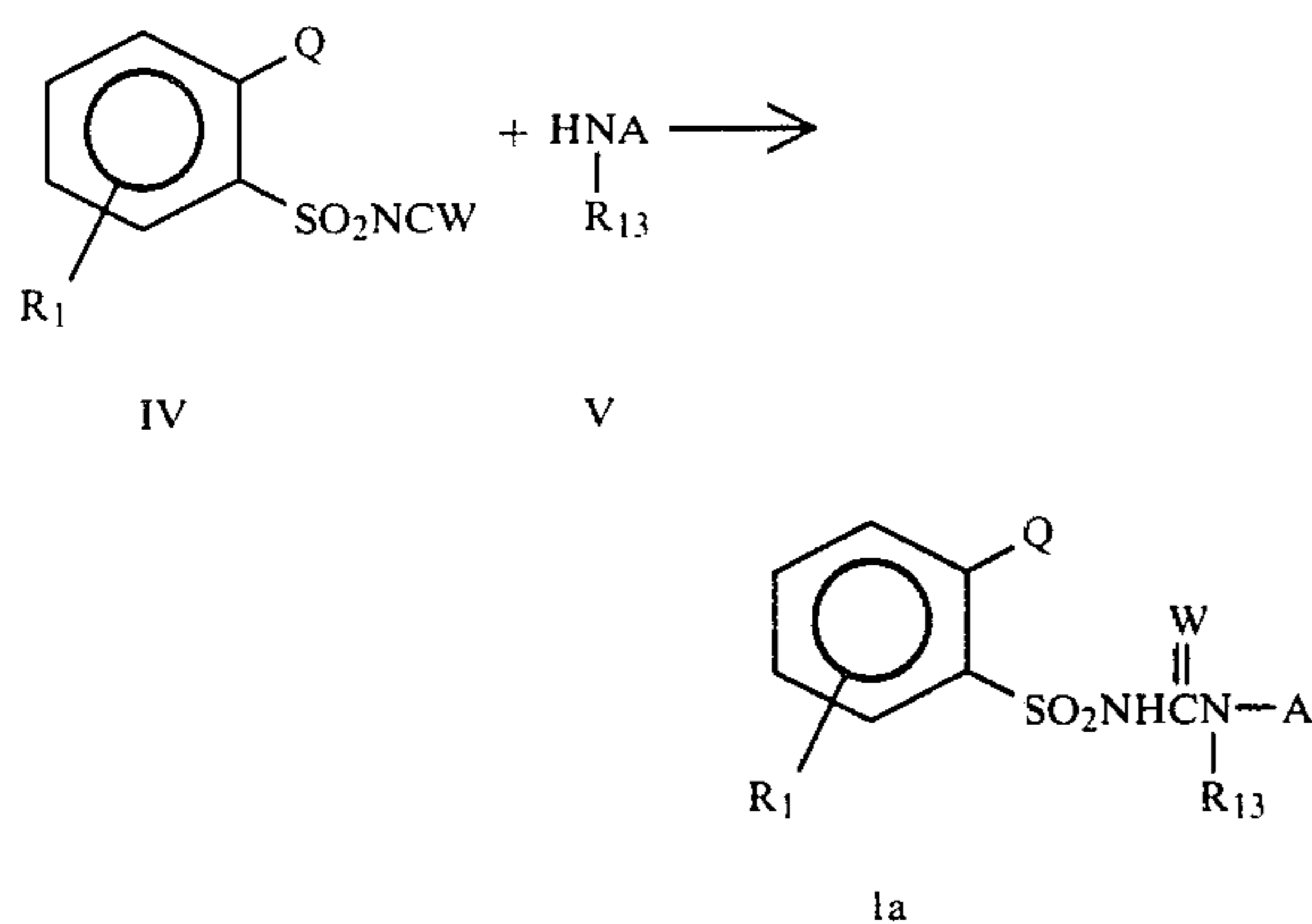
EQUATION 2
