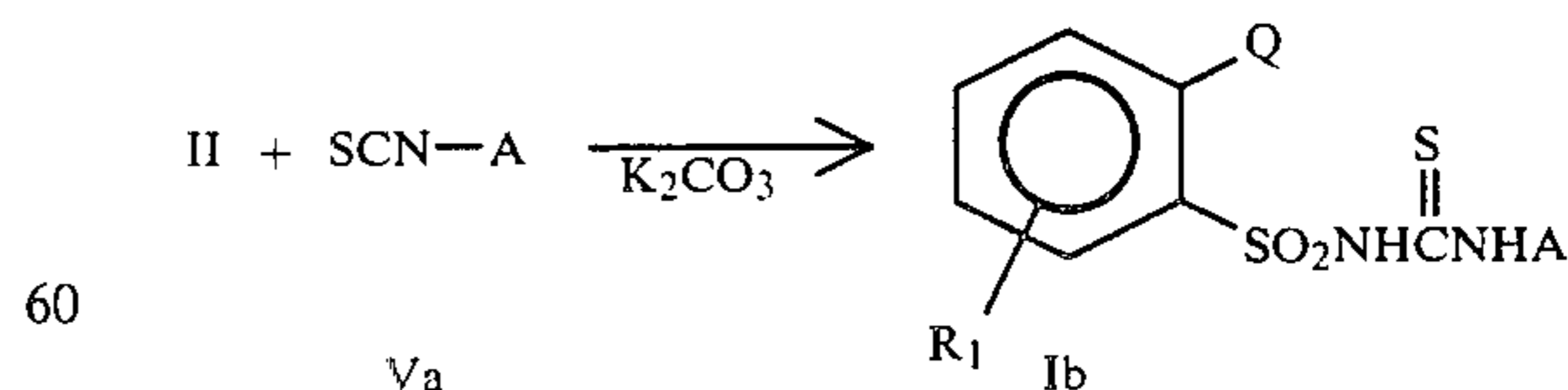
EQUATION 5
