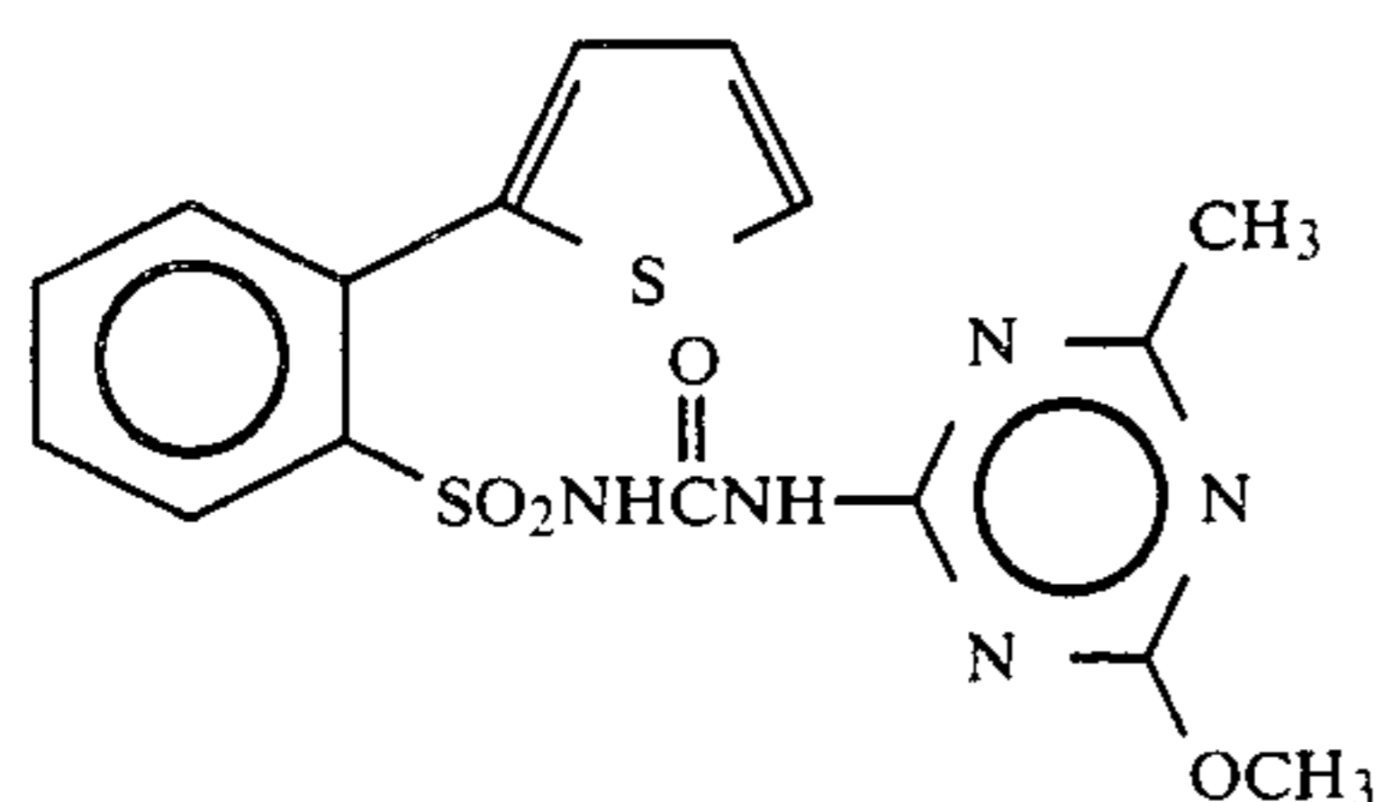
Compound 20 45
