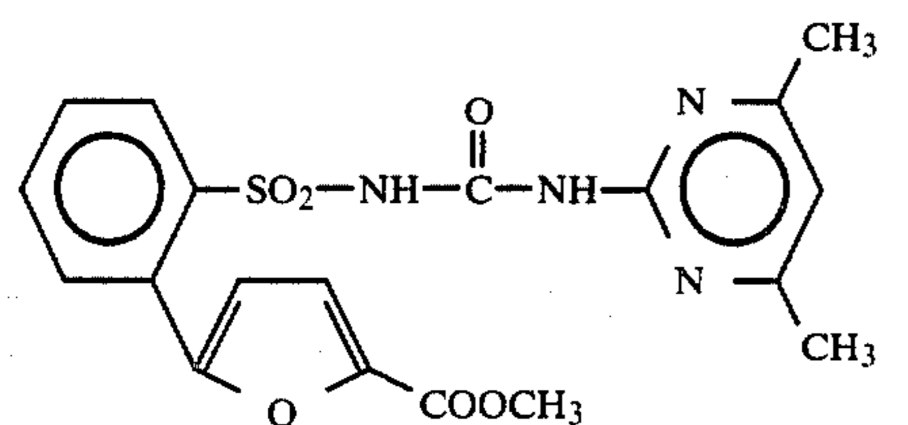
Compound 5 30
