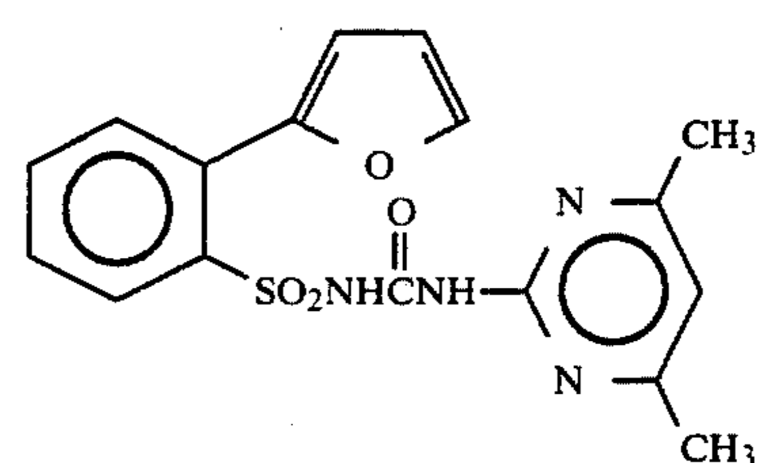
Compound 12 65
