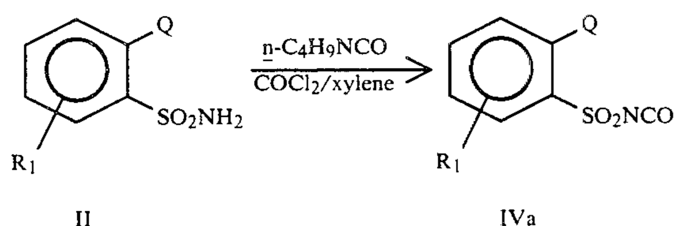
EQUATION 3
