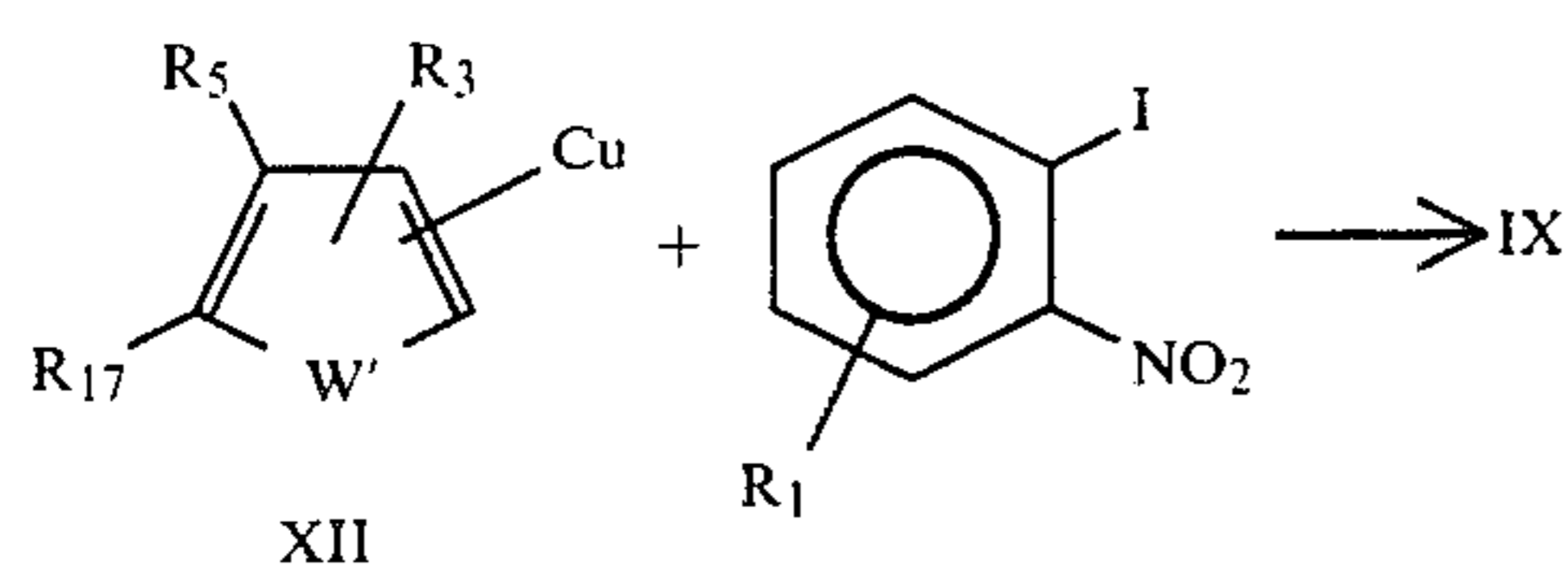
EQUATION 7
