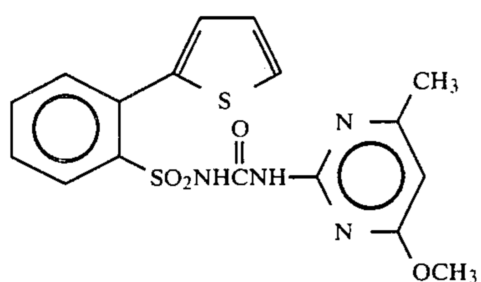
Compound 18 25
