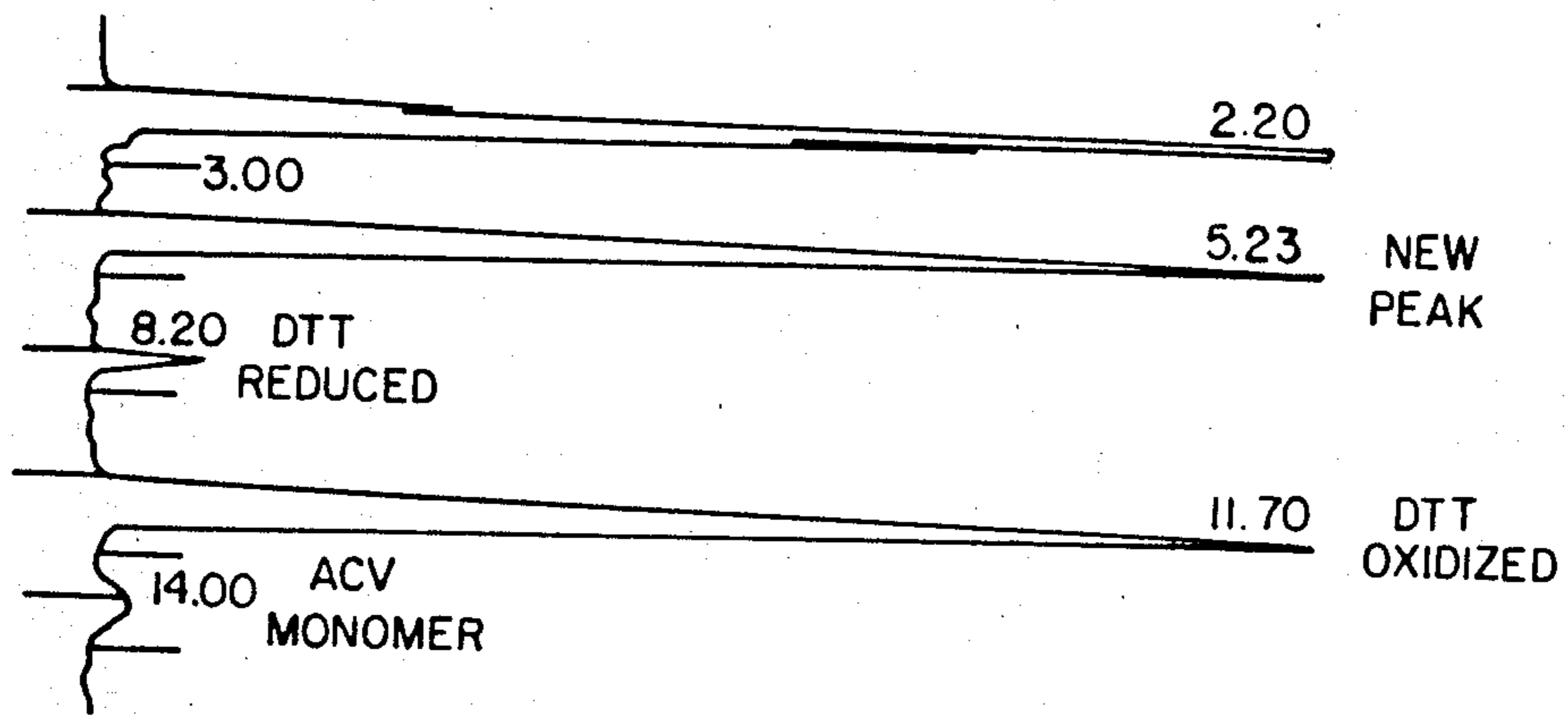
FIG. 1d 45 MIN. SAMPLE
