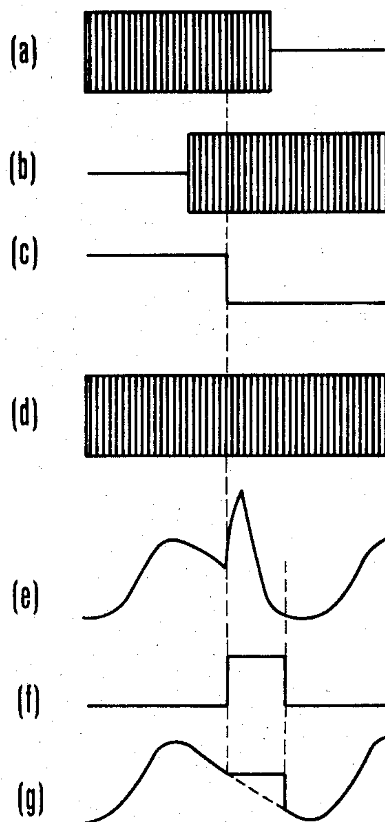
FIG. 4 PRIOR ART
