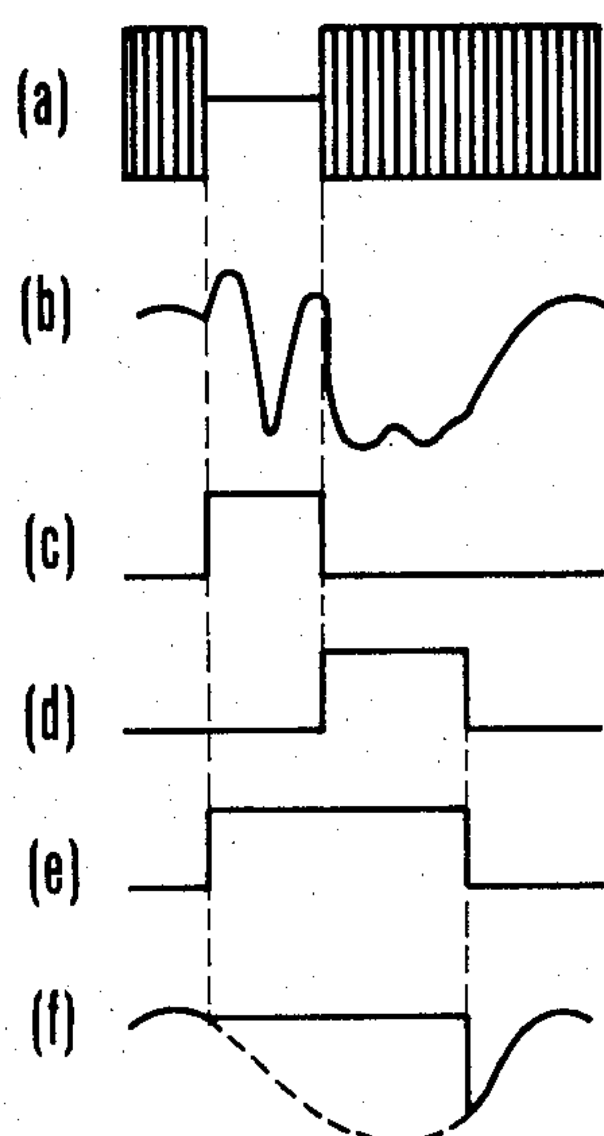
FIG. 2 PRIOR ART
