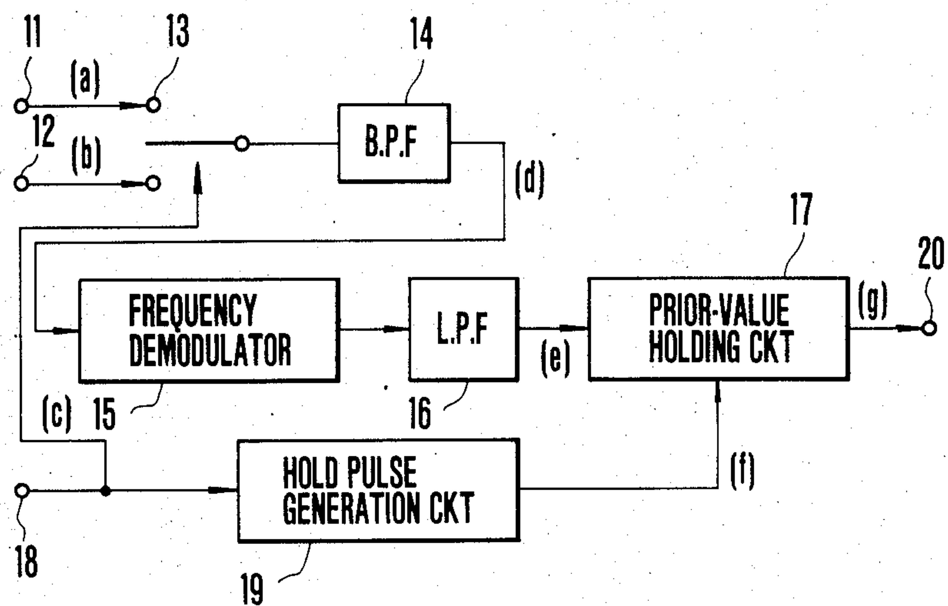
FIG. 4 PRIOR ART
