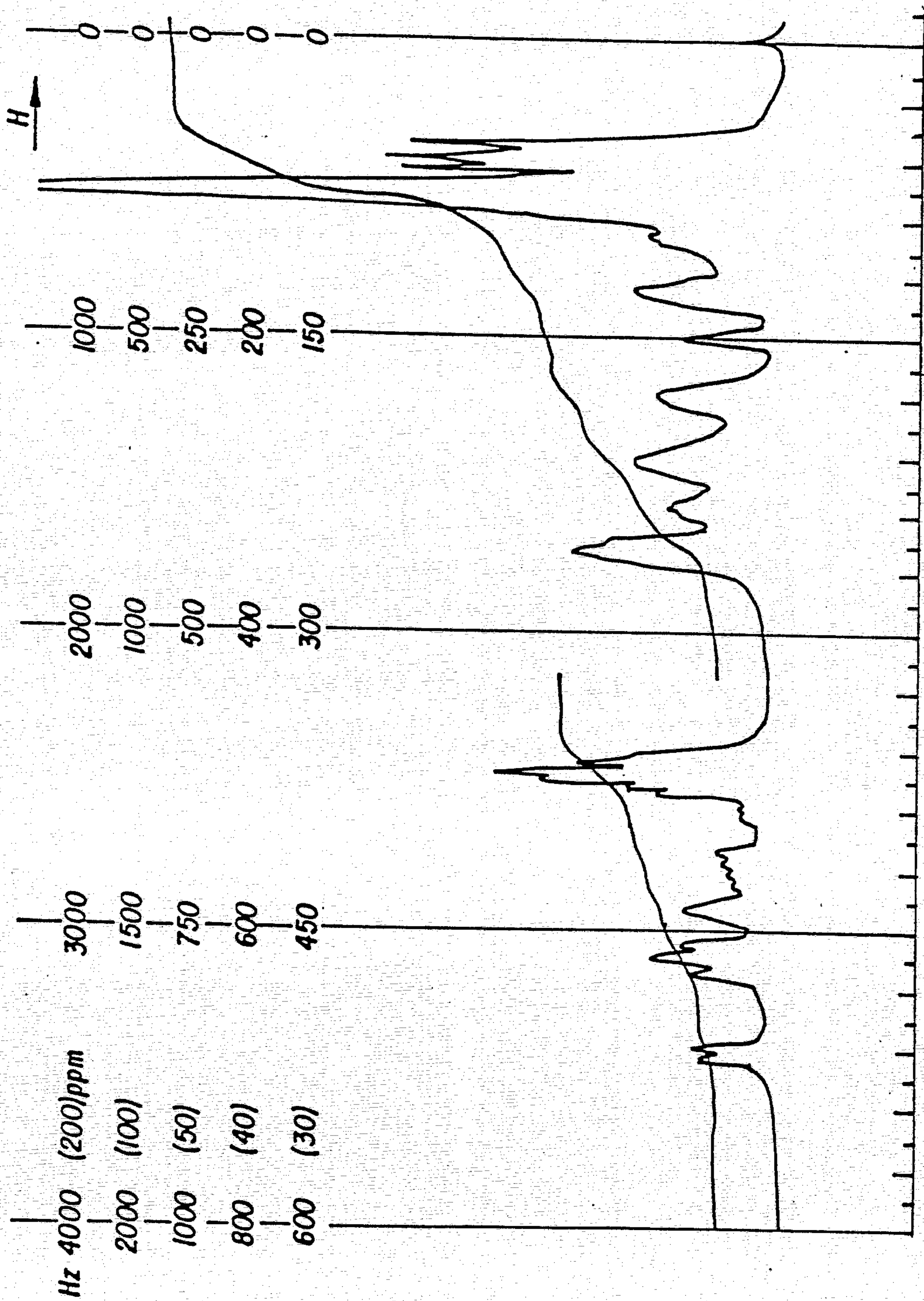
FIG. 4 ^1\text{H-NMR} SPECTRUM OF BU-2867T A (80 MHz, IN d_6\text{-DMSO} )
