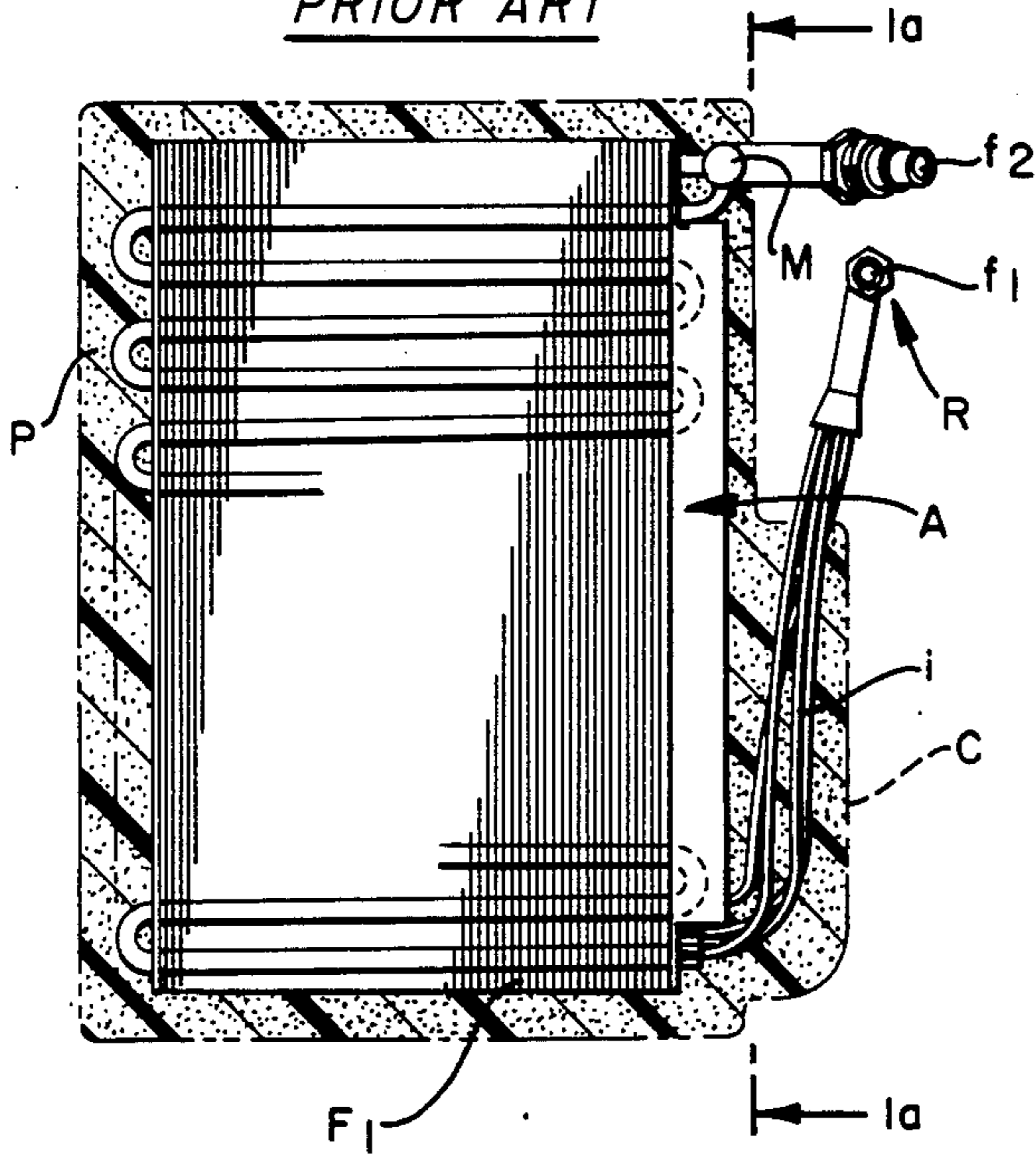
FIG. 2 "O.E.M." PRIOR ART
