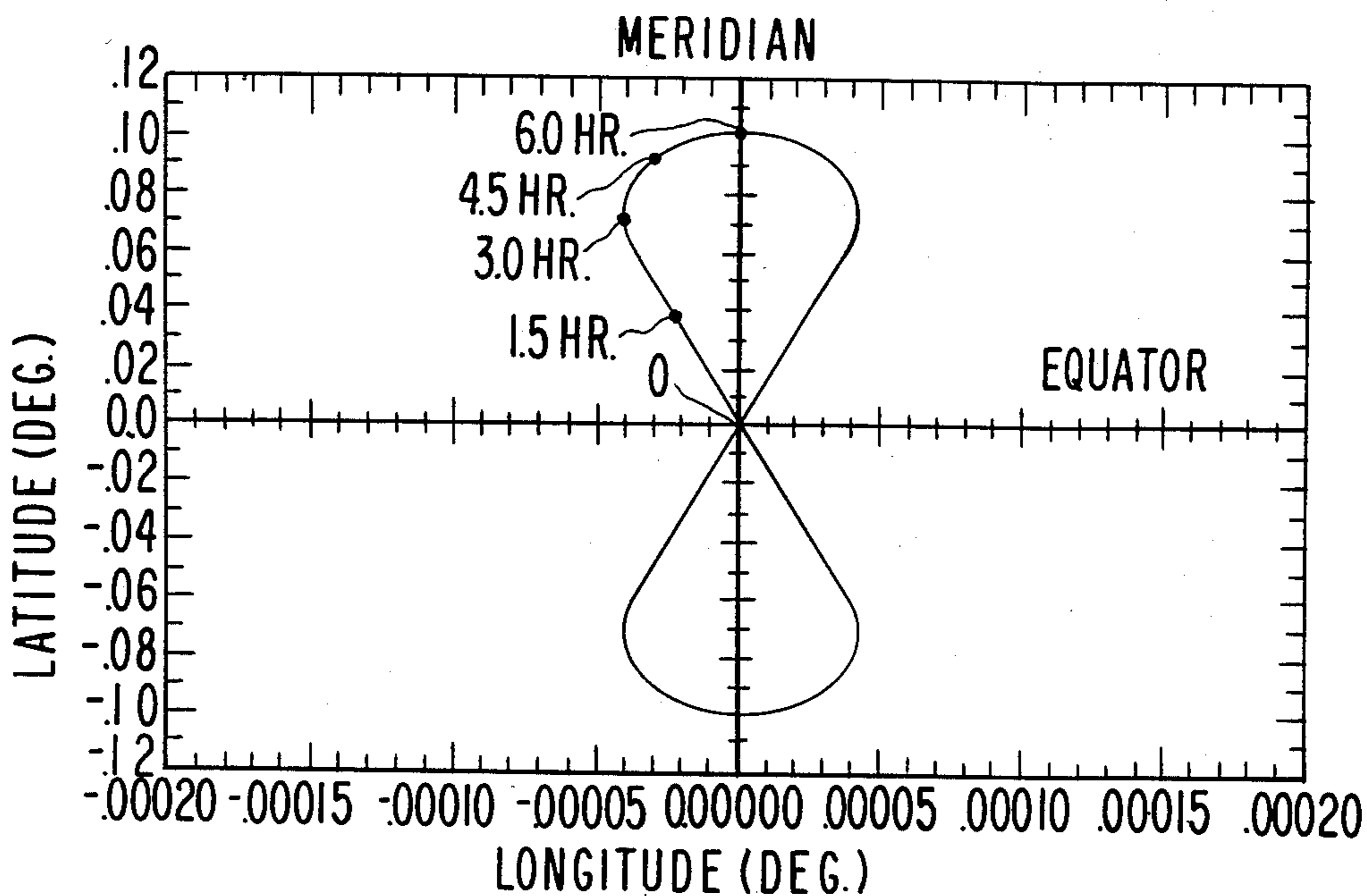
FIG. 3 SATELLITE GROUND TRACK DUE TO 0.1 DEGREE INCLINATION
