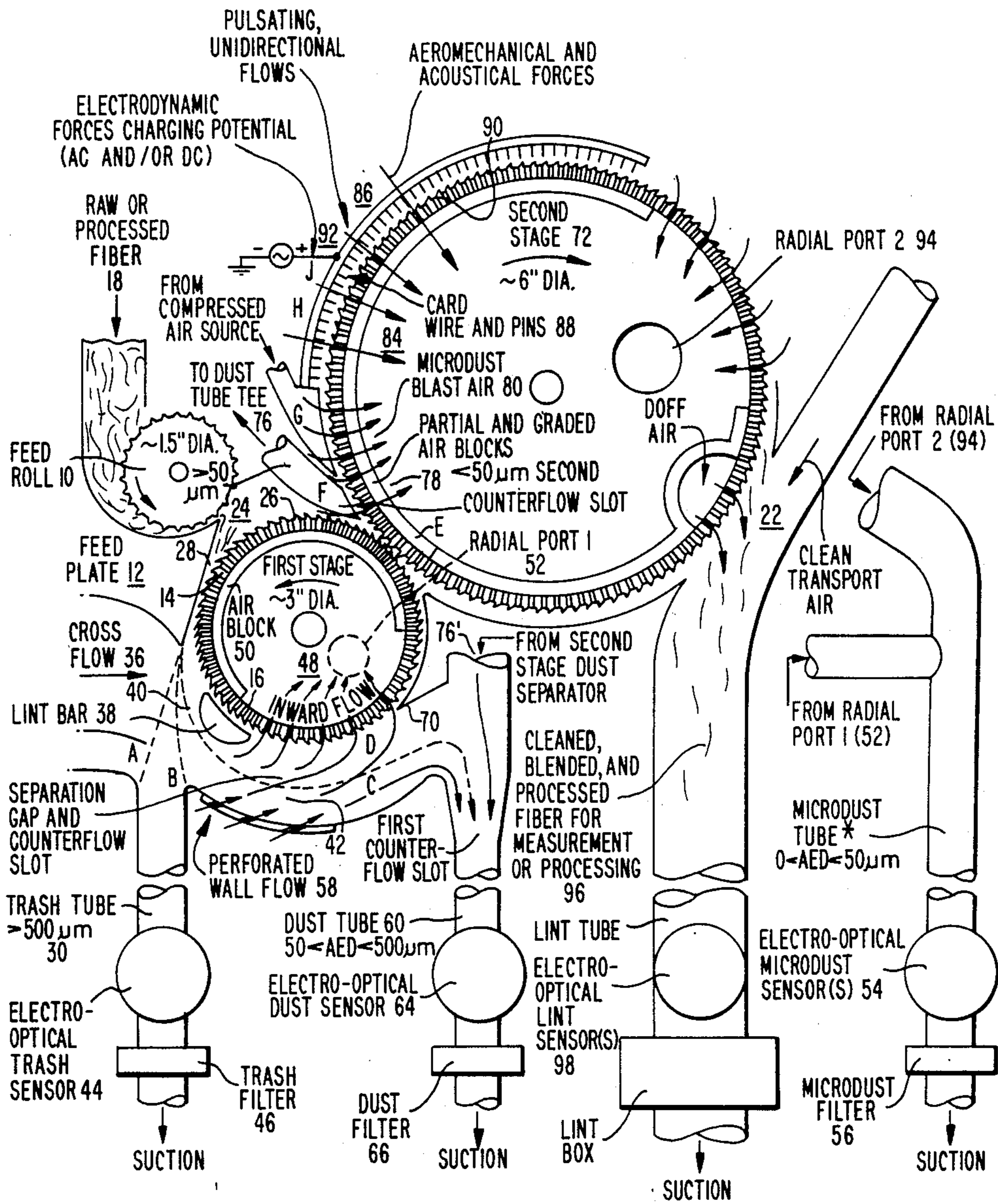
BASIC APPARATUS
