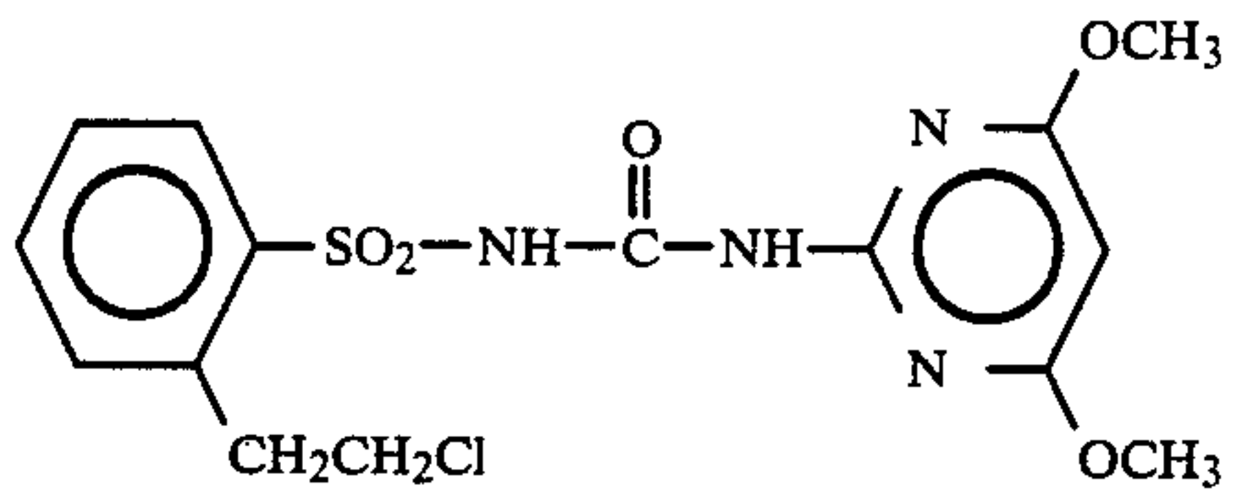
Compound 21
