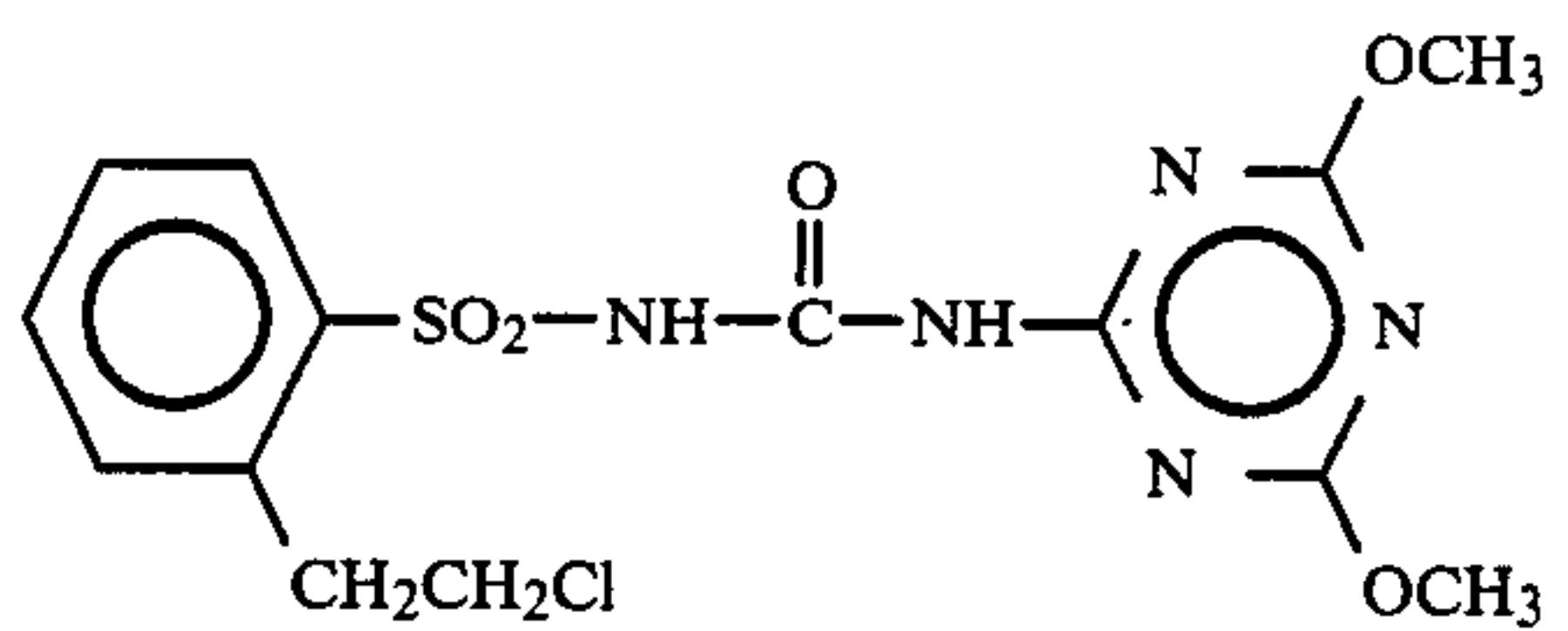
Compound 20
