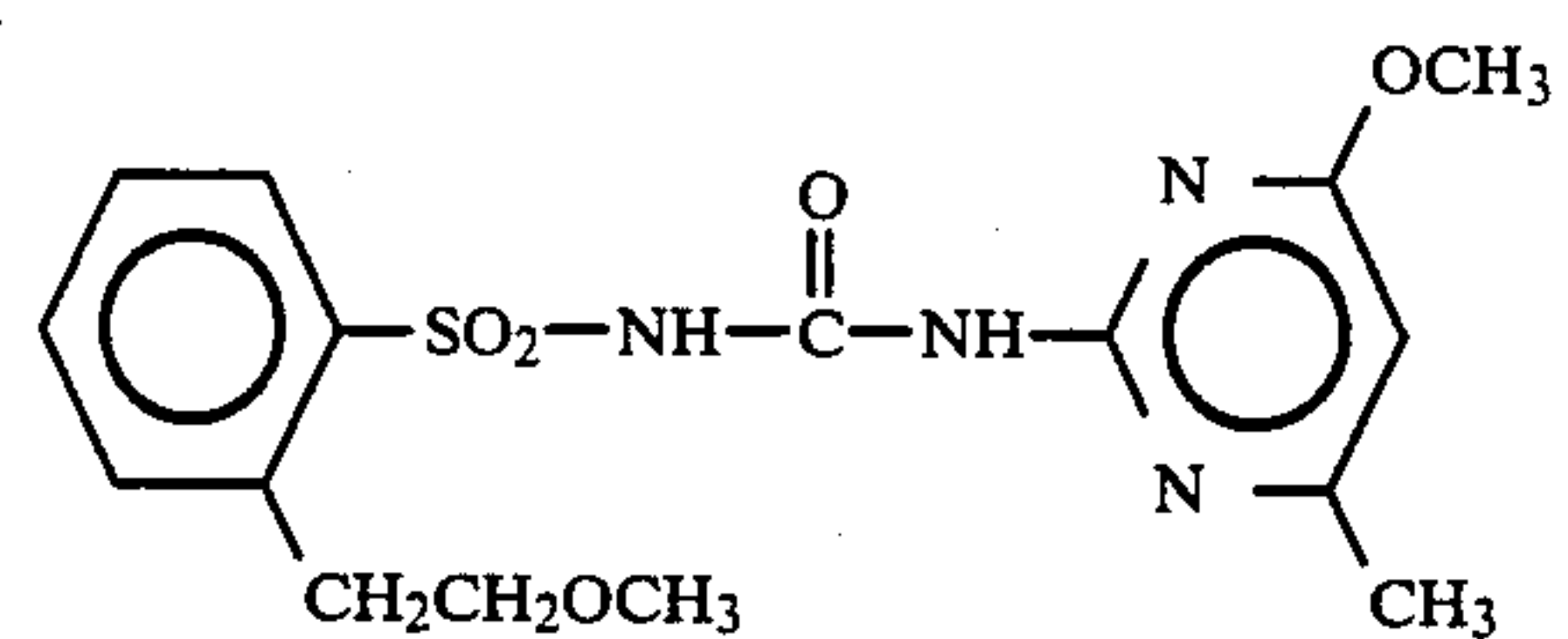
Compound 9
