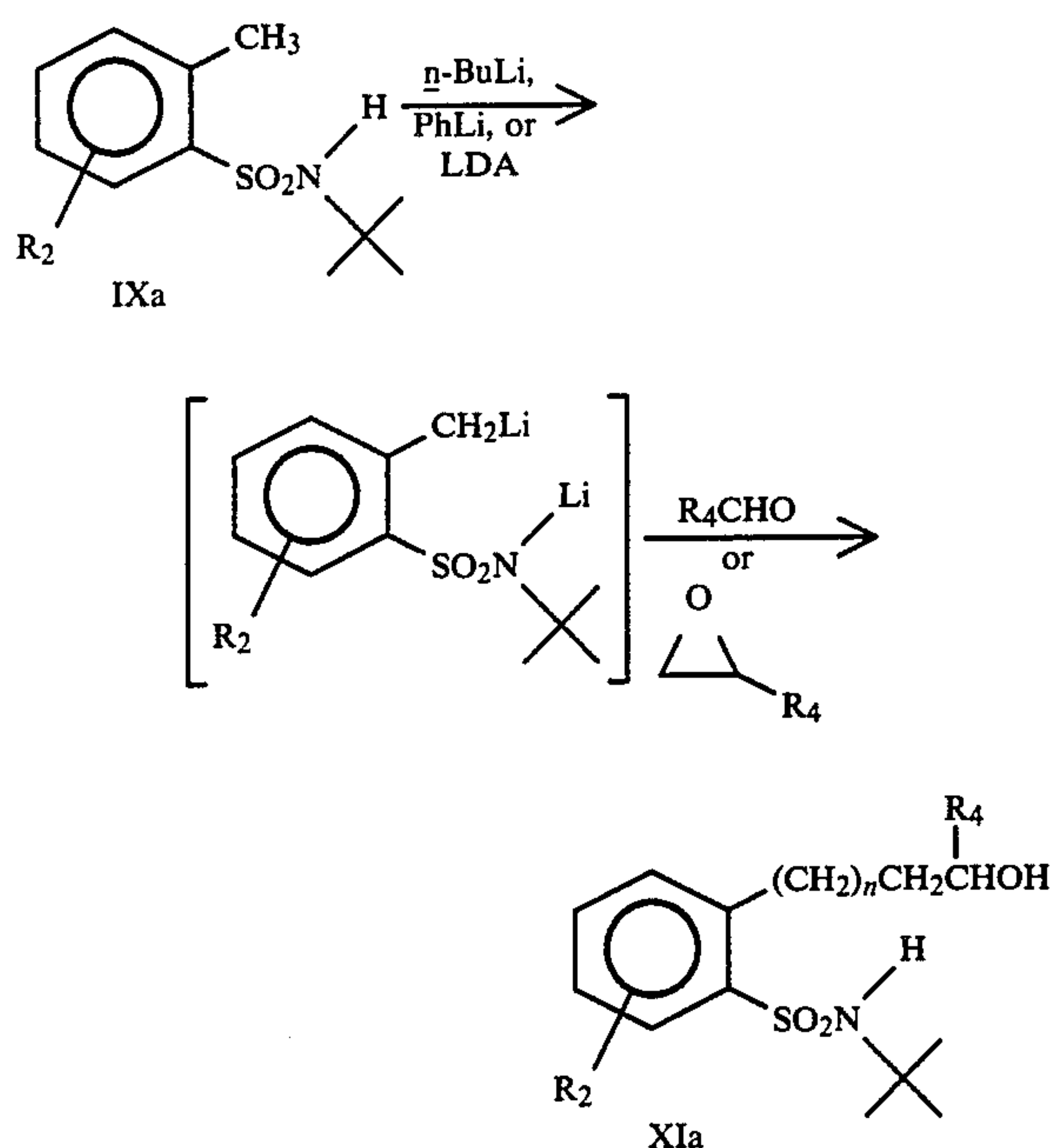
Equation 9
