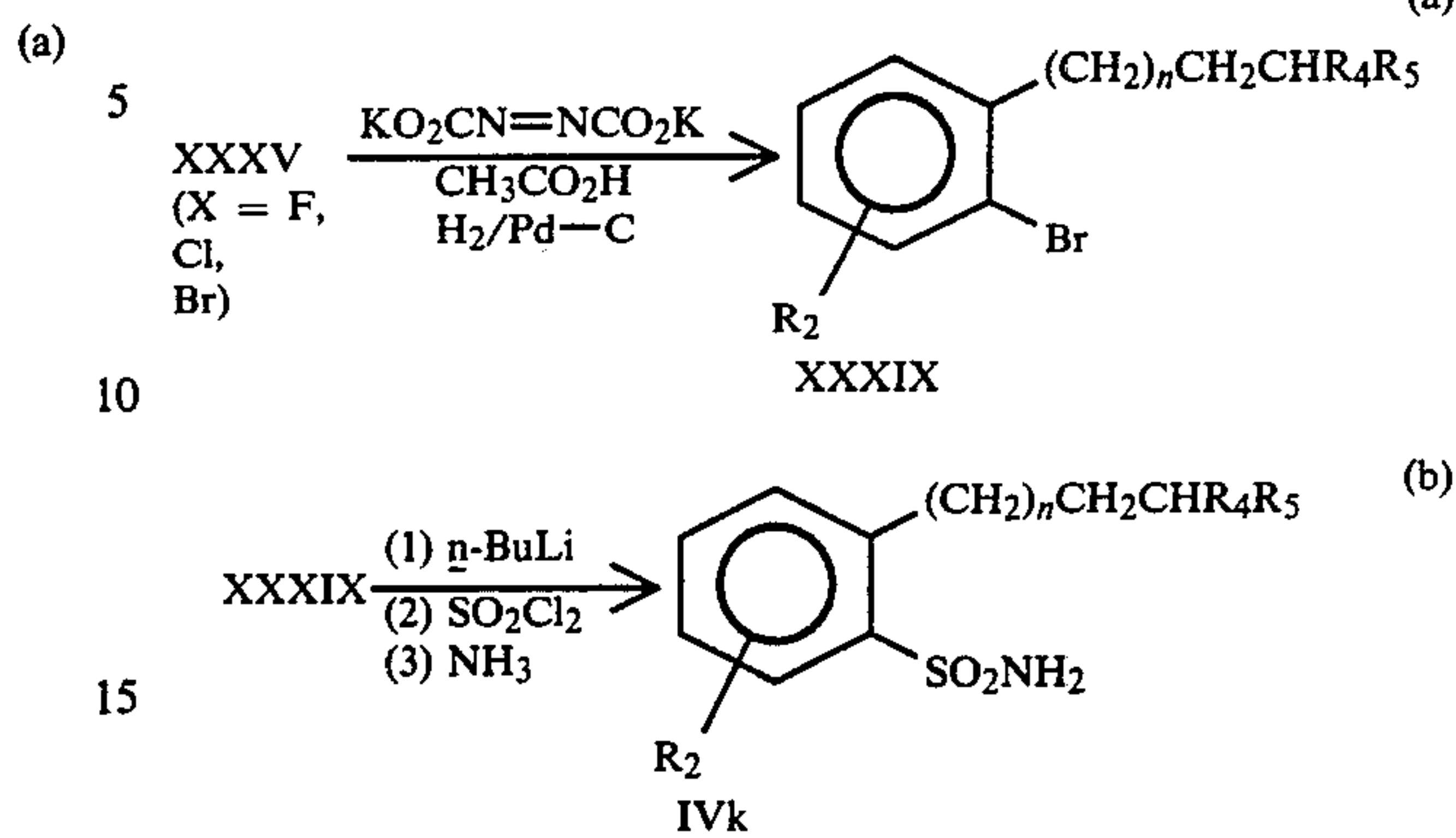
Equation 30
