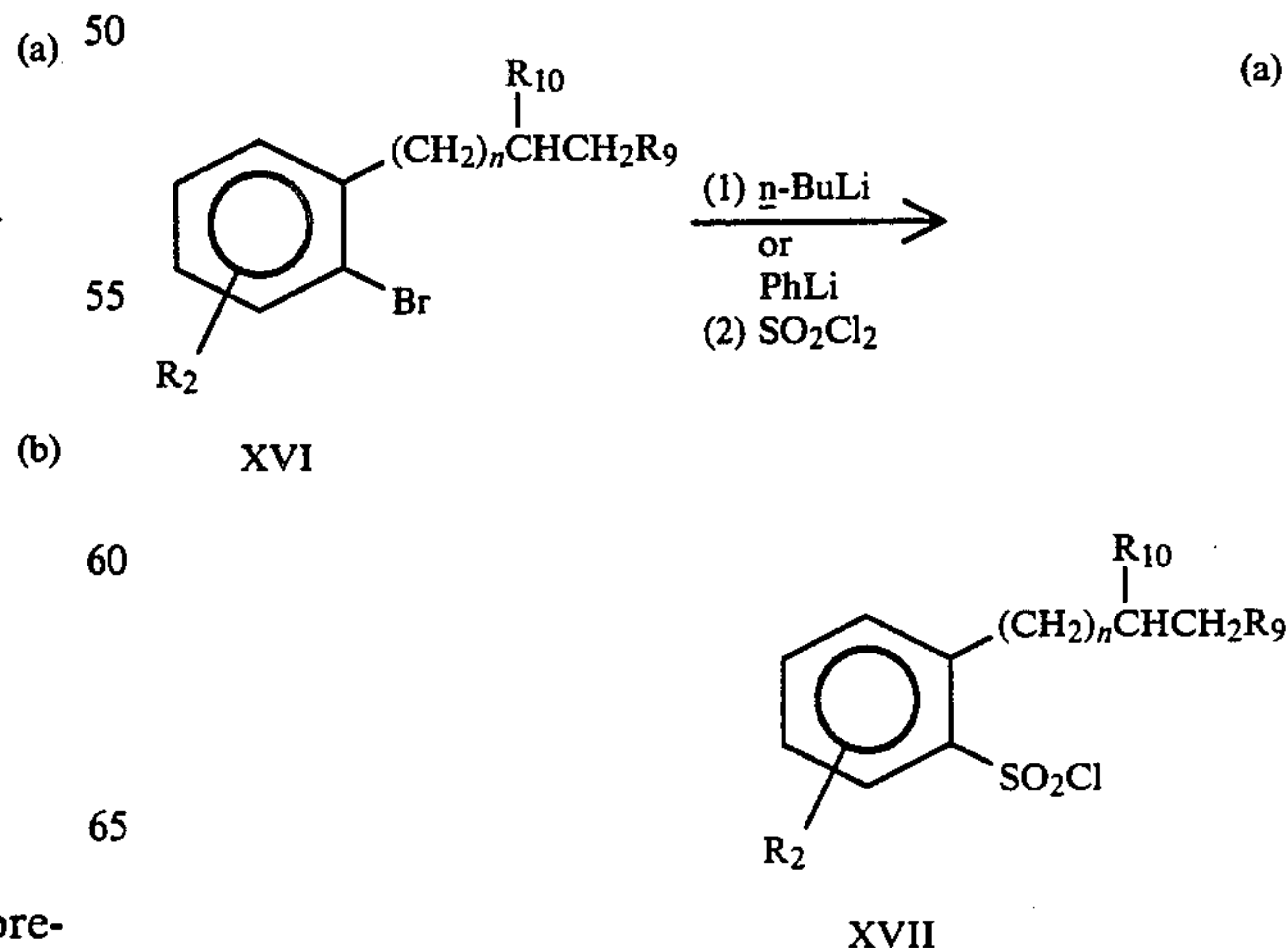
Equation 12
