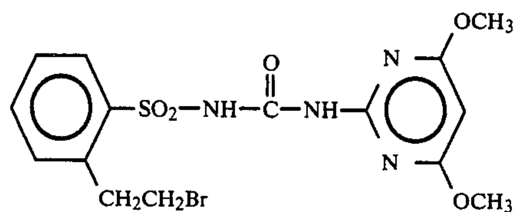
Compound 17
