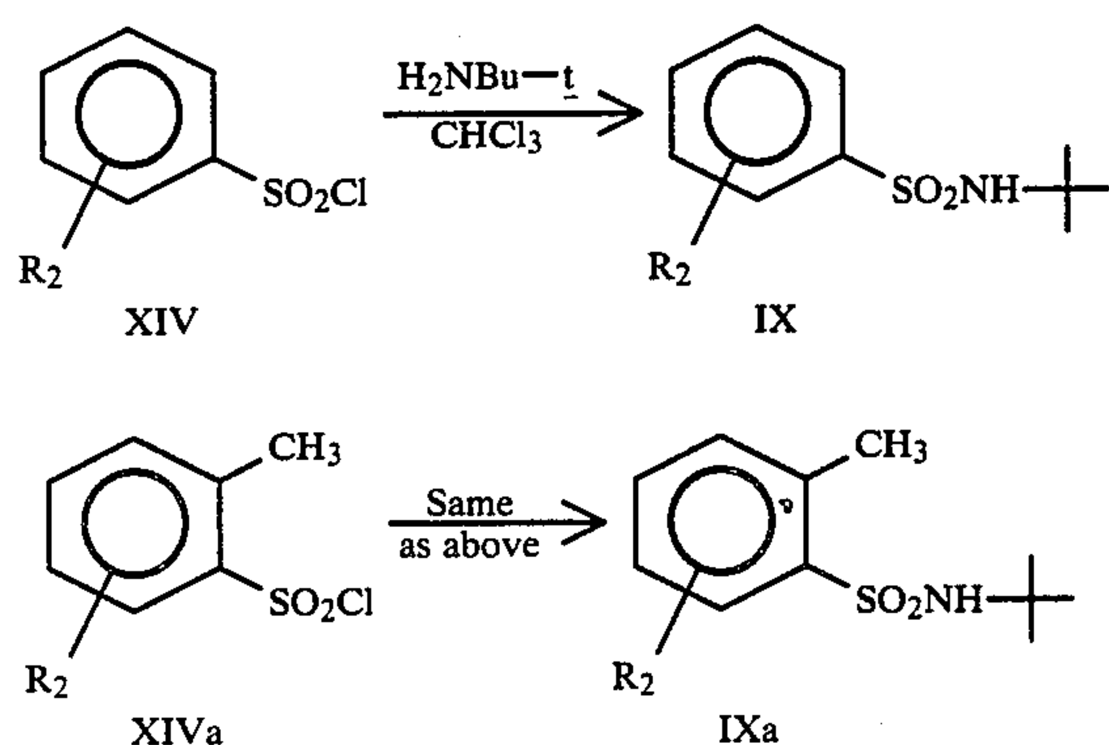
Equation 10
