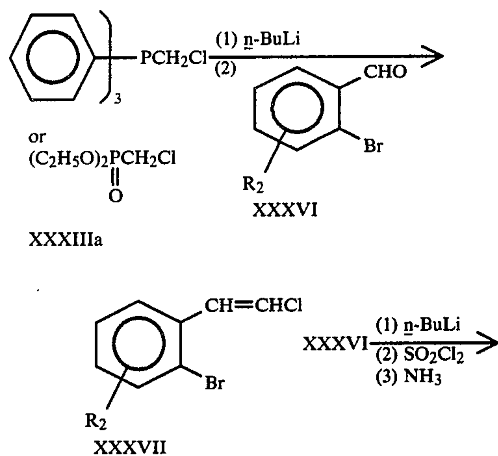
Equation 29
