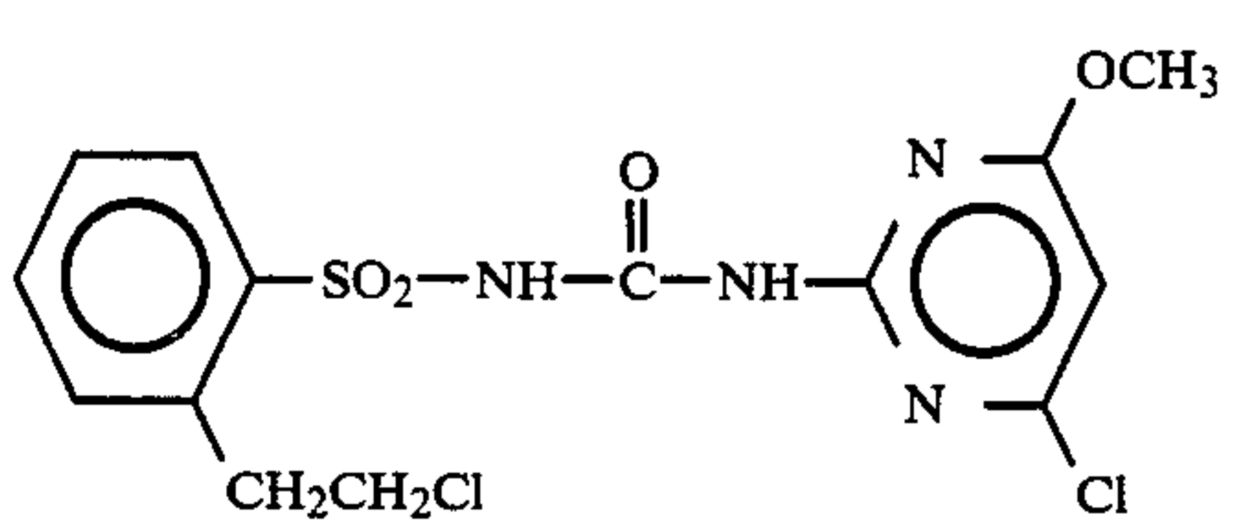
Compound 22
