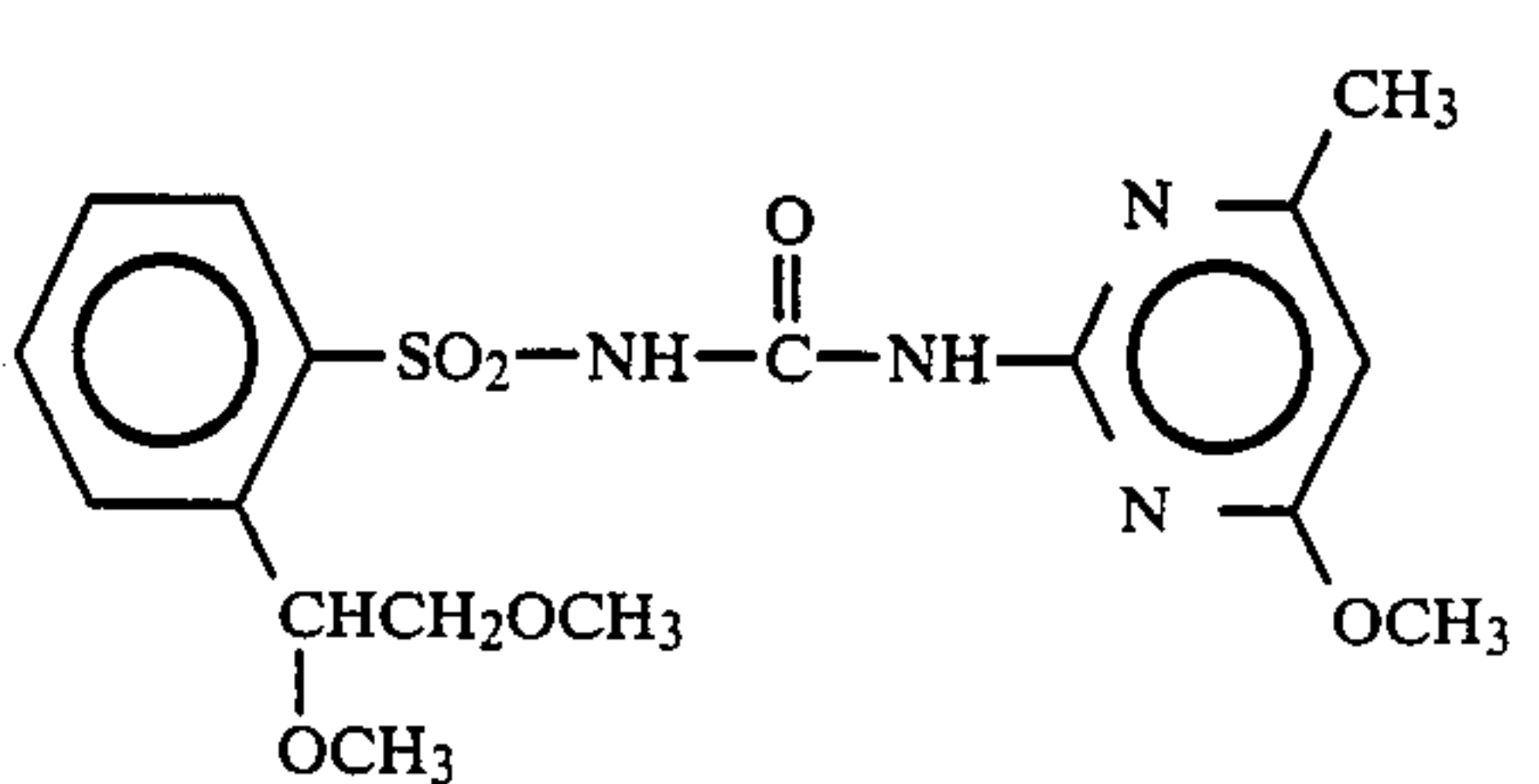
Compound 24
