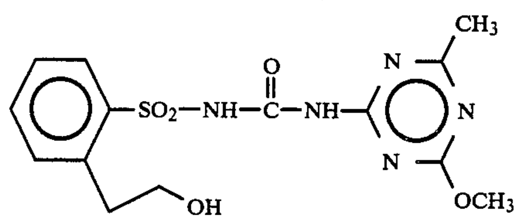
Compound 41
