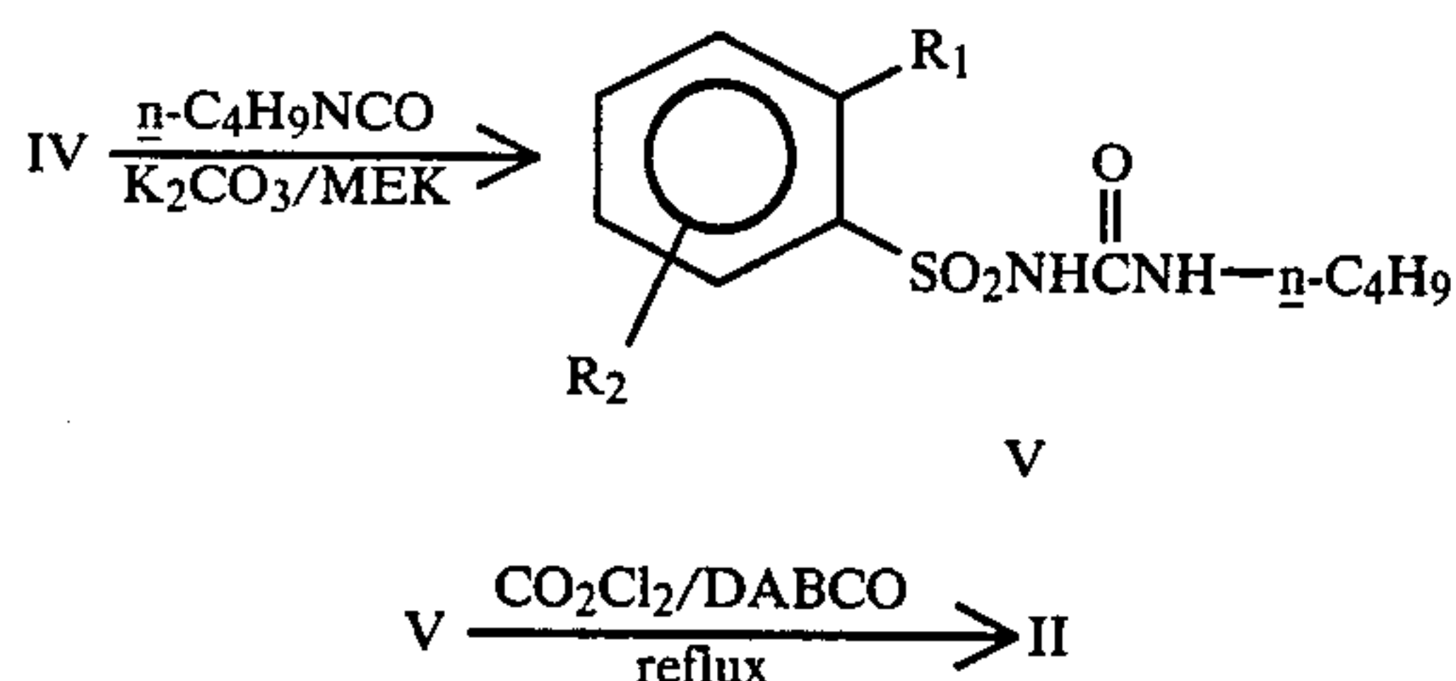
Equation 3
