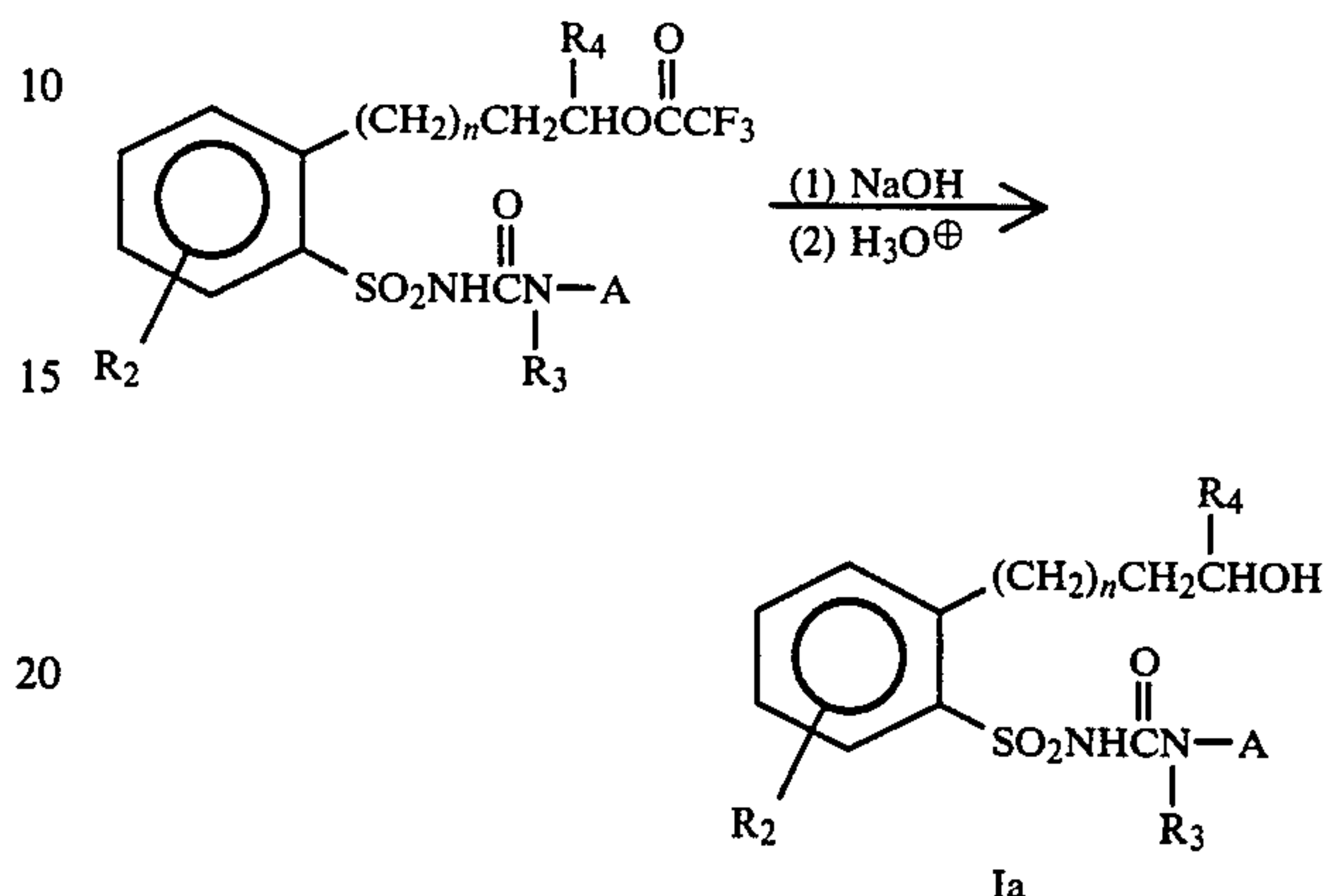
Equation 5
