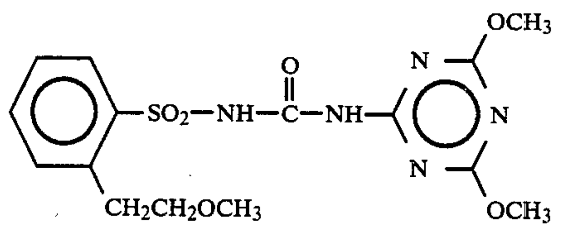
Compound 13
