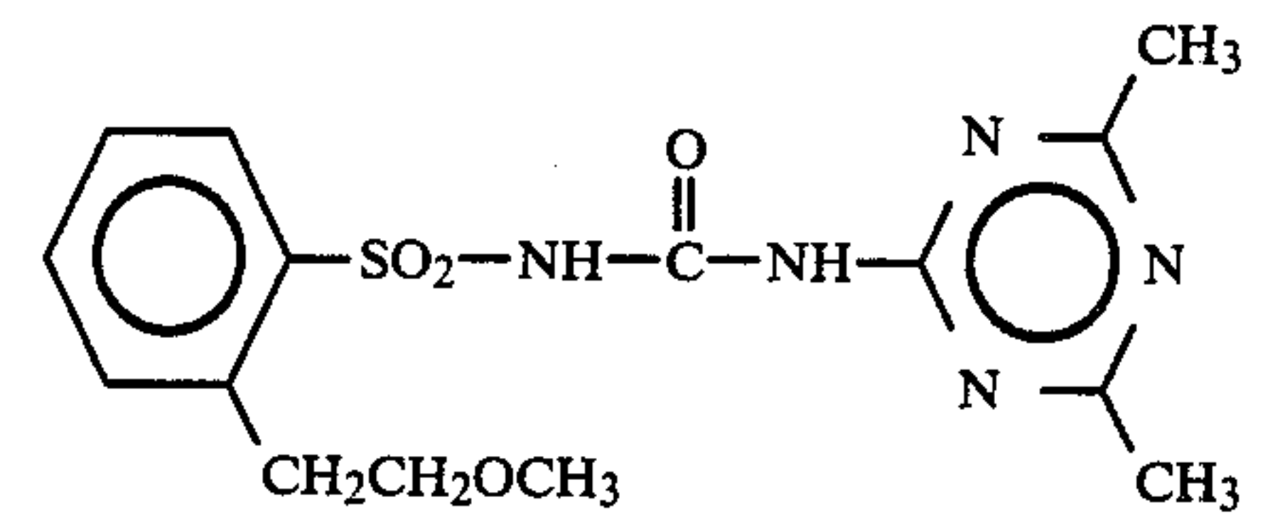
Compound 12
