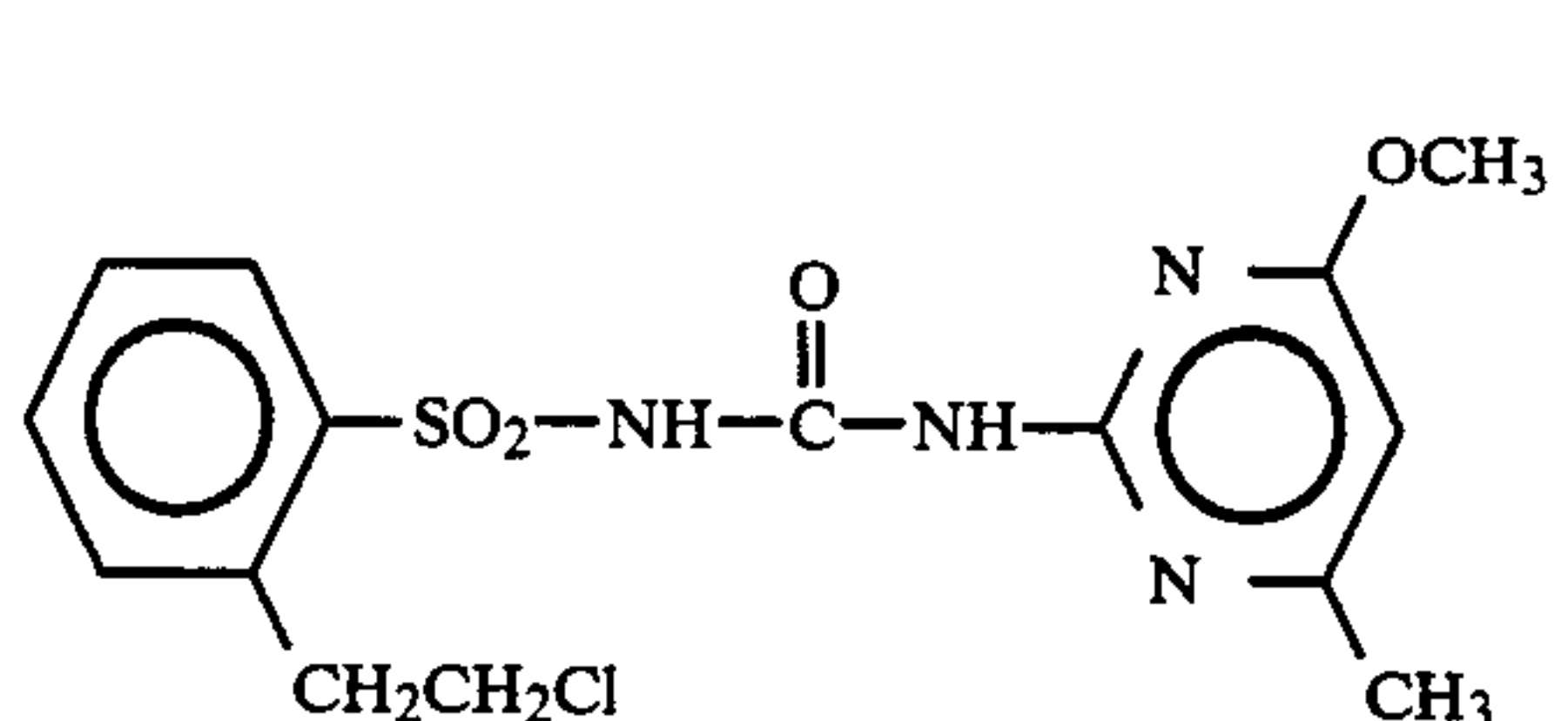
Compound 19
