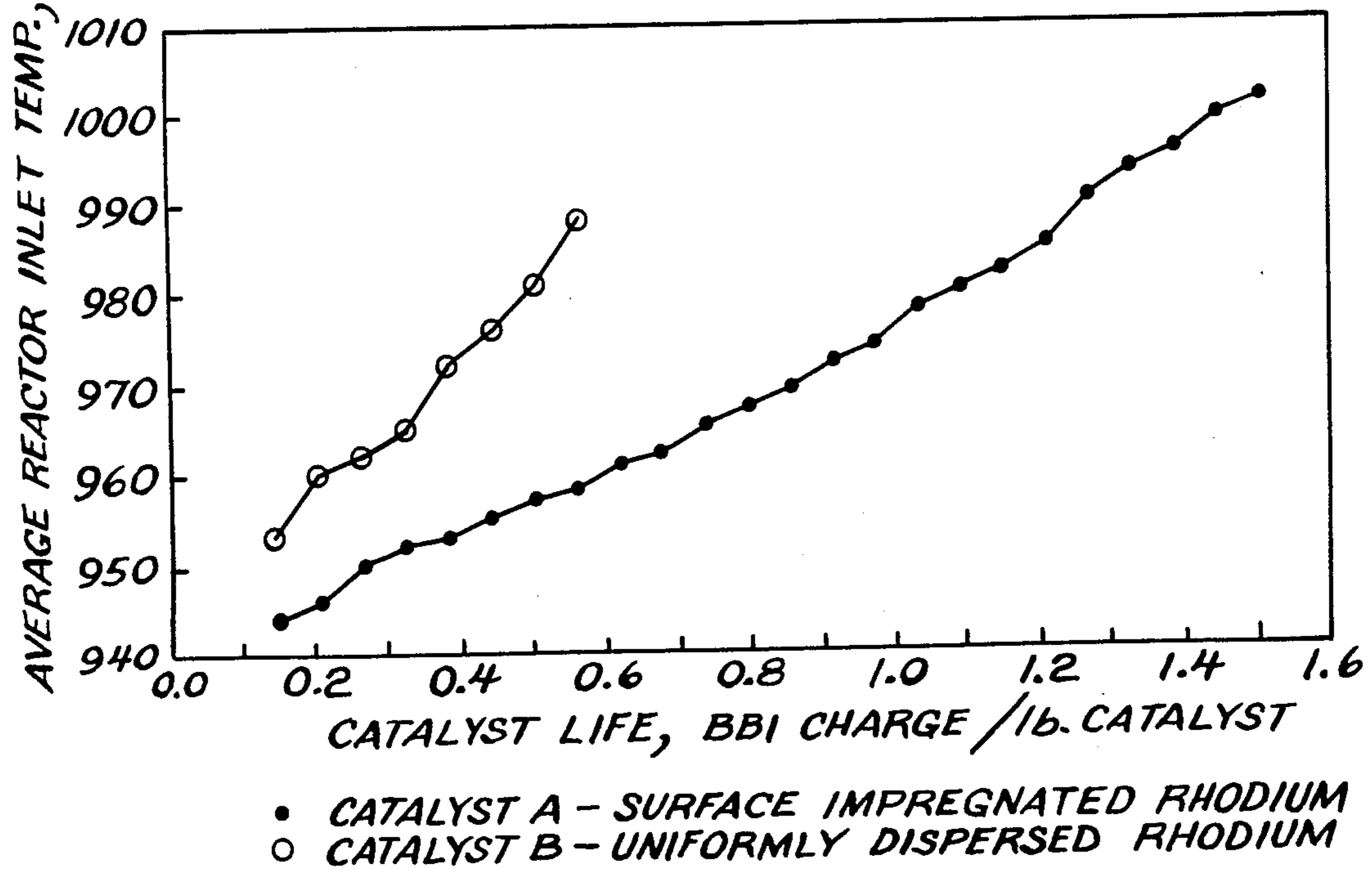
FIG. 4 AVE. REACTOR INLET TEMP. VS CATALYST LIFE
