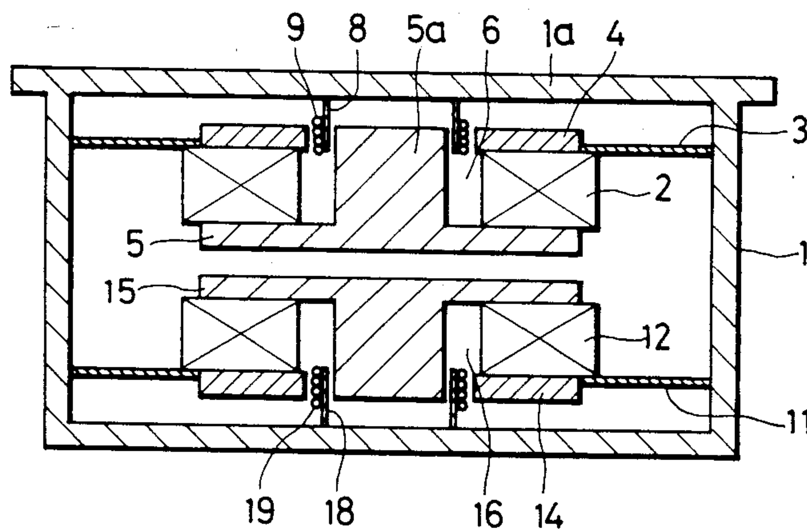
FIG. 3 PRIOR ART
