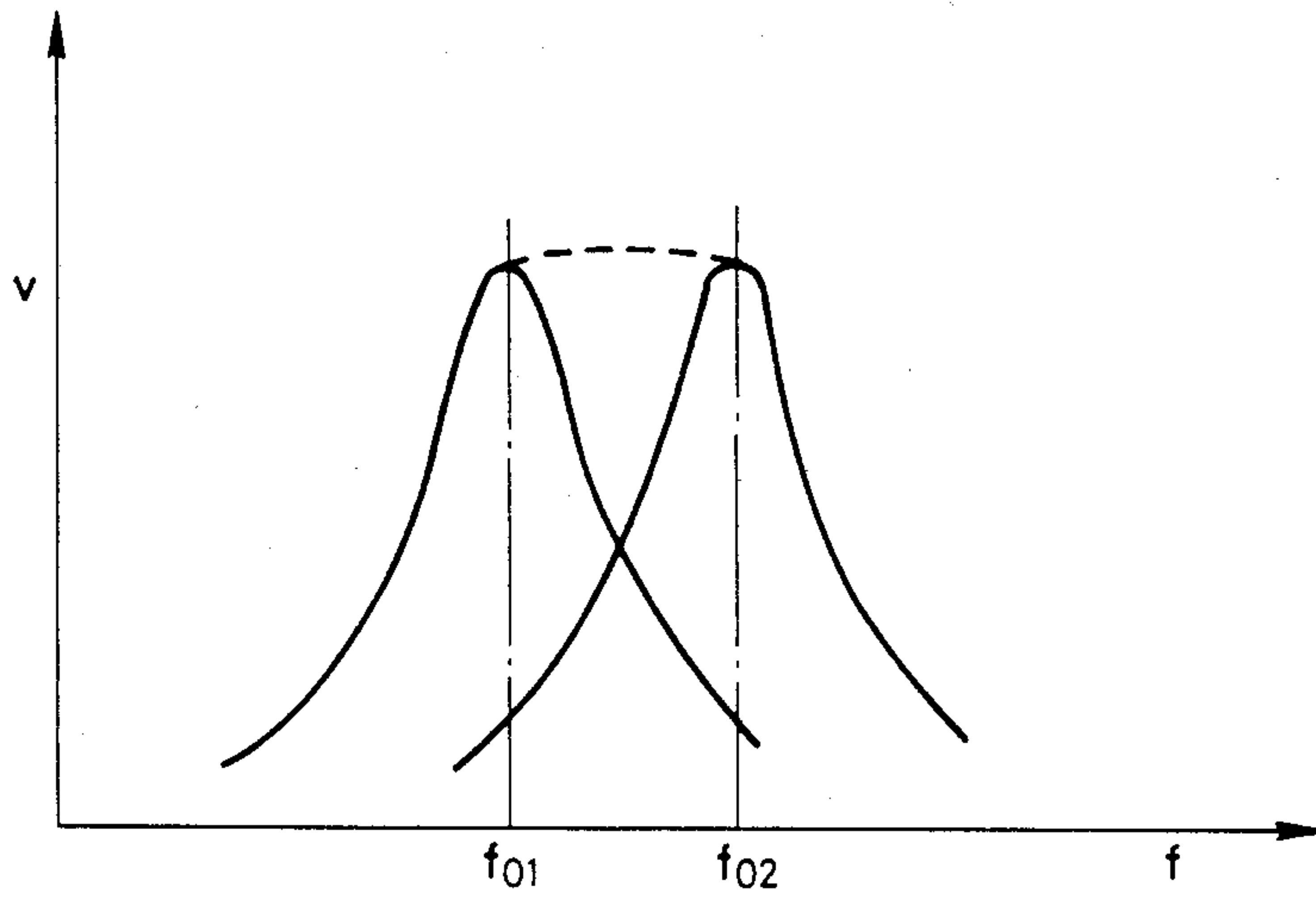
FIG. 4 PRIOR ART
