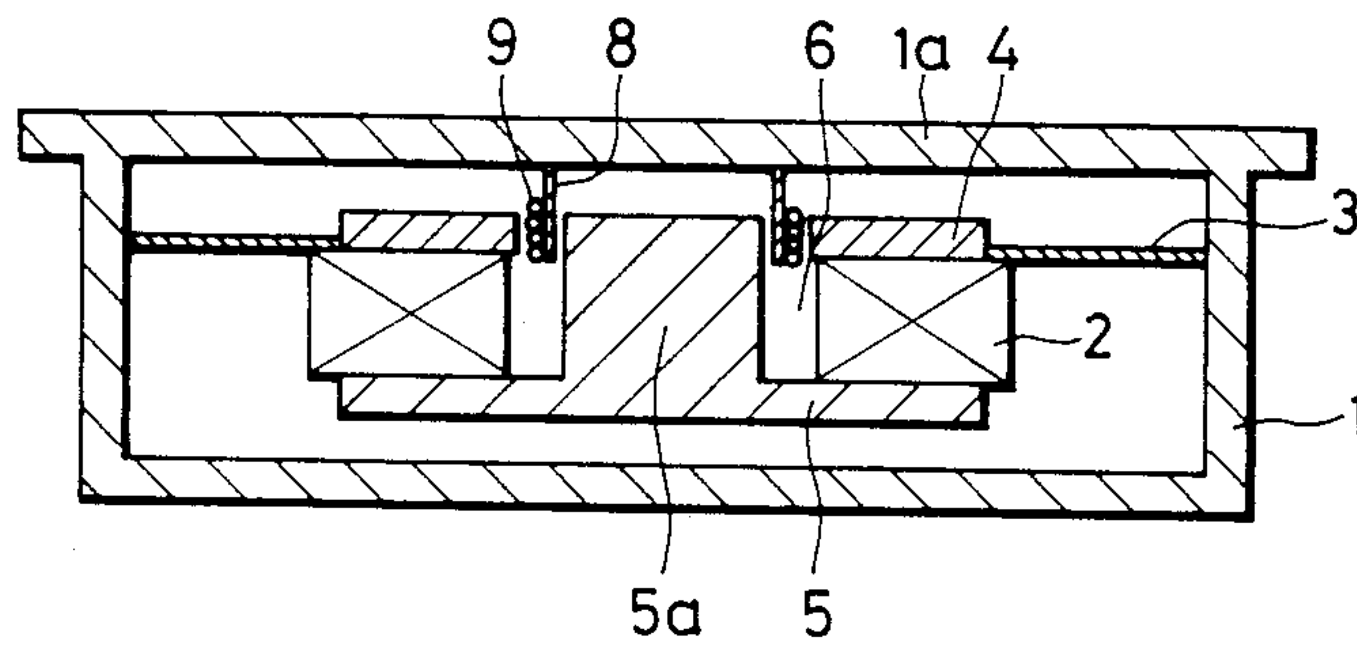
FIG. 2 PRIOR ART
