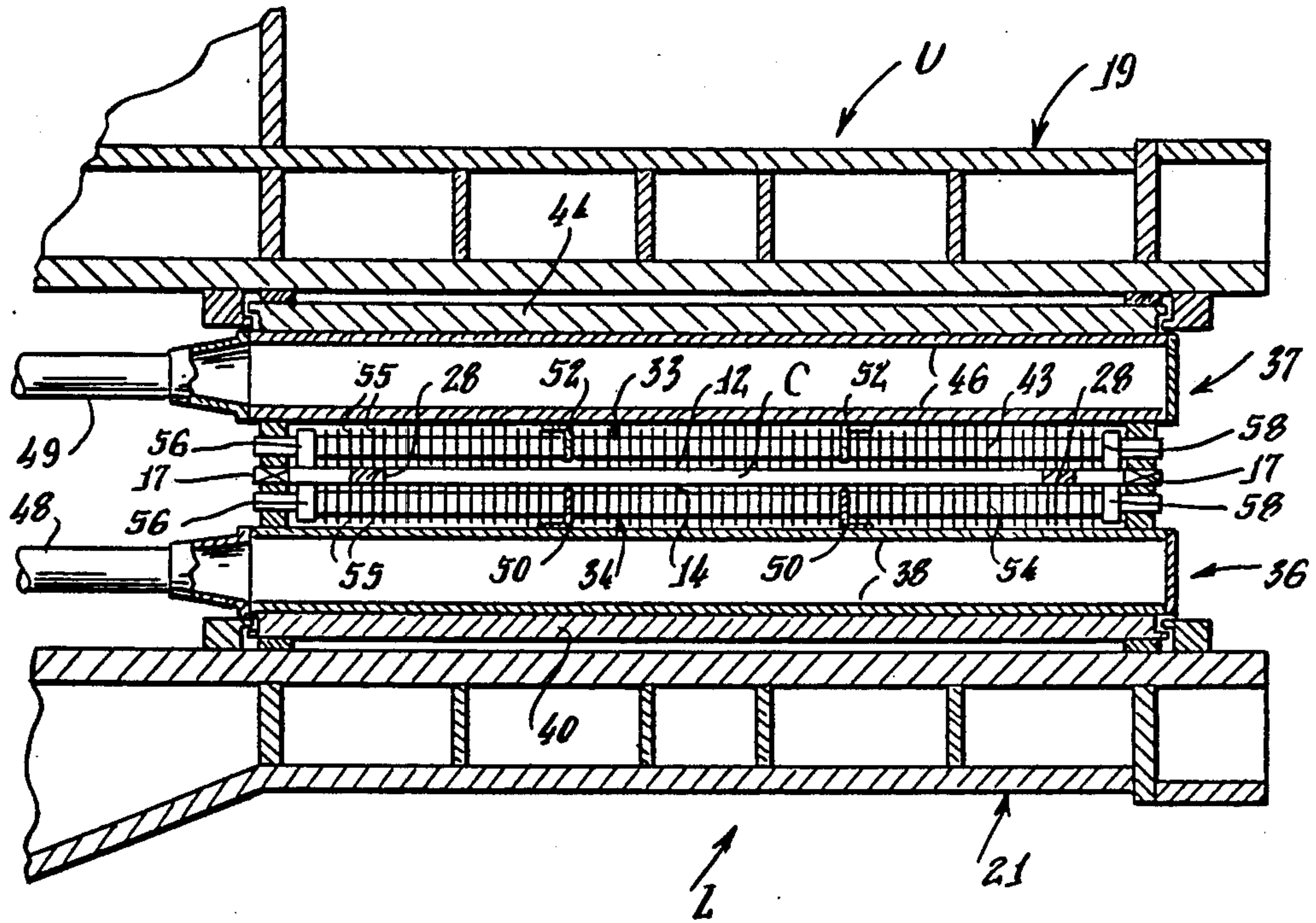
Fig. 3 (PRIOR ART)
