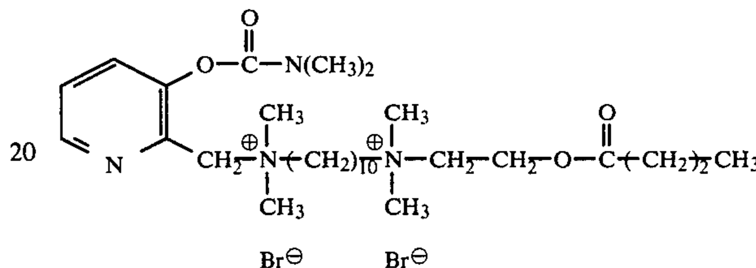
1-[N,N-dimethyl-N-(2-valeroxyethyl)ammonio]-10-[N-(3-dimethylcarbamoxy- \alpha -picolinyl)-N,N-dimethylammonio]decane dibromide.
