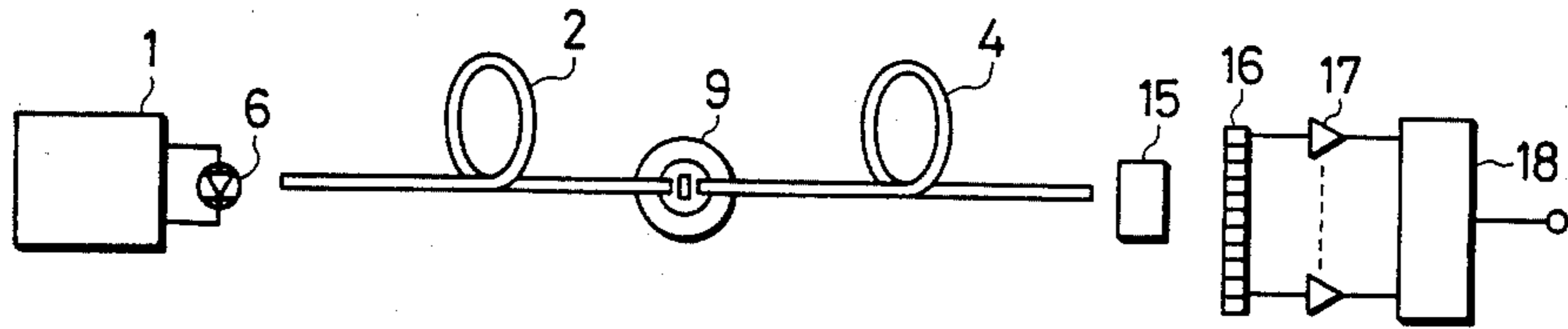
FIG. 1 PRIOR ART
