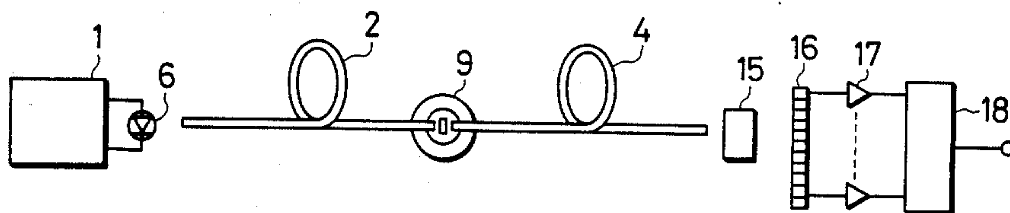
FIG. 1 PRIOR ART
