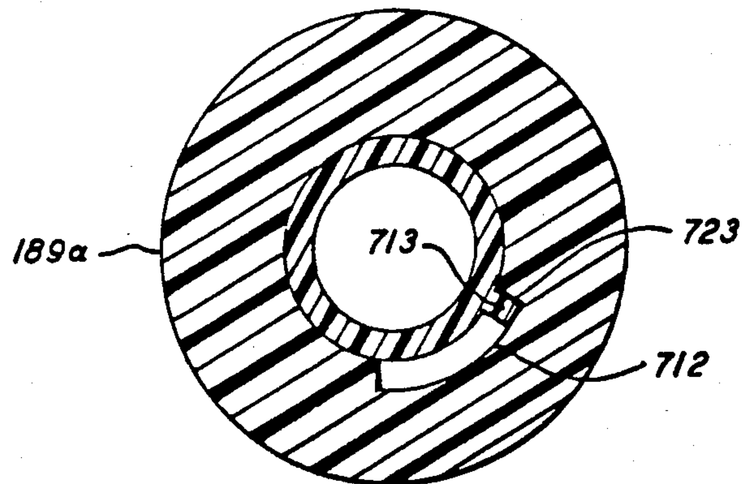
DISPENSING FIG. 29c
