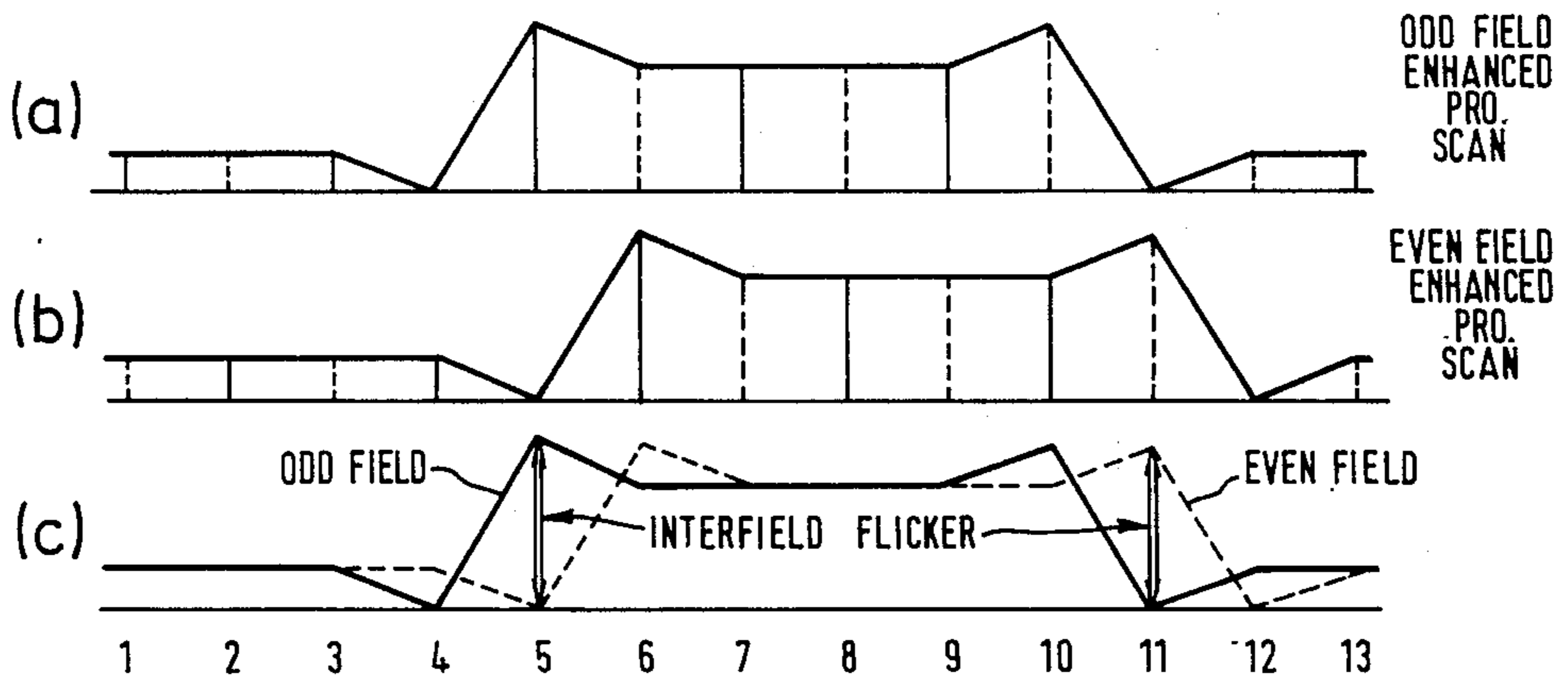
FIG. 4 PRIOR ART
