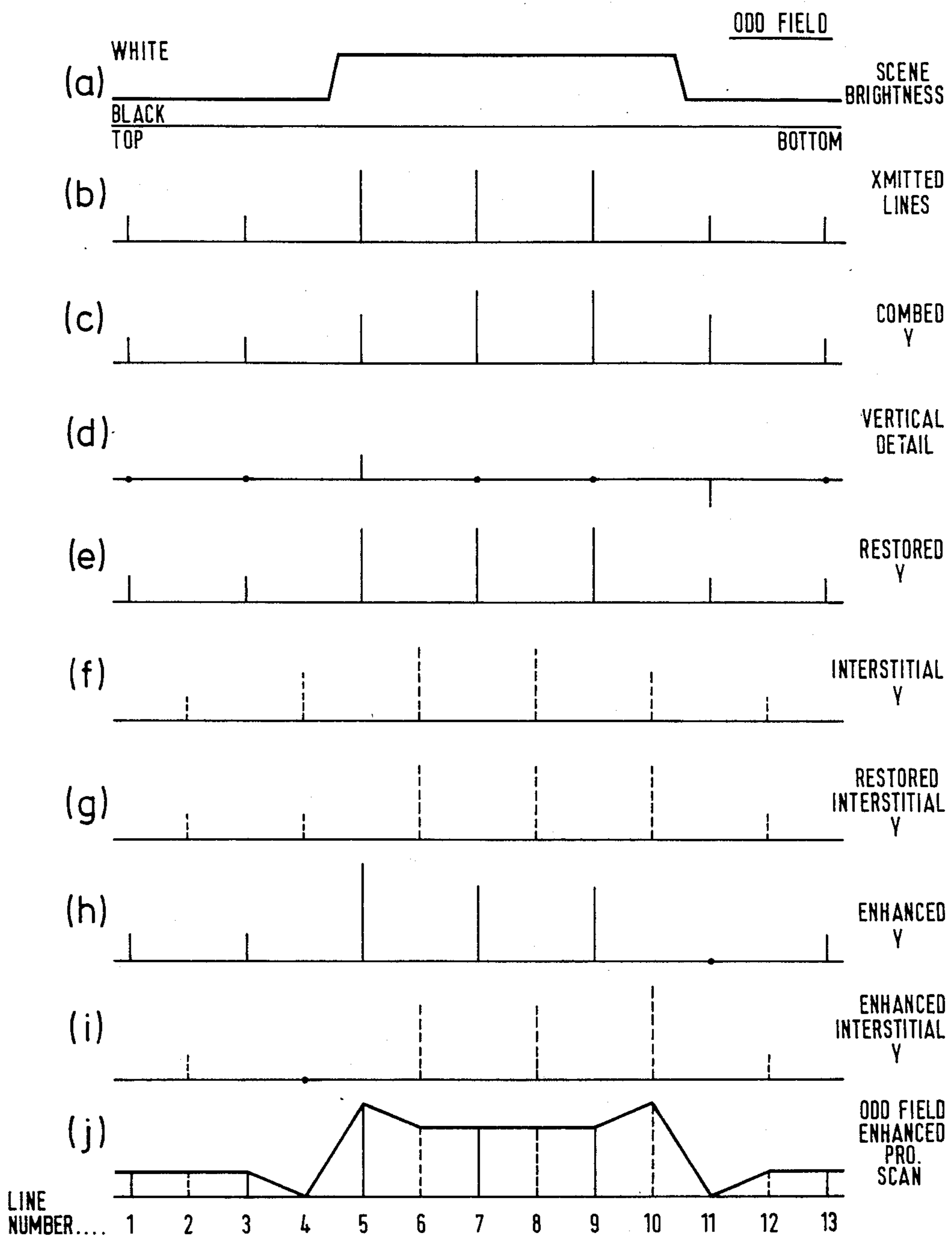
FIG. 3 PRIOR ART
