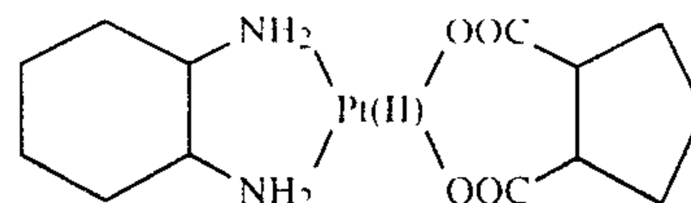
(trans-1,2-cyclopentanedicarboxylato)
