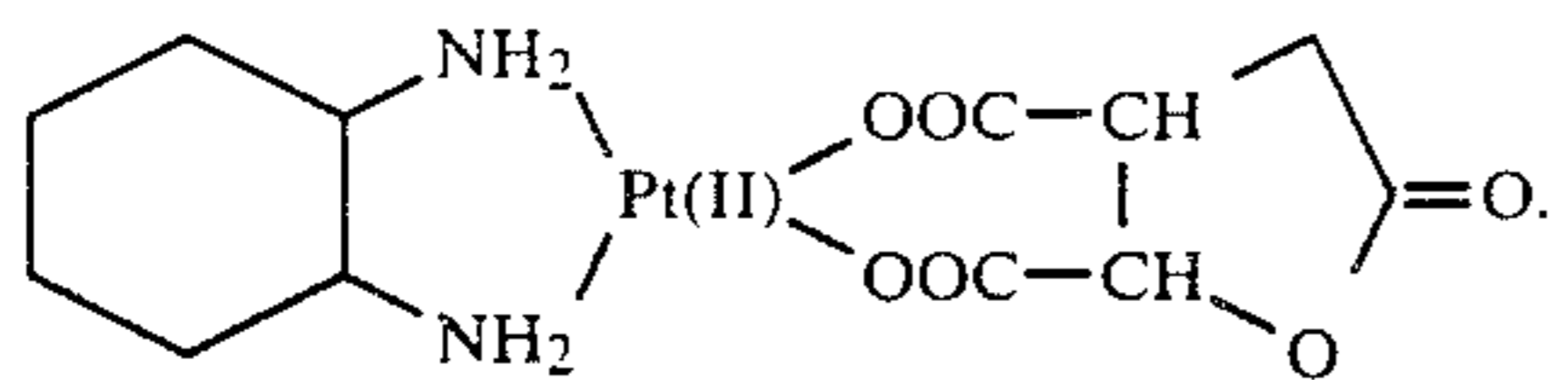
[isocitratolactone]
