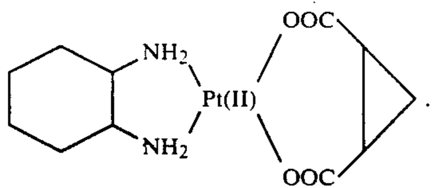
(1,2-cyclopropanedicarboxylato)
