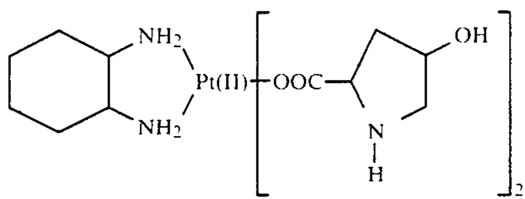
[bis-hydroxyprolinato]
