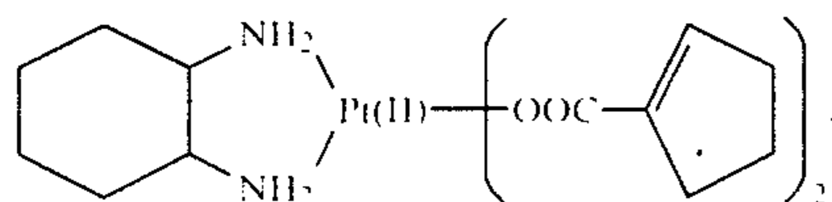
(bis-cyclopentenecarboxylato)
