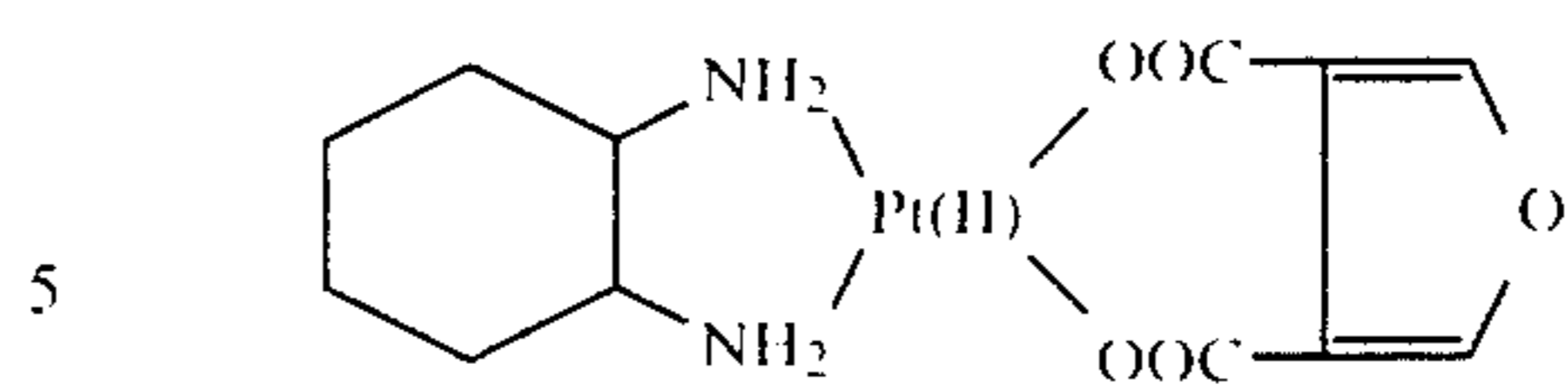
[furanedicarboxylate]
