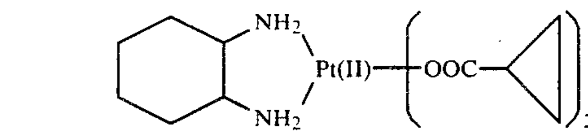
(bis-cyclopropanecarboxylato)
