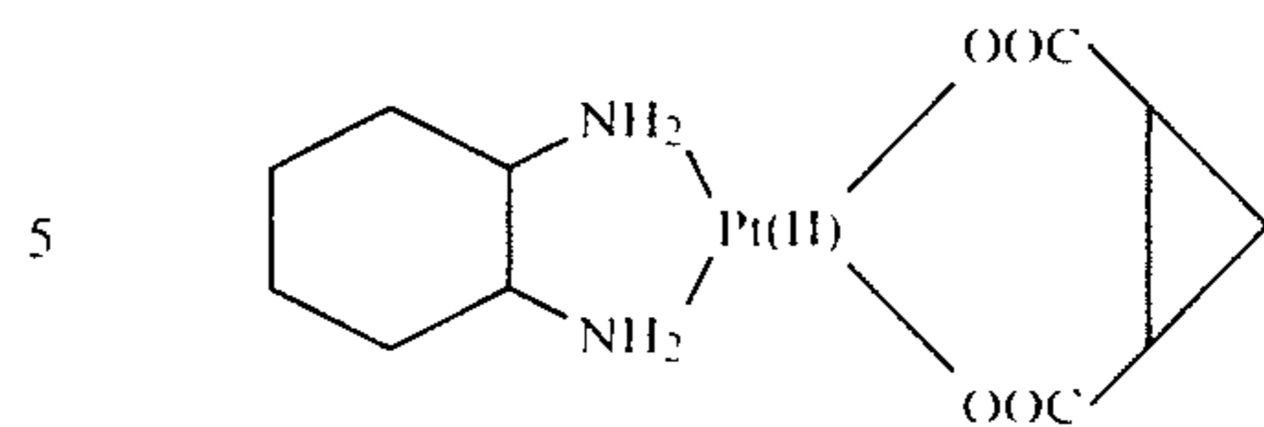
(1,2-cyclopropanedicarboxylato)
