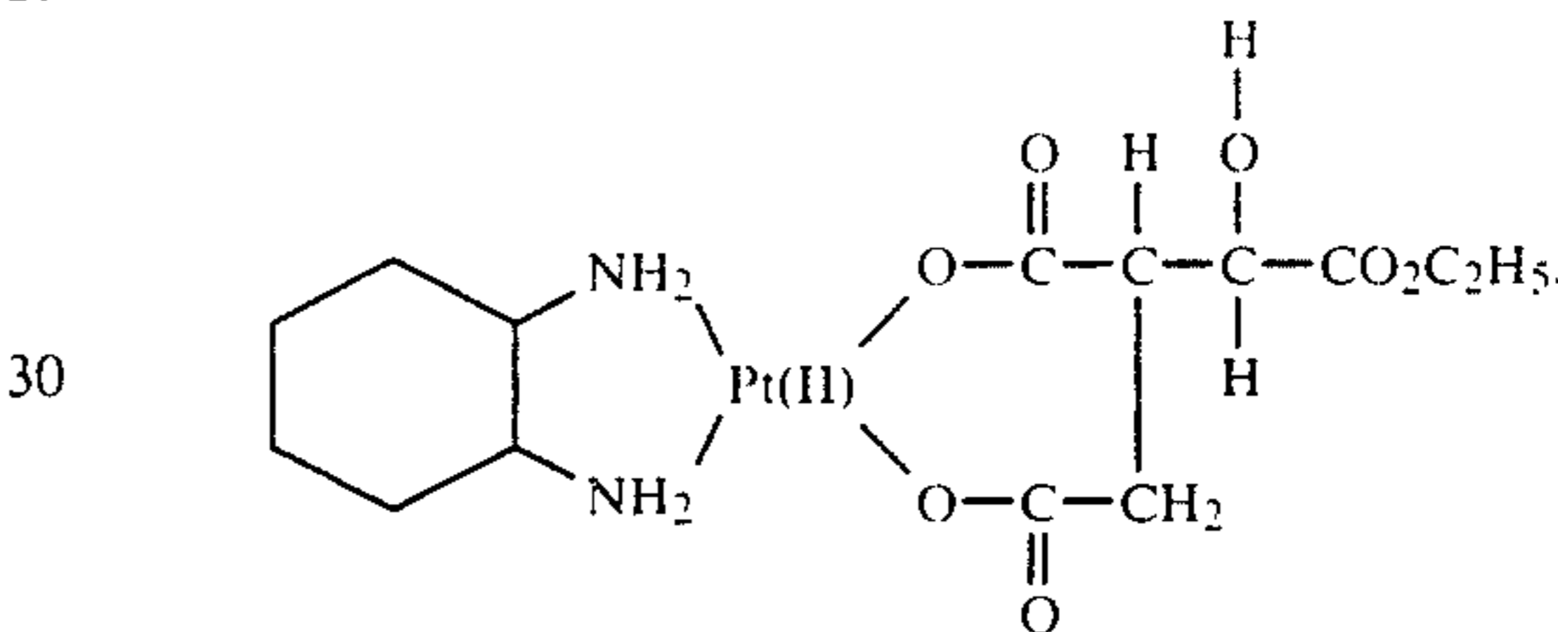
[isocitratomonoethylester]
