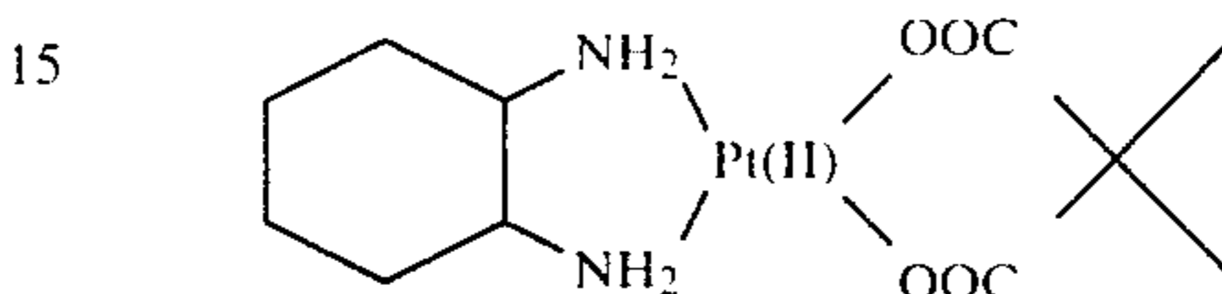
[cyclopropanedicarboxylato-]
