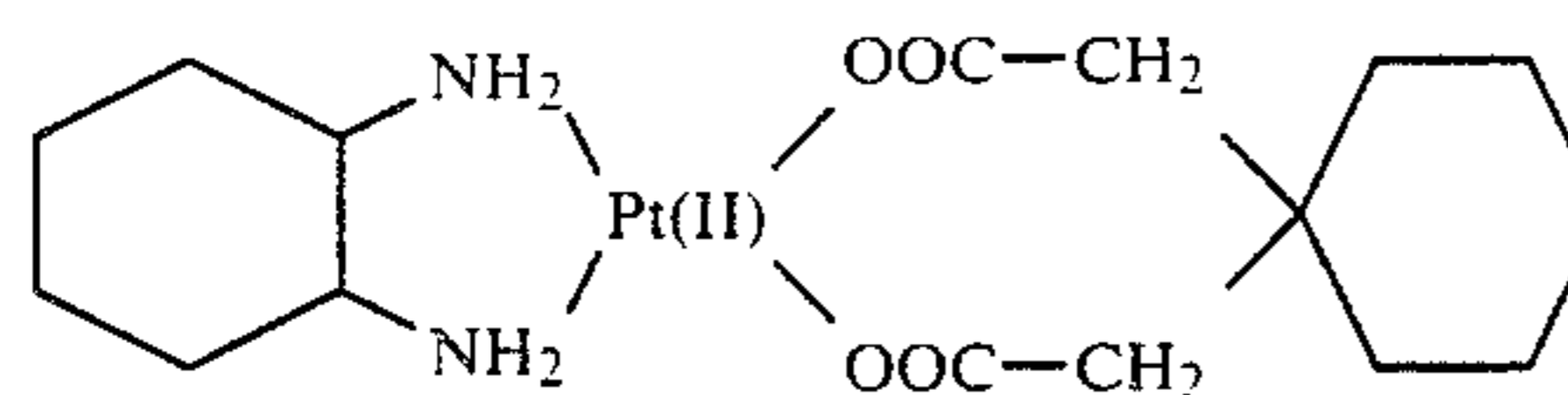
(cyclohexane-1,1-diacetato)
