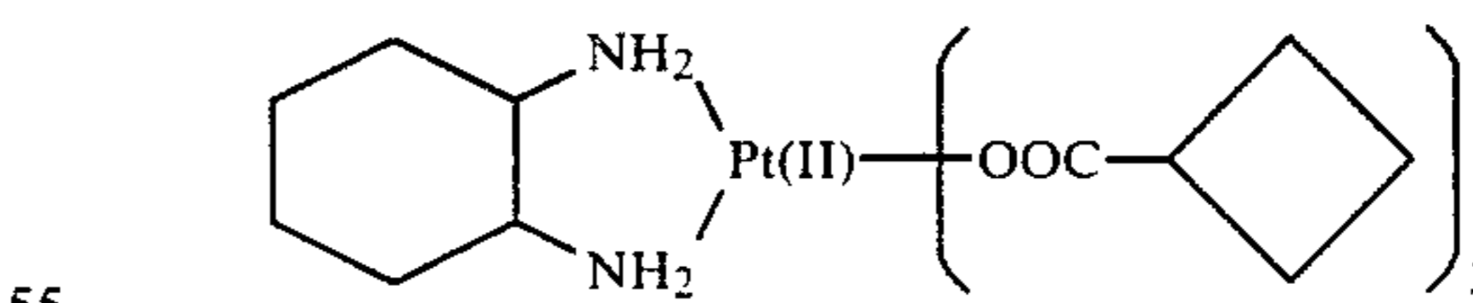
(bis-cyclobutanecarboxylato)
