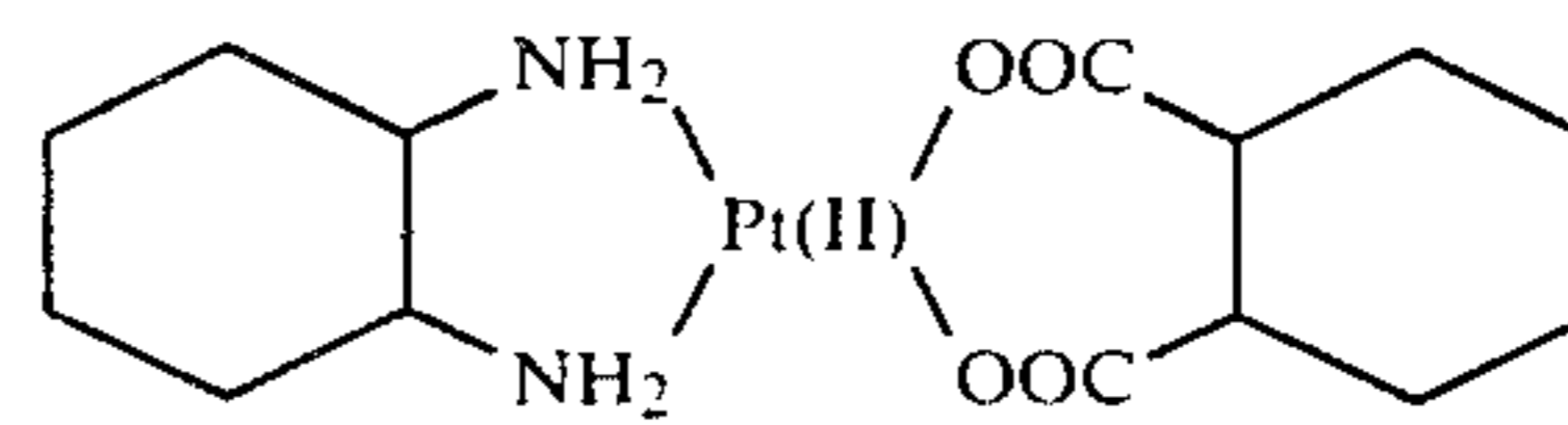
(trans-1,2-cyclohexanedicarboxylato)
