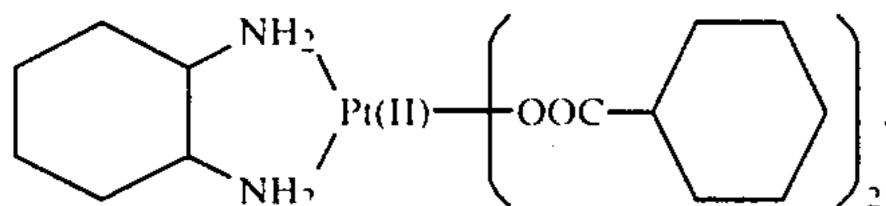
(bis-cyclohexanecarboxylato)
