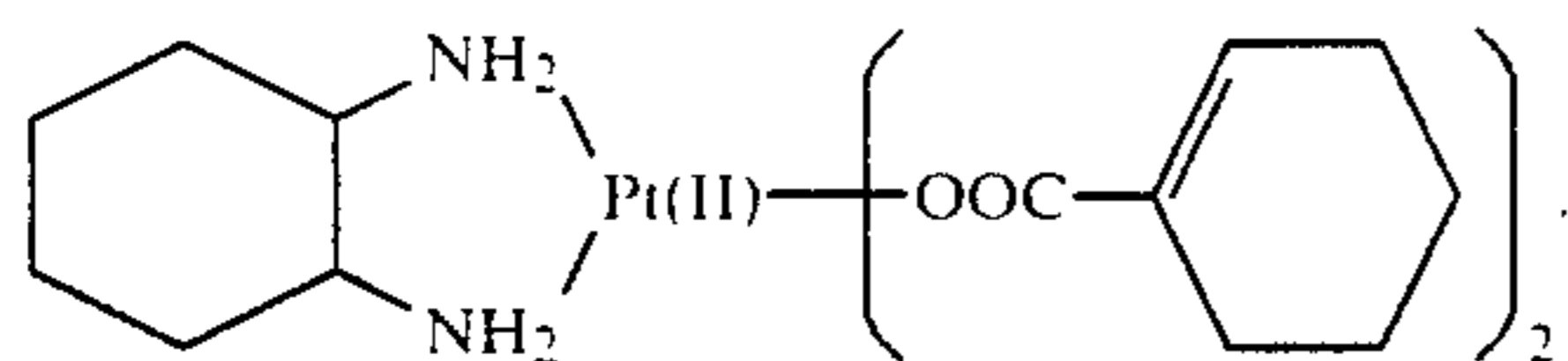
(bis-cyclohexenecarboxylato)
