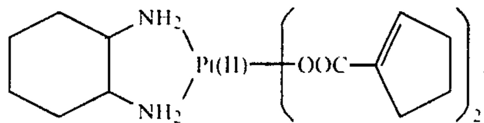
(bis-cyclopentenecarboxylato)
