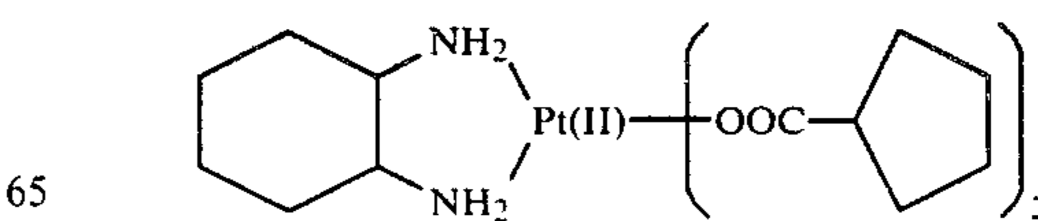
(bis-cyclopentanecarboxylato)
