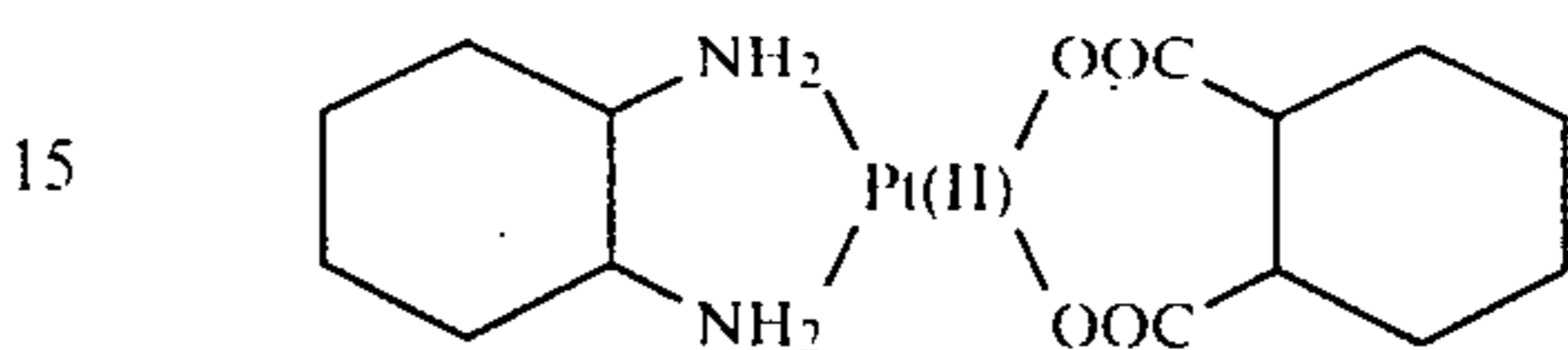
(trans-1,2-cyclohexanedicarboxylato)
