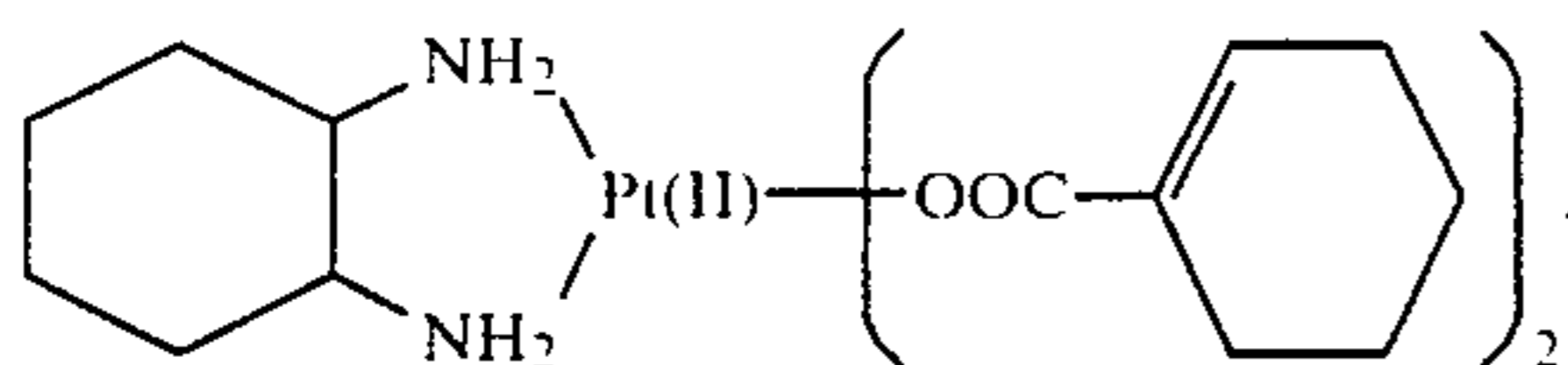
(bis-cyclohexenecarboxylato)
