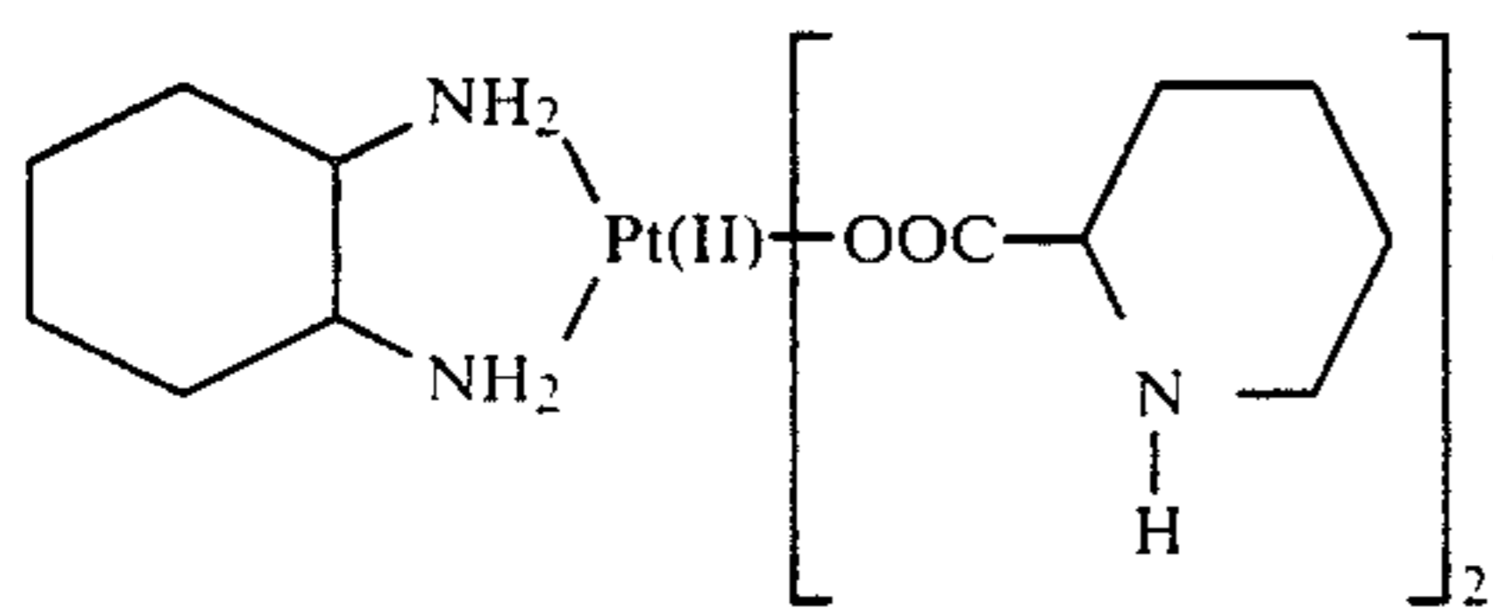
[bis-pipecolinato]
