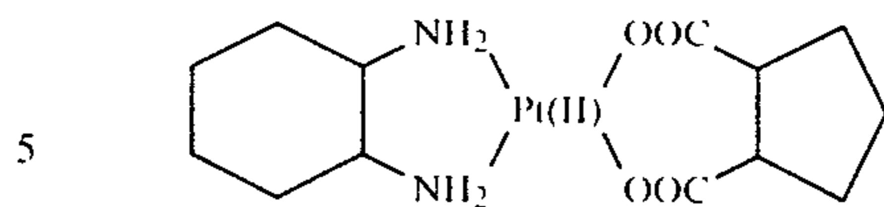
(trans-1,2-cyclopentanedicarboxylato)
