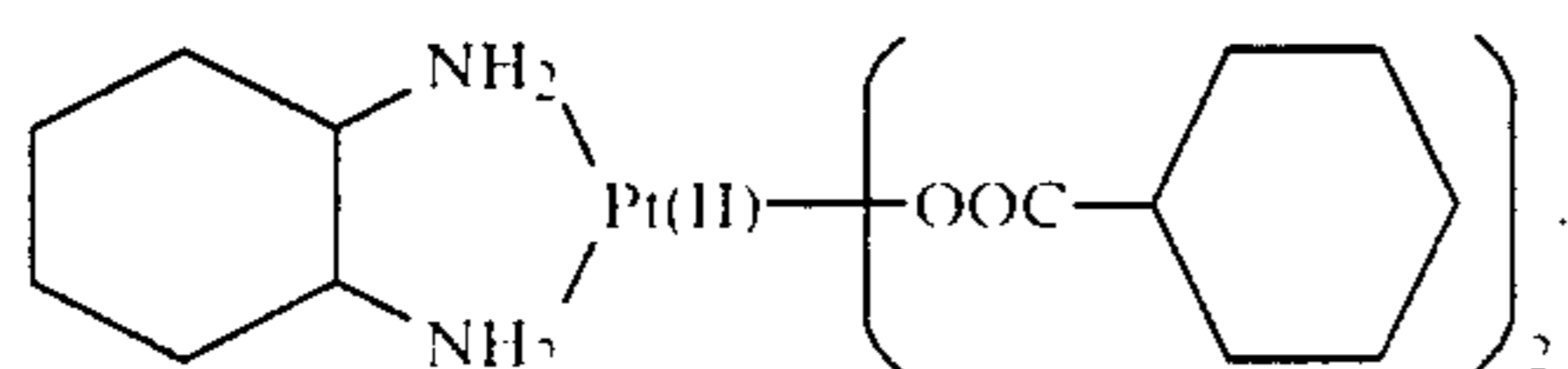
(bis-cyclohexanecarboxylato)
