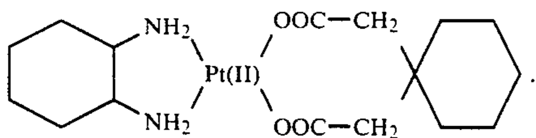
(cyclohexane-1,1-diacetato)
