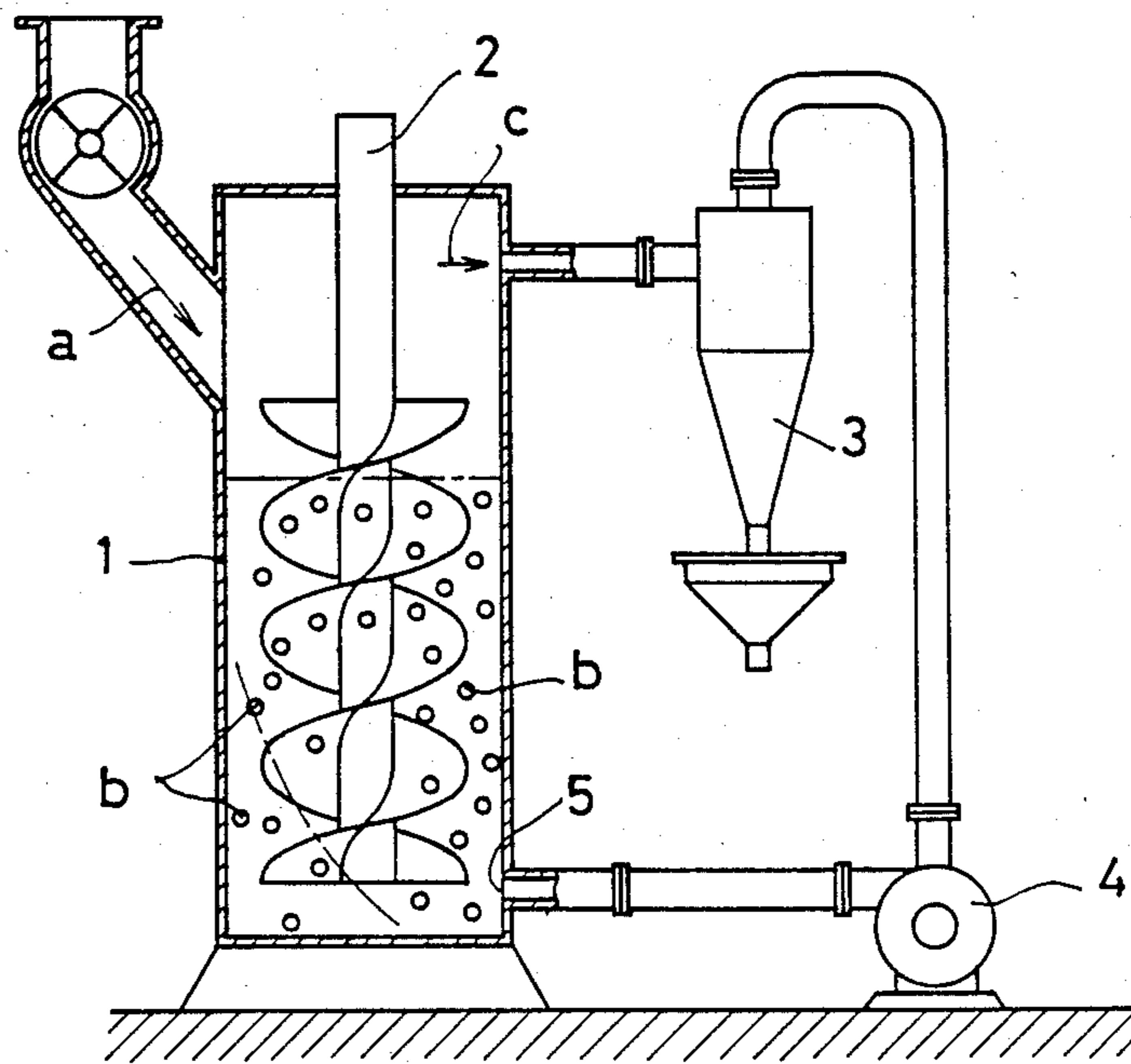
FIG. 7 PRIOR ART
