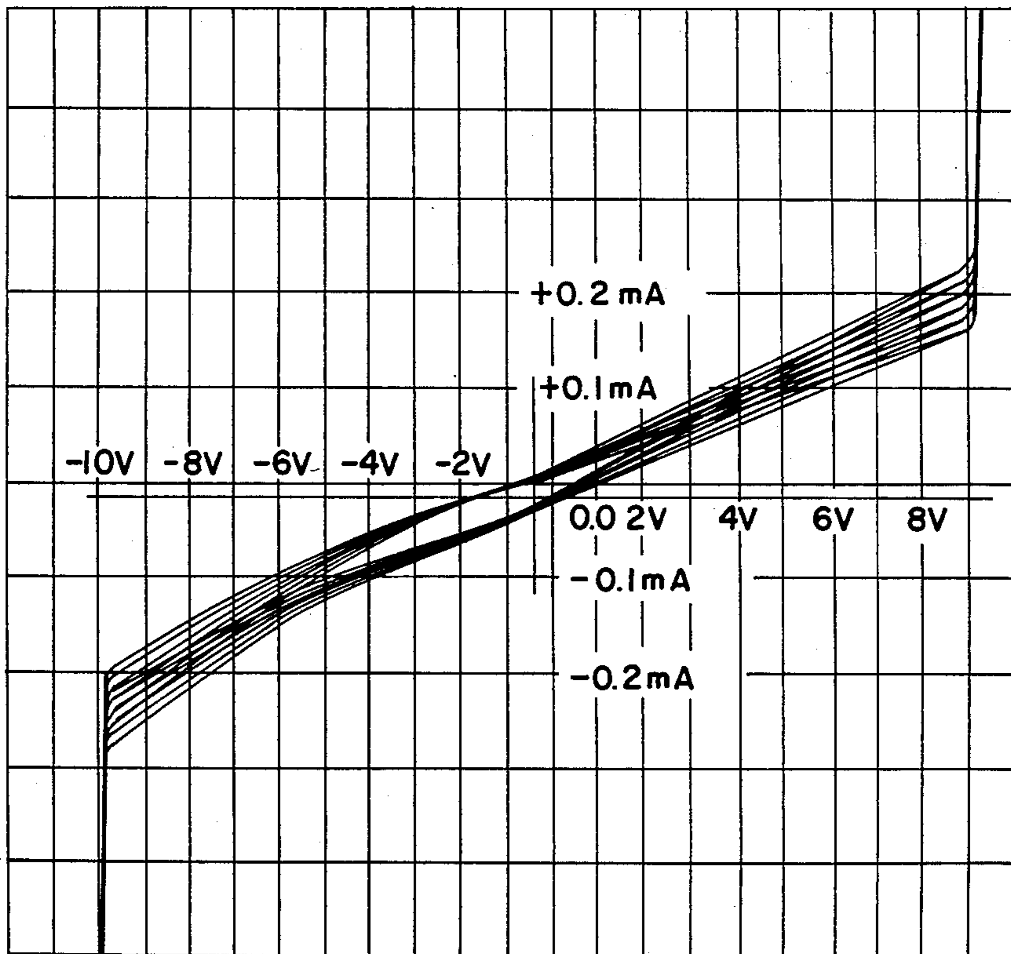
CYCLIC VOLTAMMOGRAM OF CSZ + 1m/o Cr CELL Pt ELECTRODES 850°C
