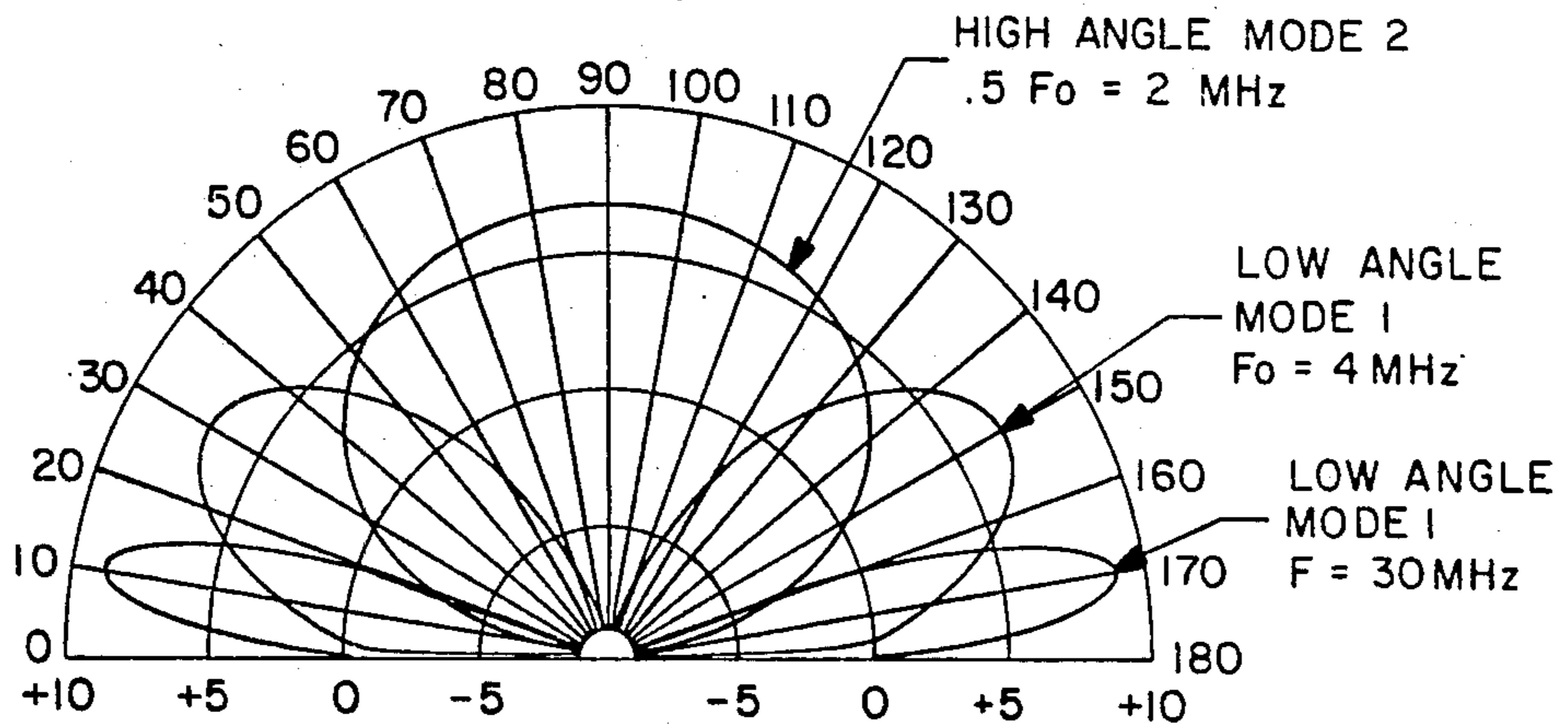
ELEVATION PATERN
