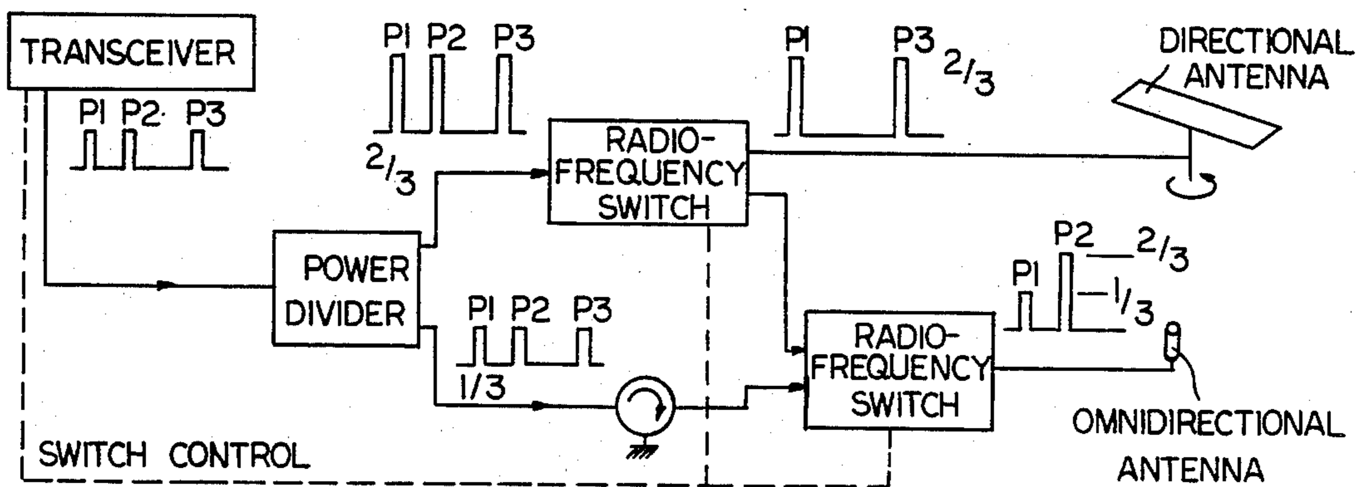
a) CONVENTIONAL SIDE-LOBE-SUPPRESSION (SLS) TECHNIQUE
