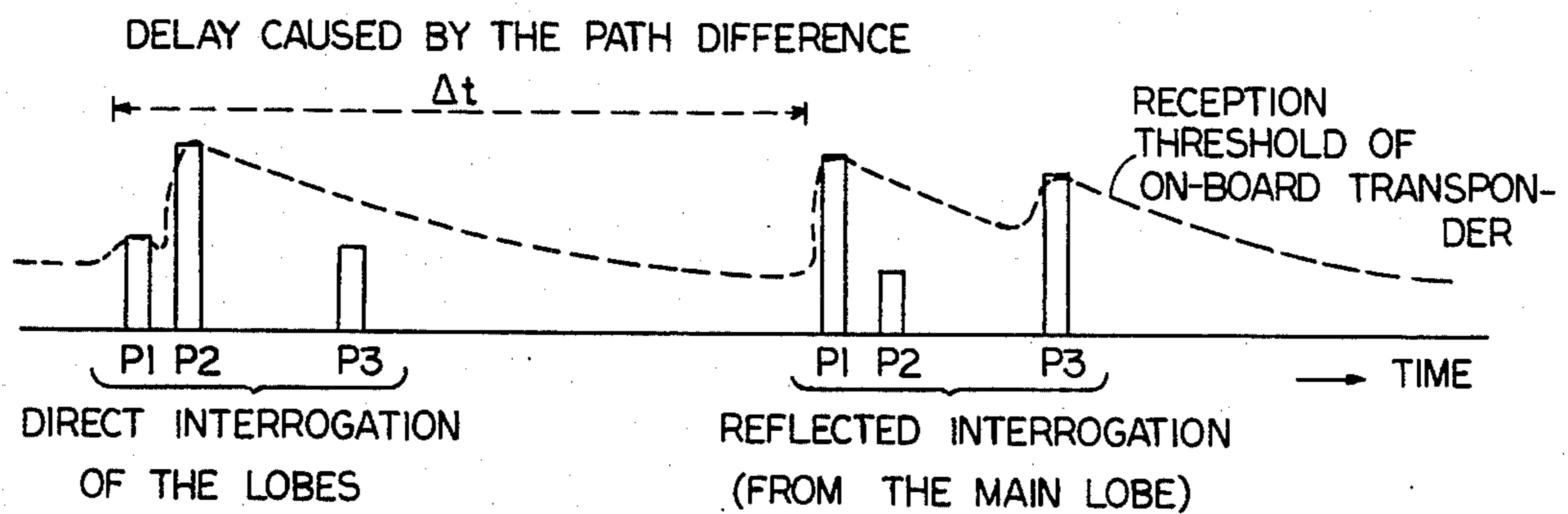
b) INPUT SIGNALS AT THE TRANSPONDER
