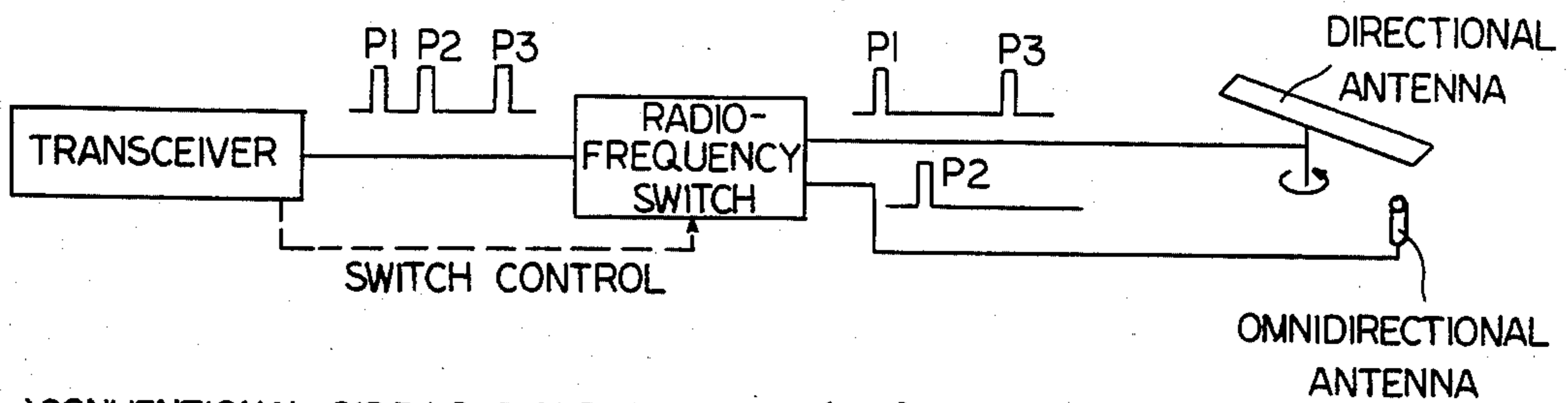
a) CONVENTIONAL SIDE-LOBE-SUPPRESSION (SLS) TECHNIQUE
