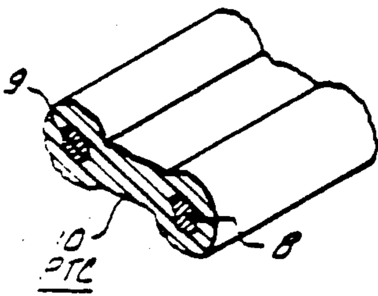
FIG. 5 (PRIOR ART)
