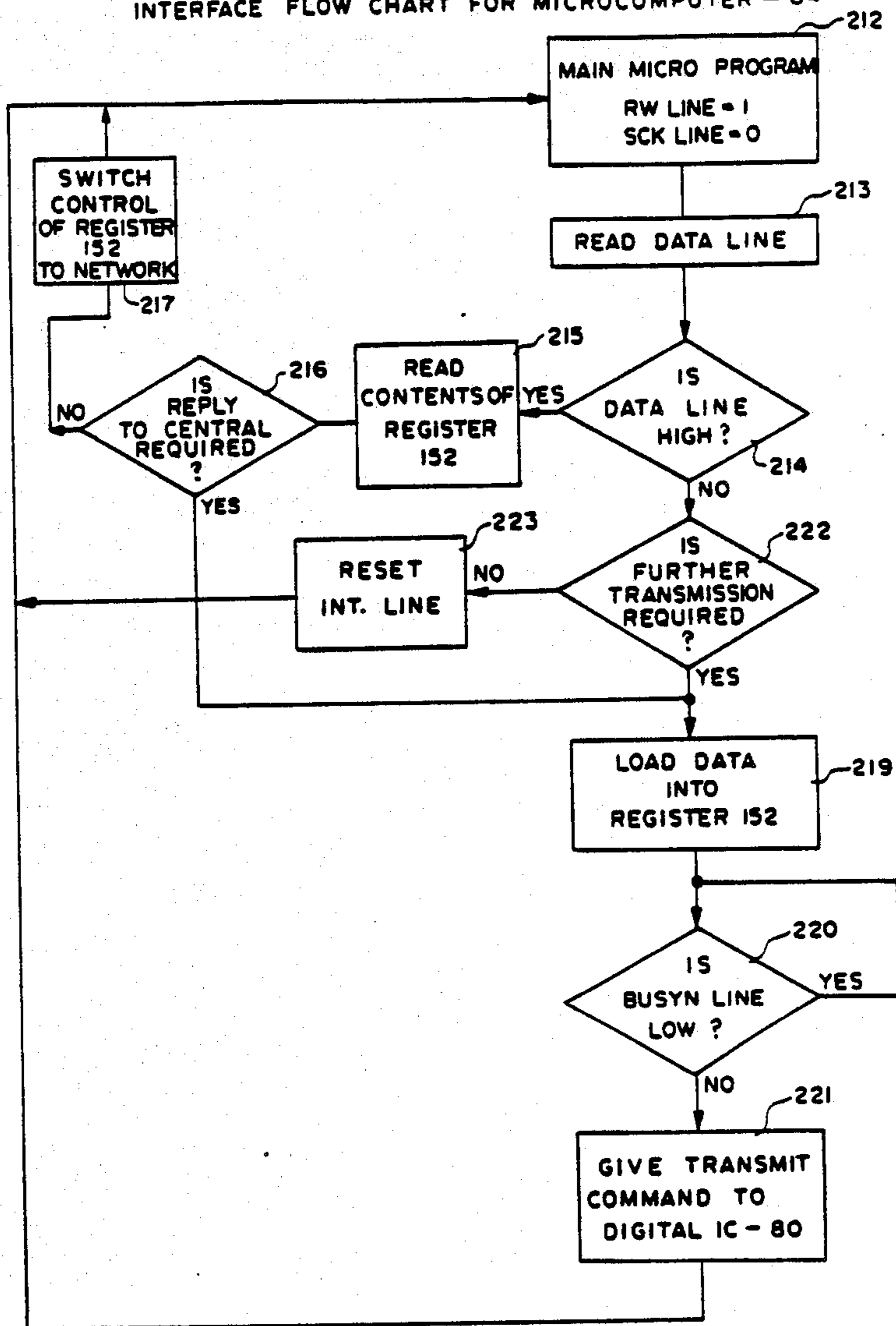
FIG. 15 INTERFACE FLOW CHART FOR MICROCOMPUTER - 84
