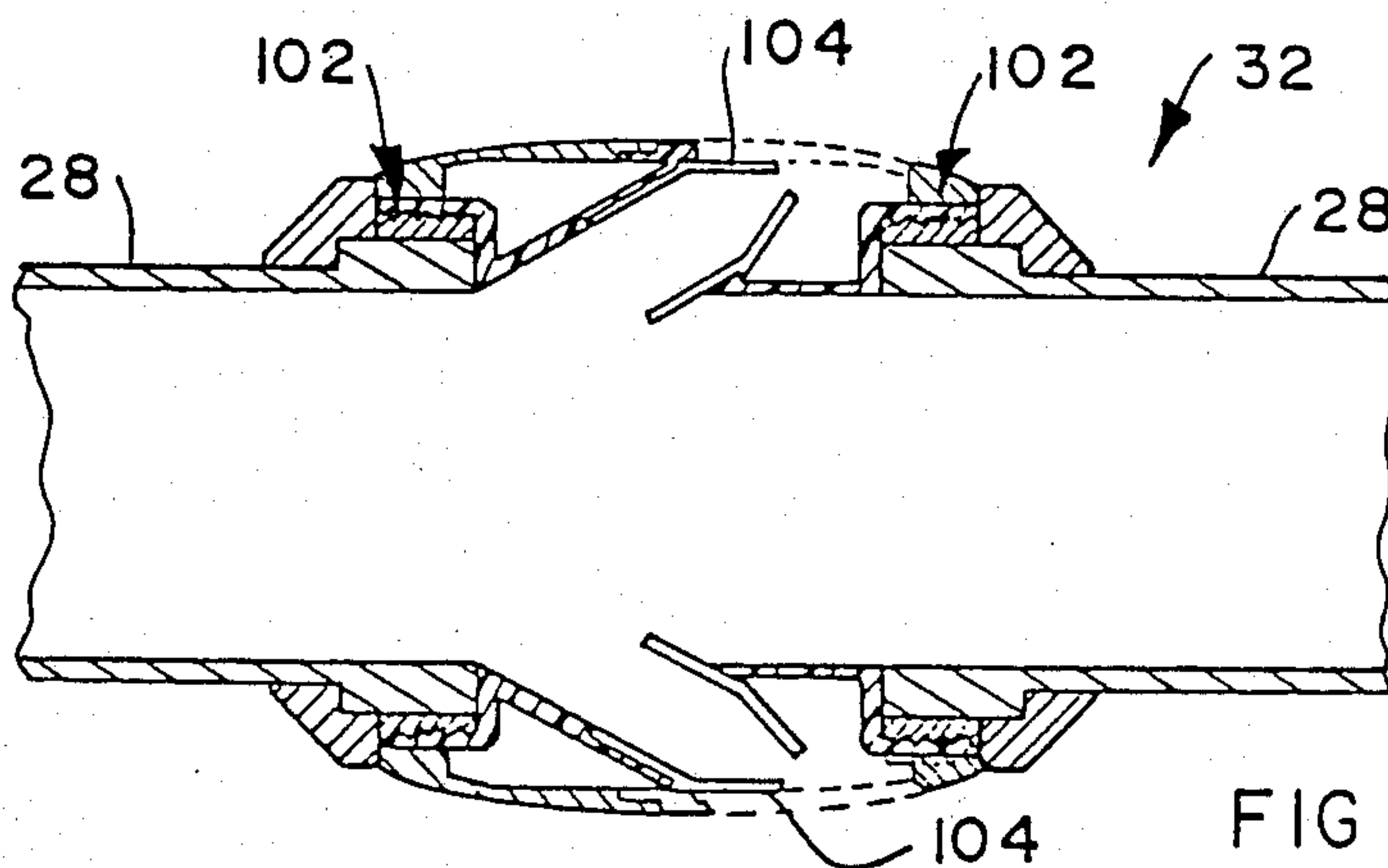
FIG 6
