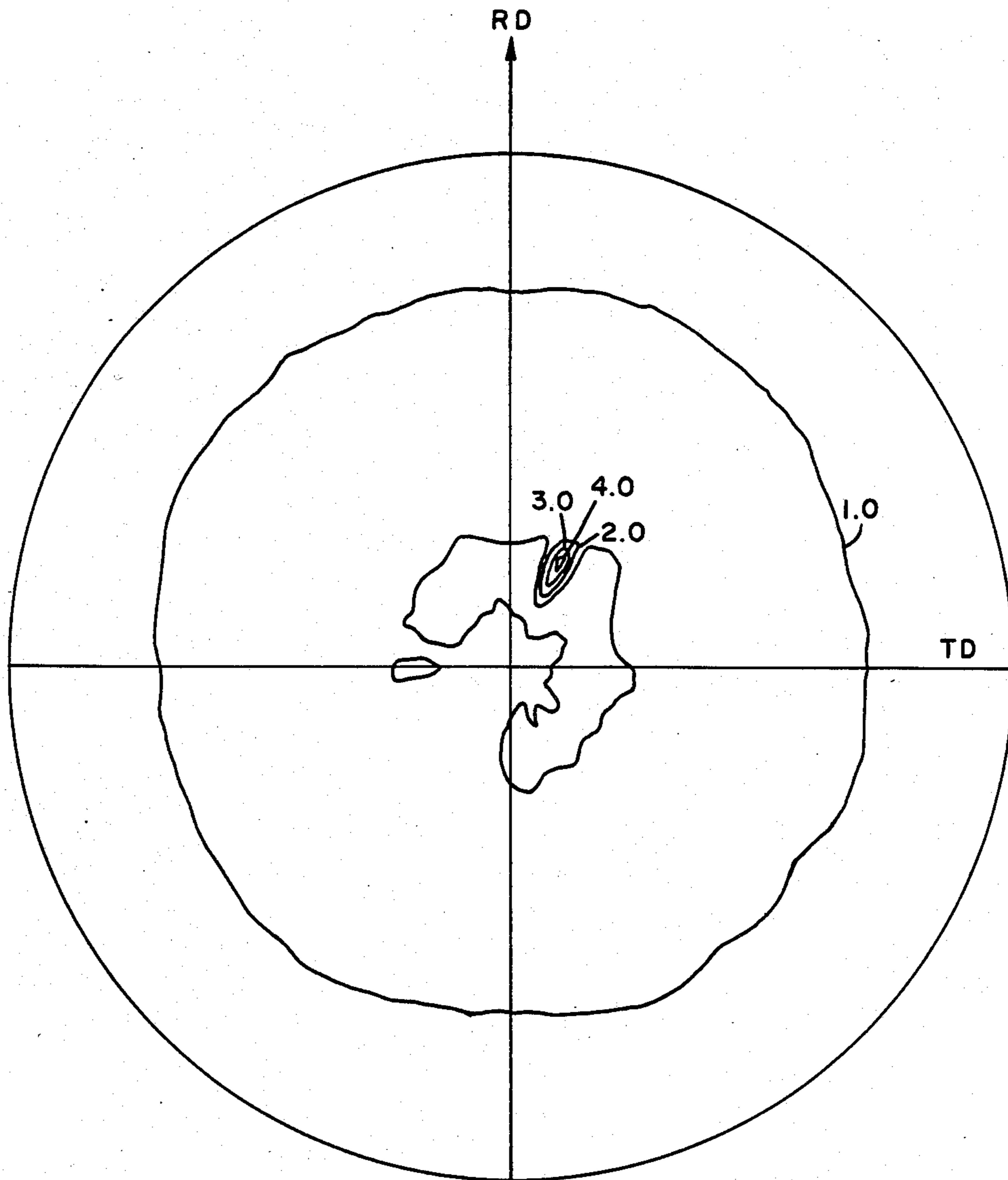
Cu-Be SUBSTRATE (110) POLE FIGURE
