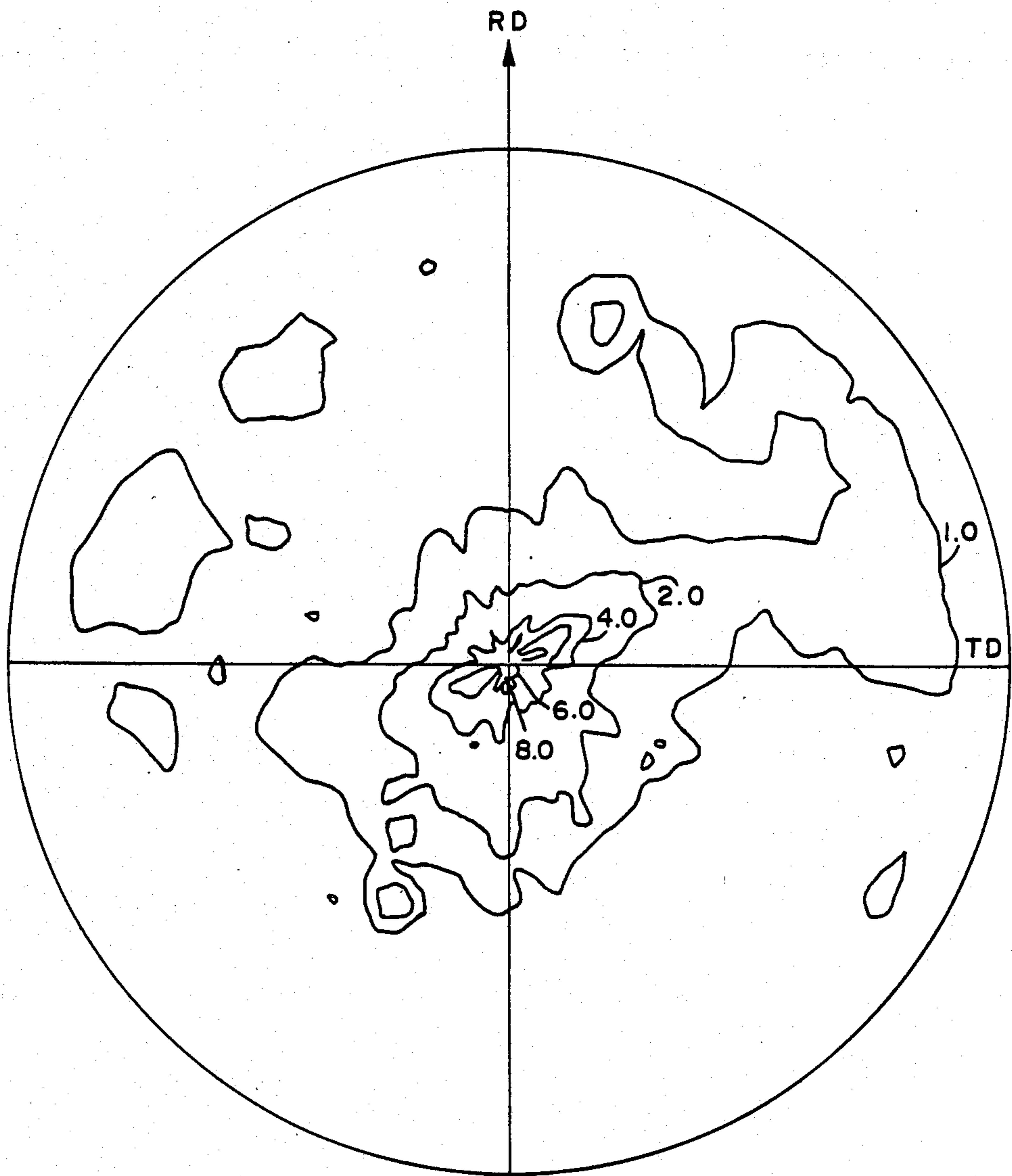
Cu-Be SUBSTRATE (200) POLE FIGURE
