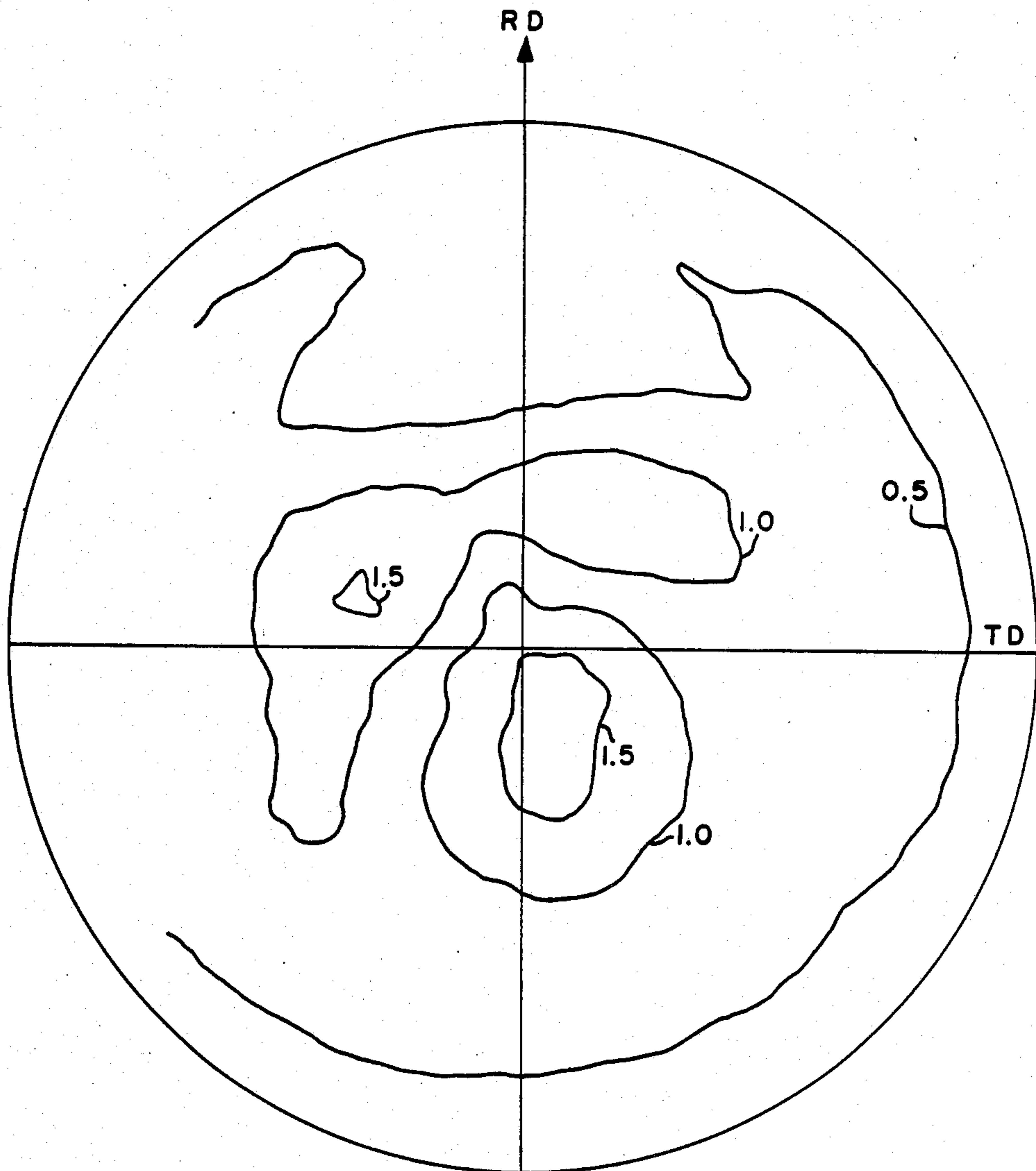
STEEL SUBSTRATE (110) POLE FIGURE
