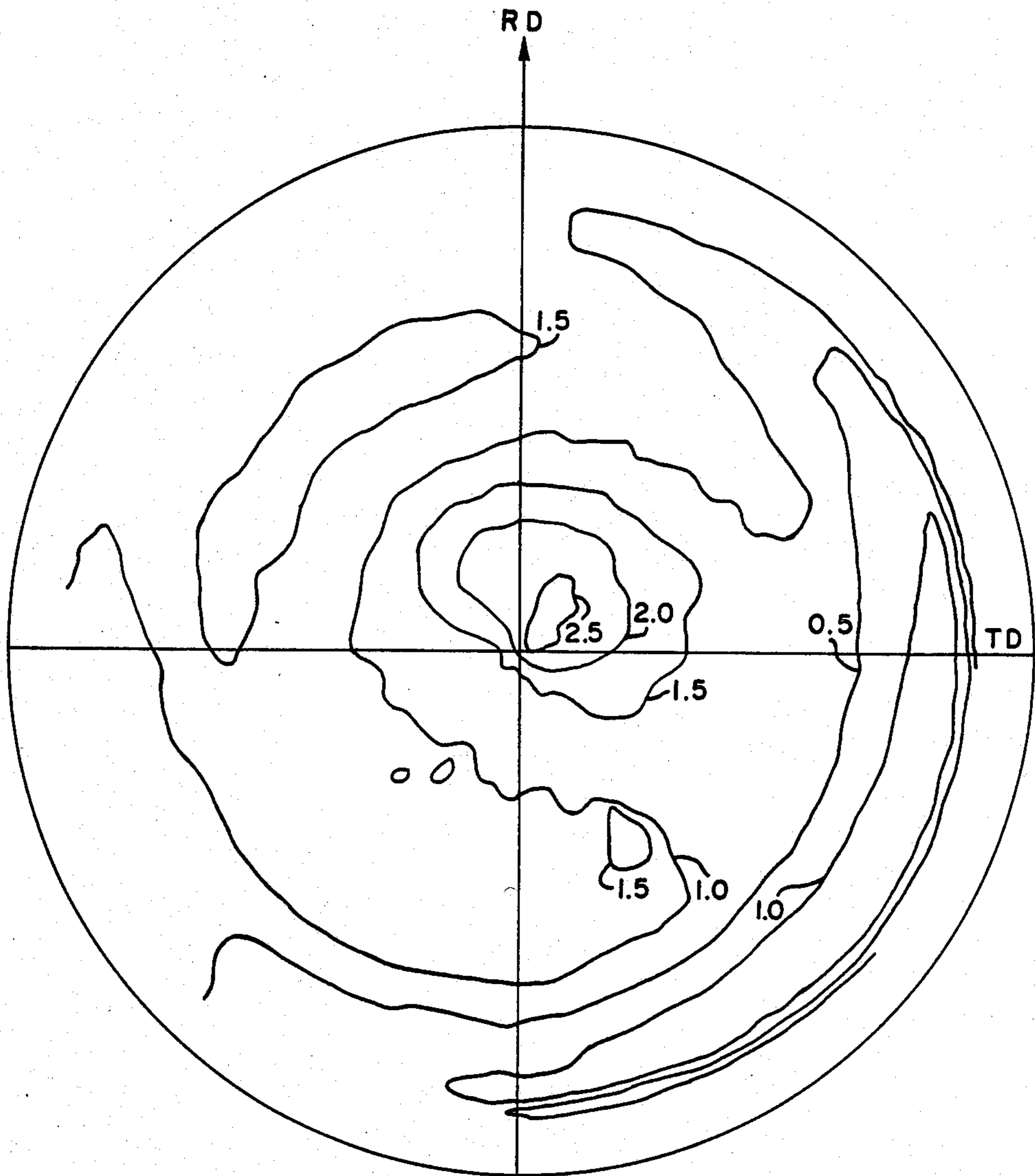
STEEL SUBSTRATE (200) POLE FIGURE
