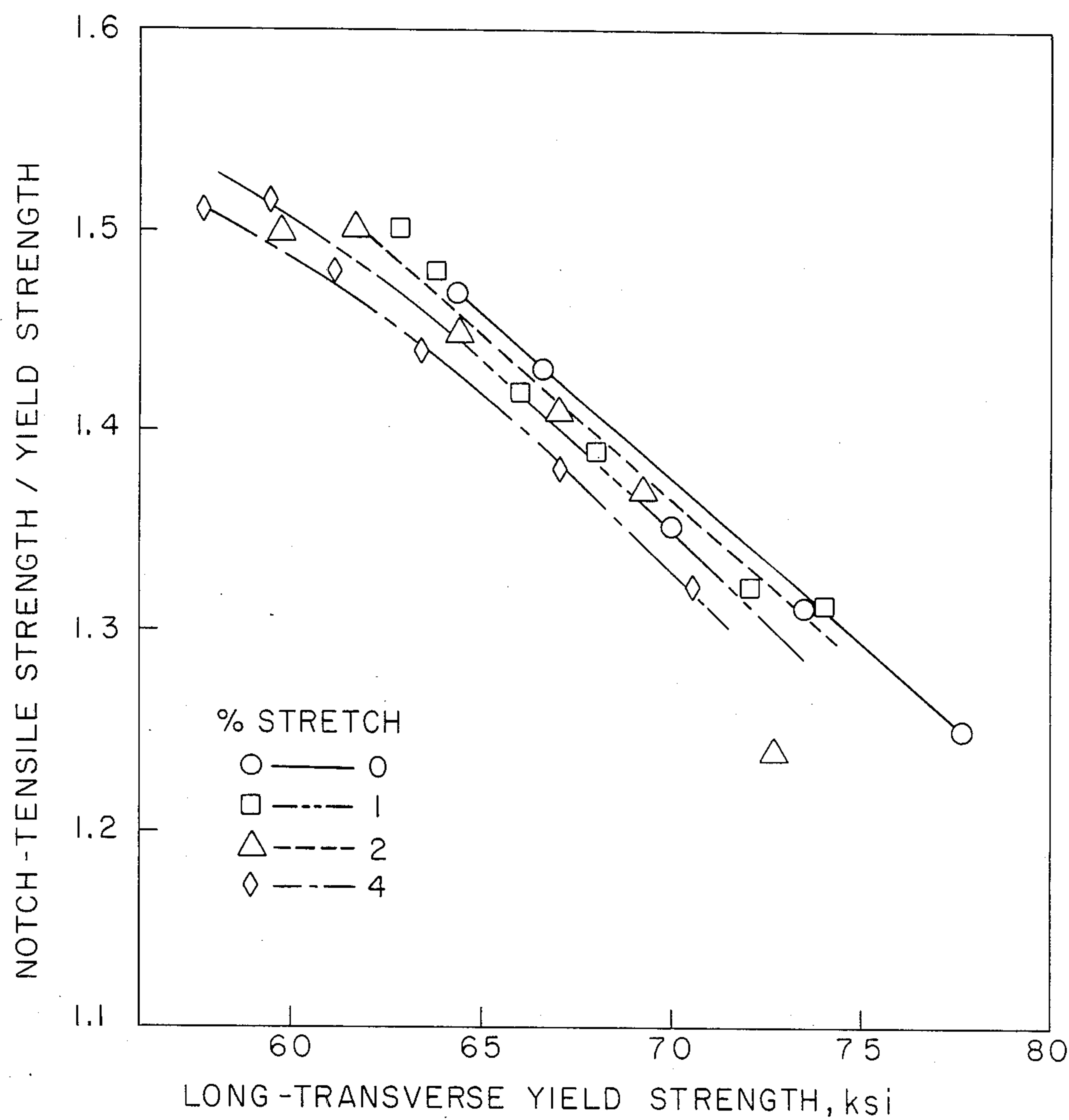
EFFECT OF STRETCH ON LONG-TRANSVERSE TOUGHNESS
