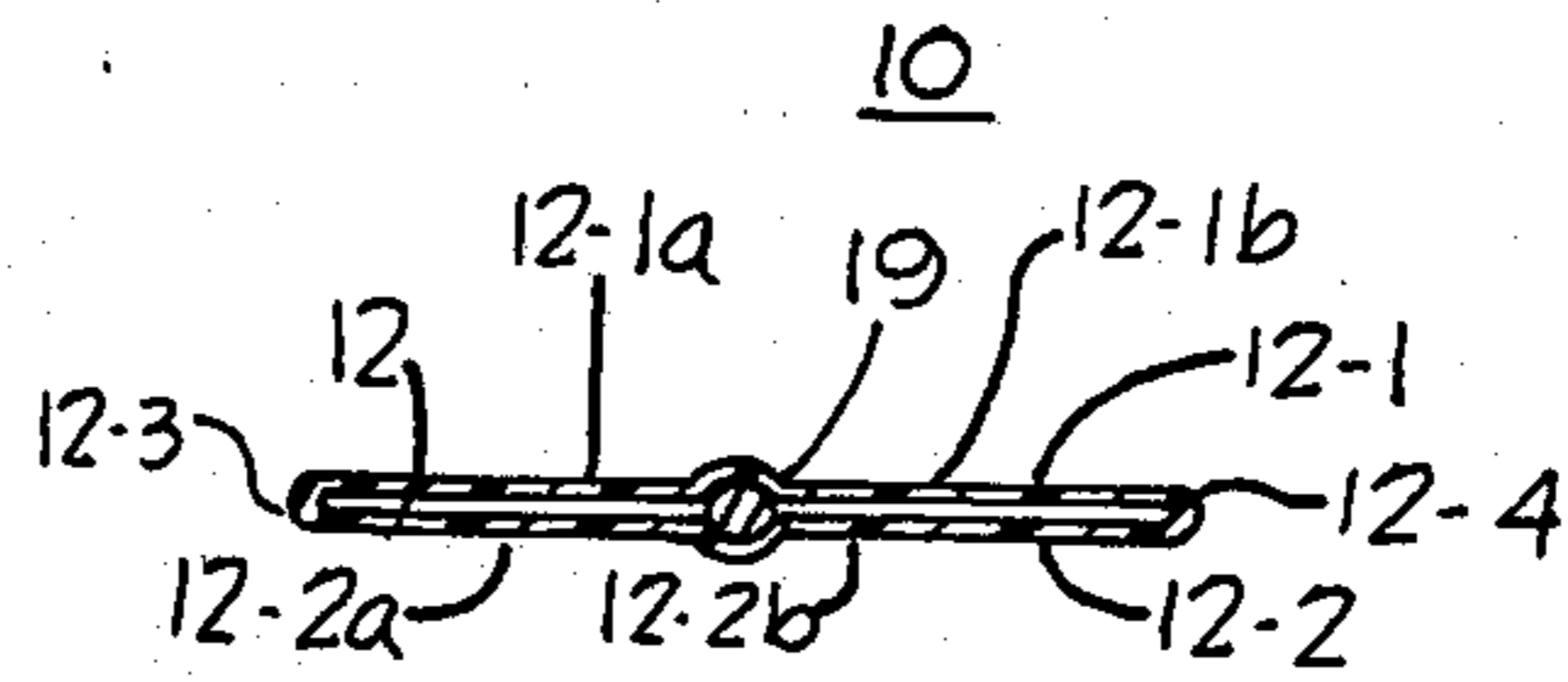
PRIOR ART FIG. 1b
