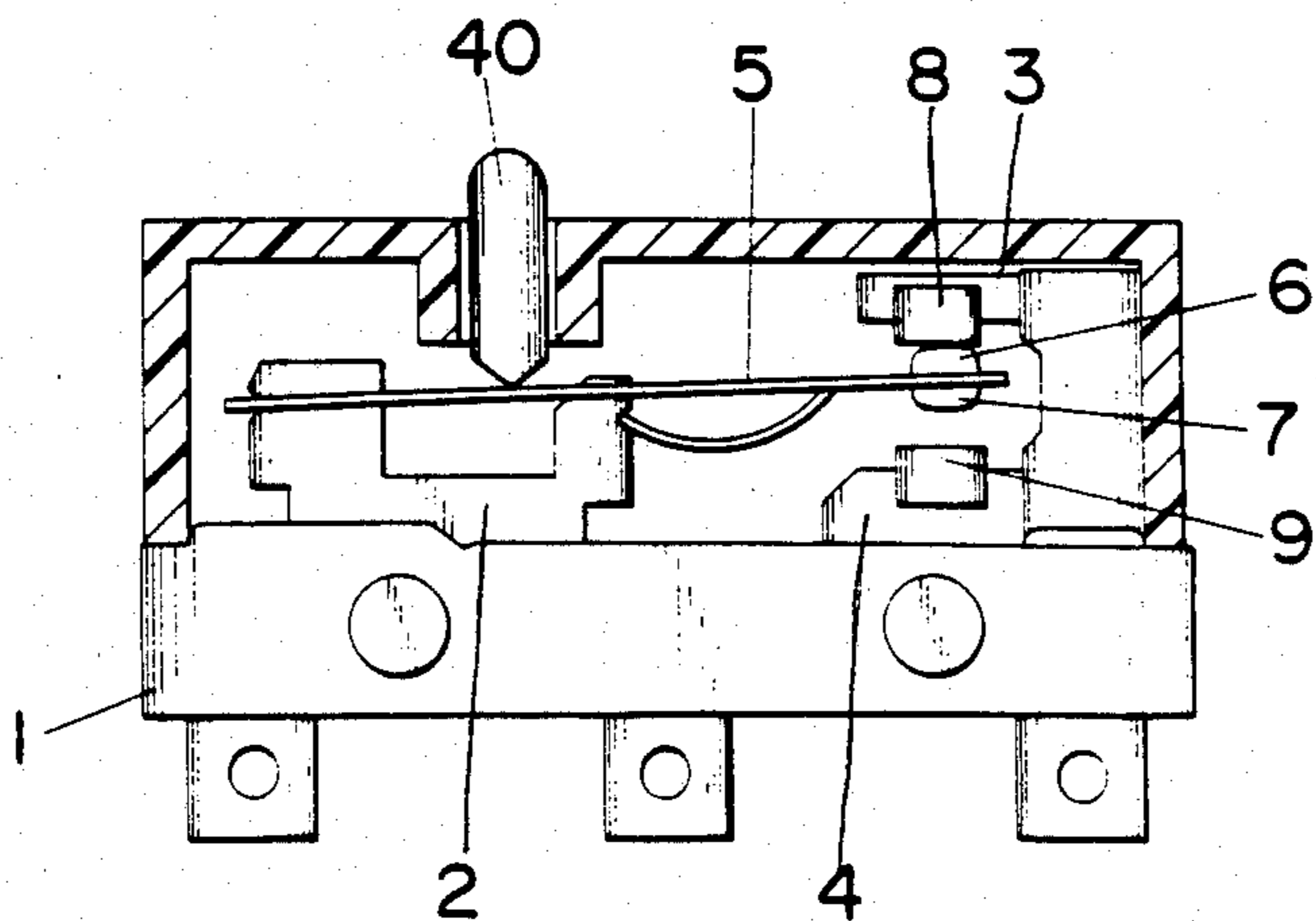
Fig. 4 (PRIOR ART)
