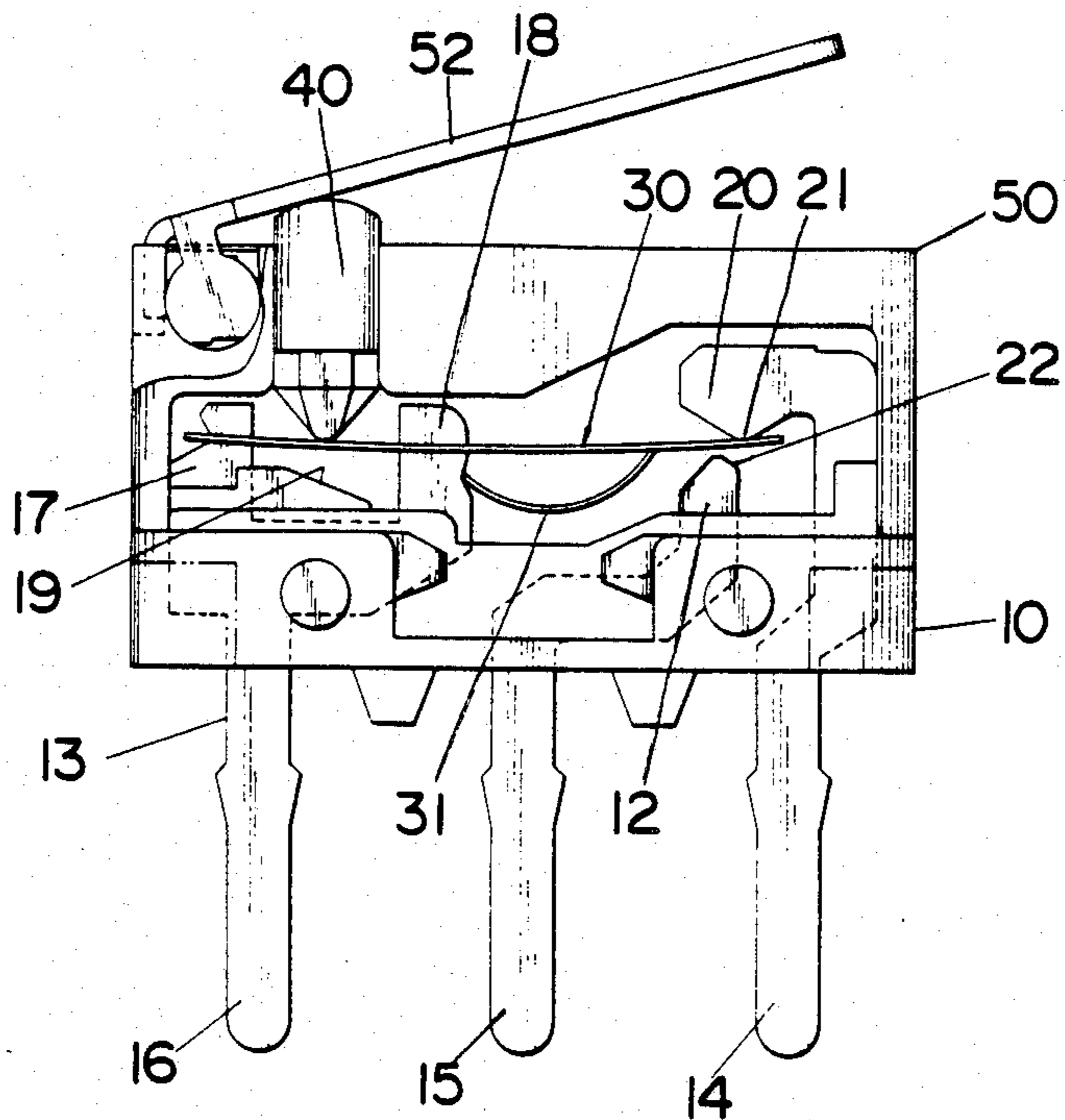
Fig. 4 (PRIOR ART)
