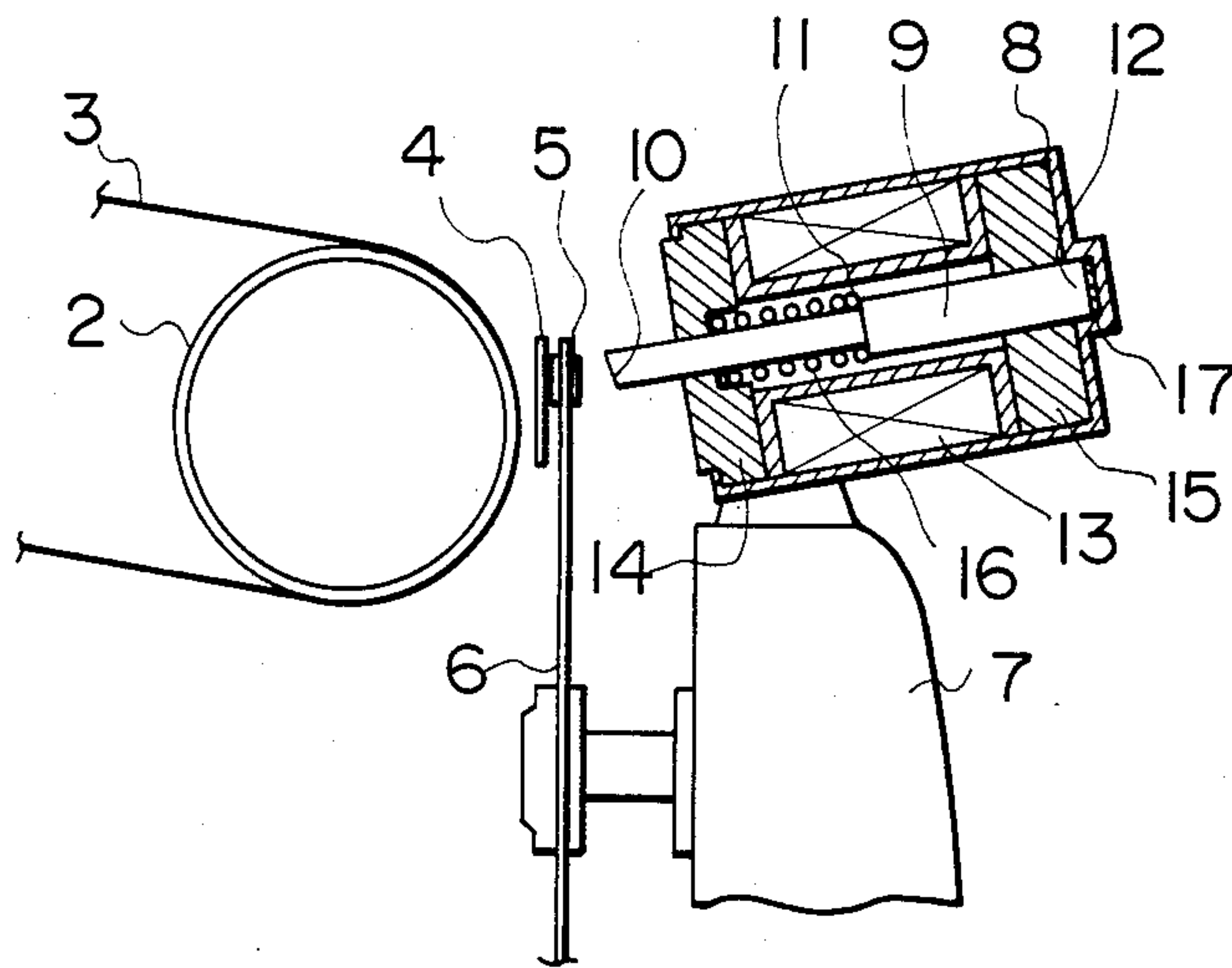
FIG. 5 PRIOR ART
