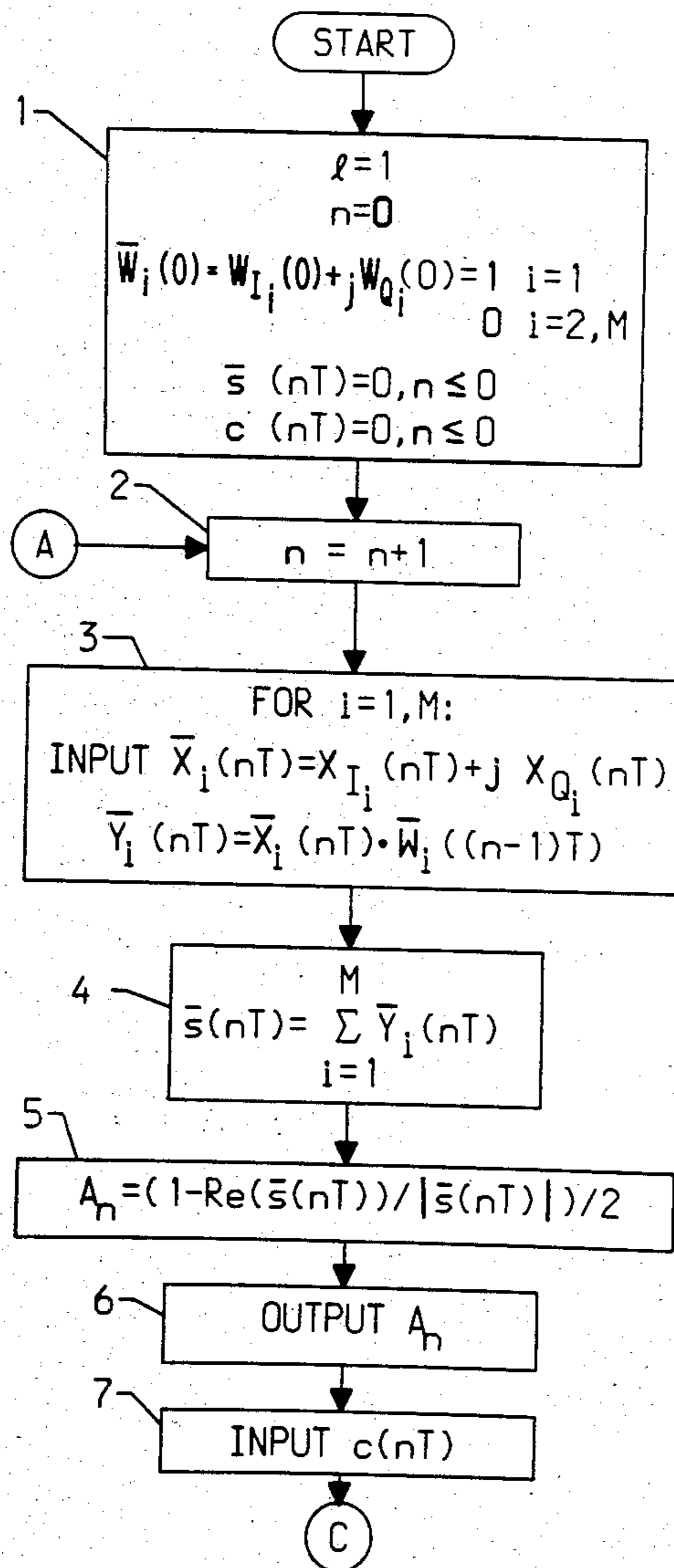
FIG. 6 BASE STATION FLOWCHART
