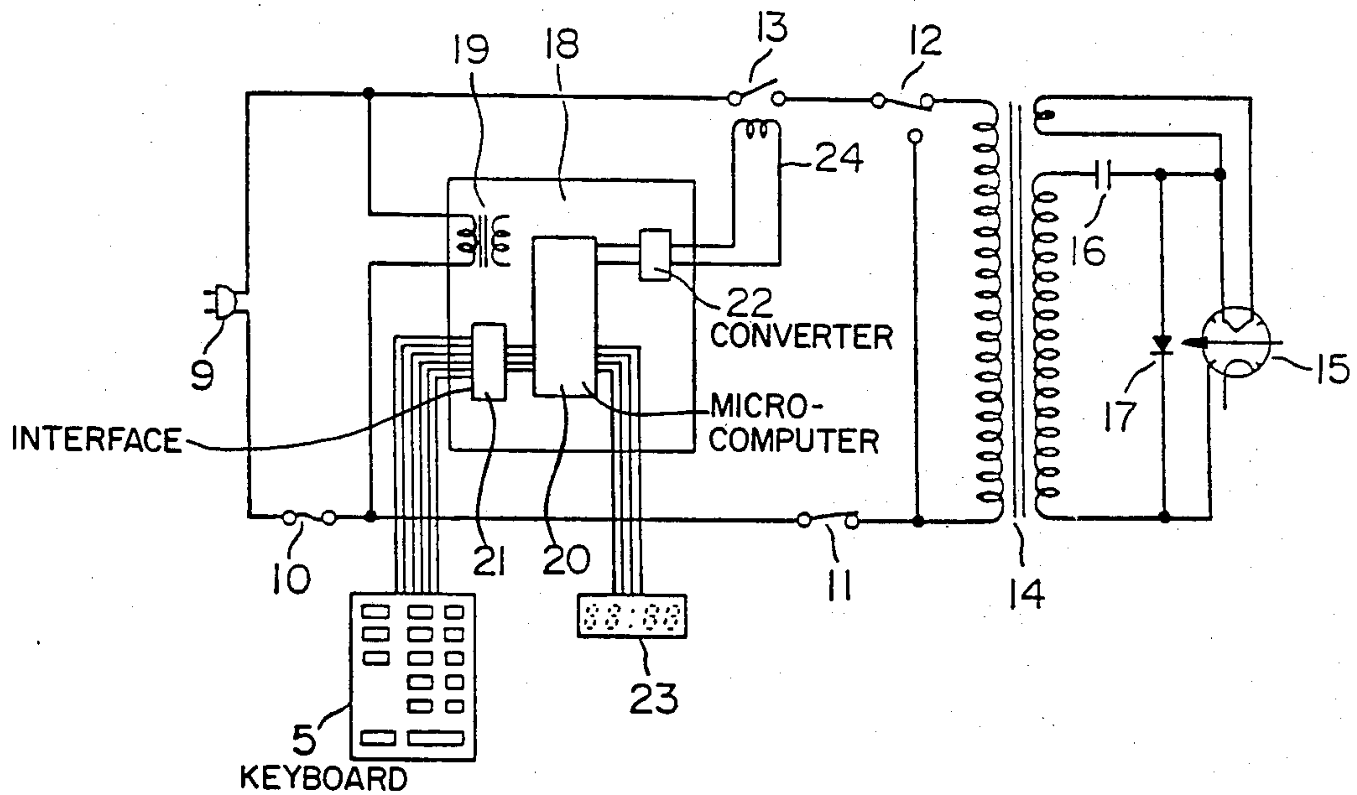
FIG. 2 PRIOR ART
