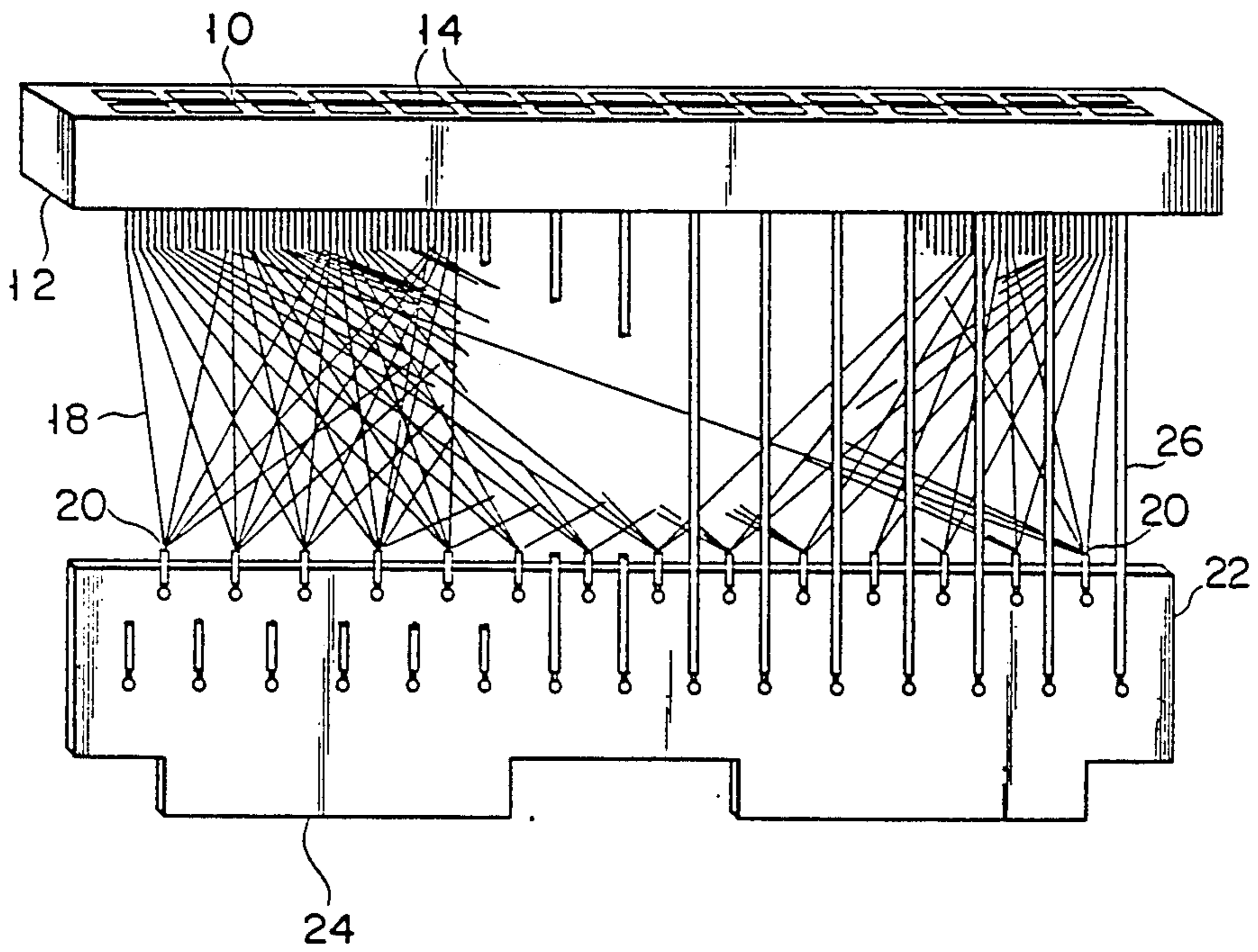
FIG. 4 PRIOR ART
