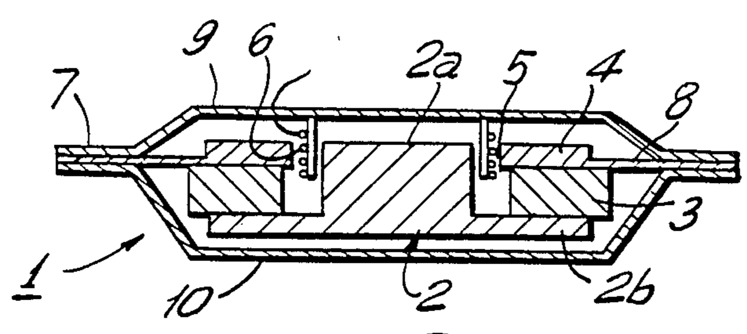
FIG. 1 (PRIOR ART)
