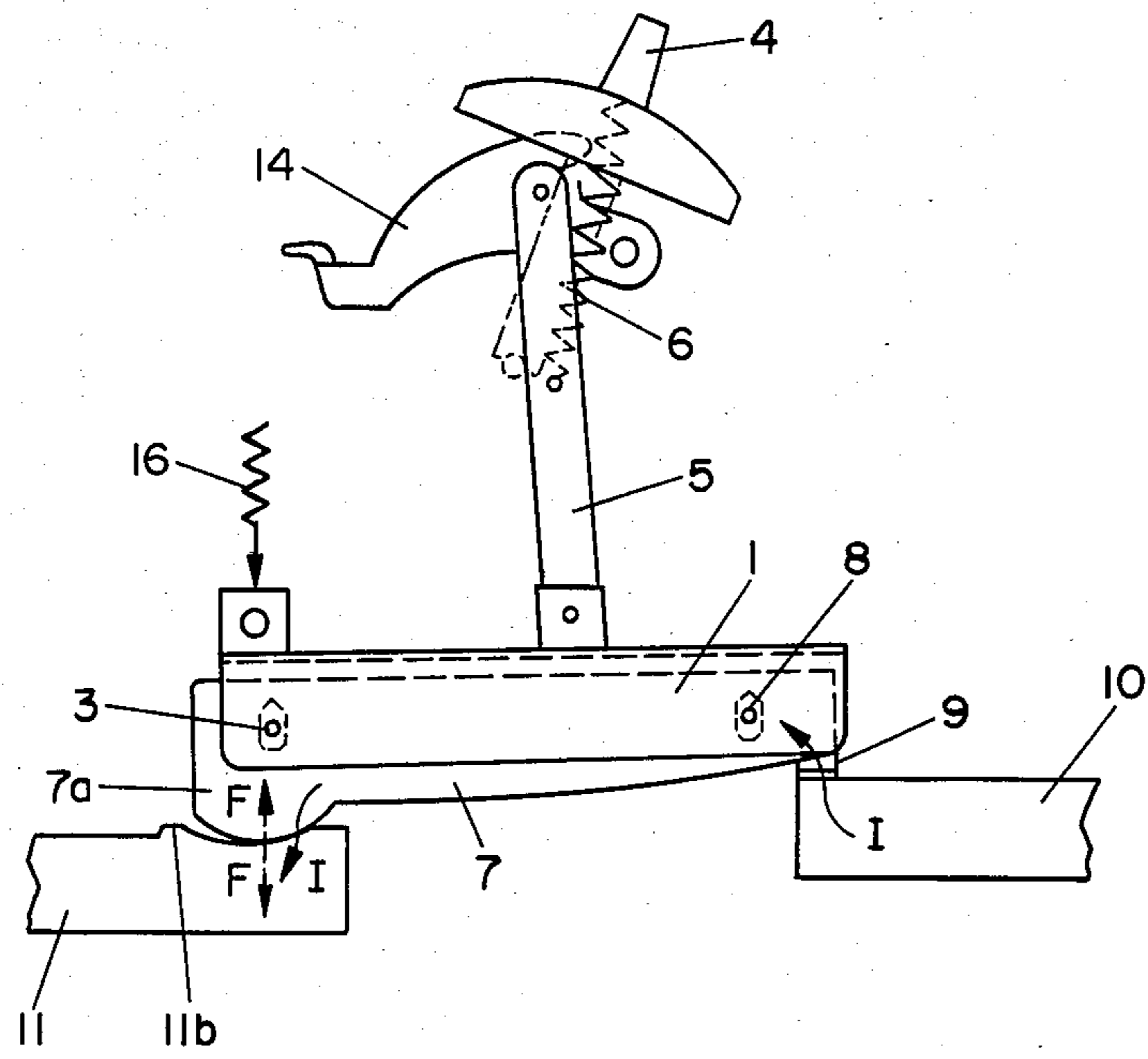
FIG. 8 PRIOR ART
