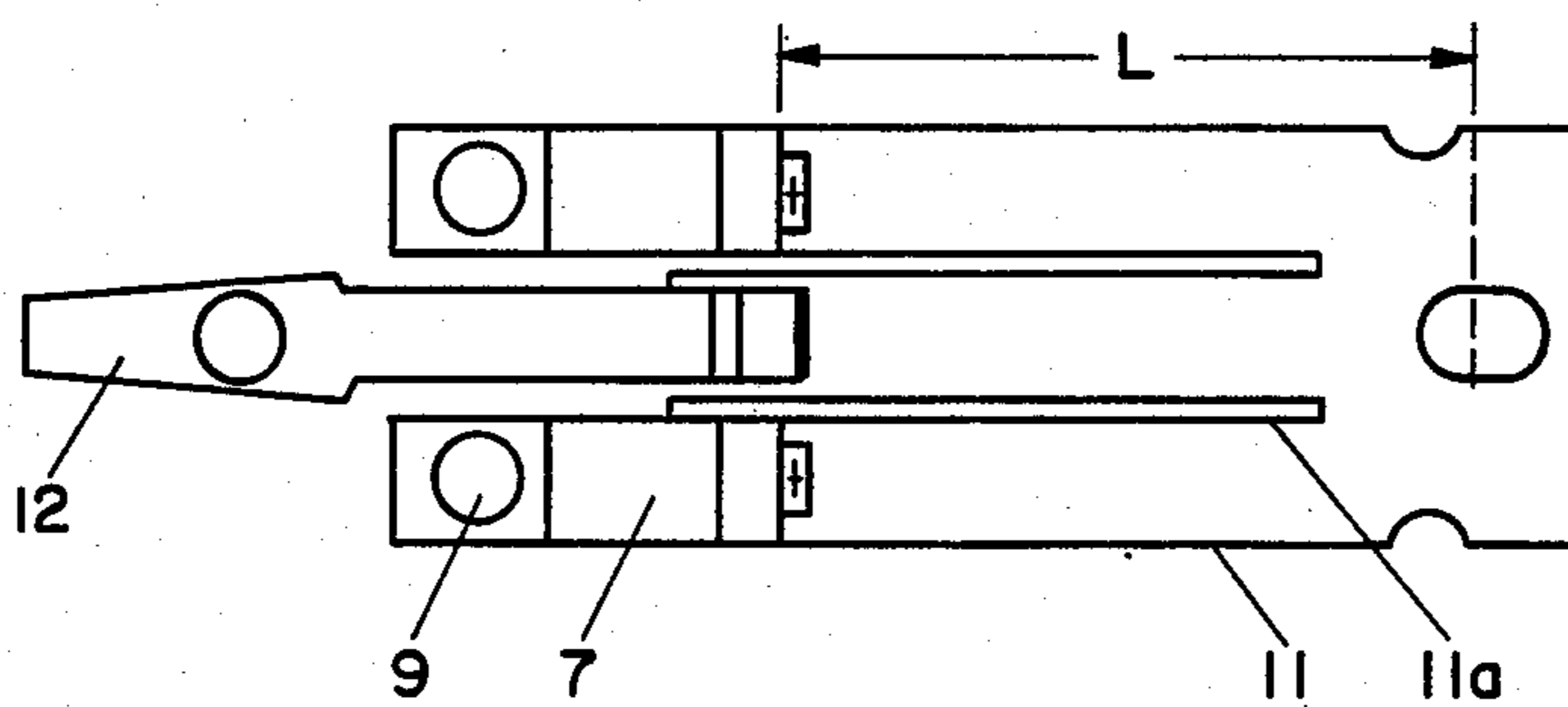
FIG. 7 PRIOR ART
