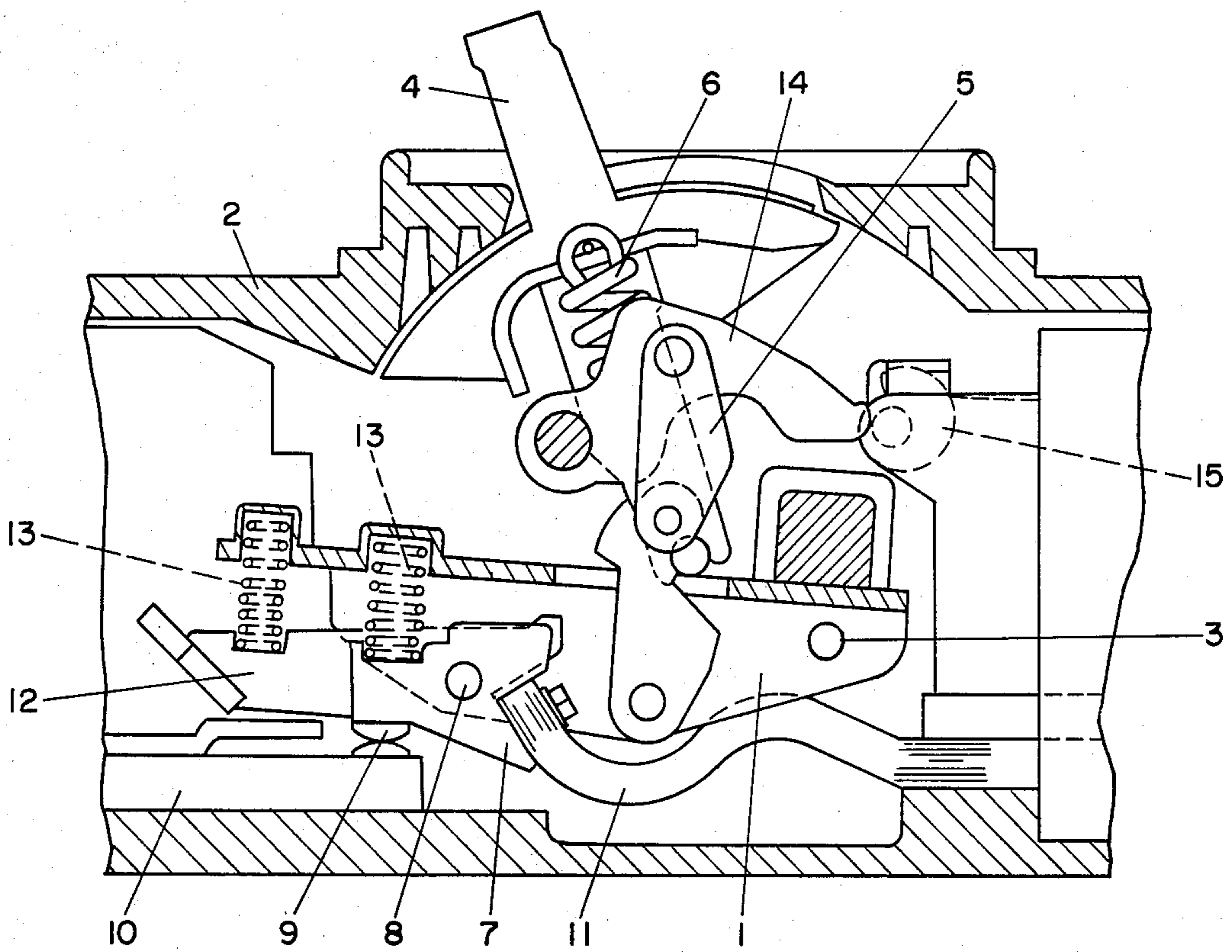
FIG. 6 PRIOR ART
