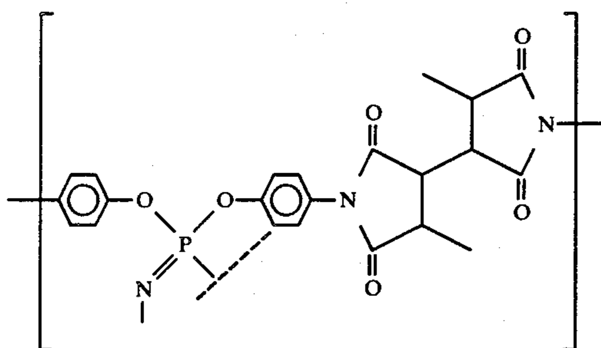
(d) Reaction of 6 with a Mixture of Maleic Anhydride and Perfluorosuccinic Anhydride, Conversion of the Maleamic Acid to Maleimide and Polymerization of the Imide
