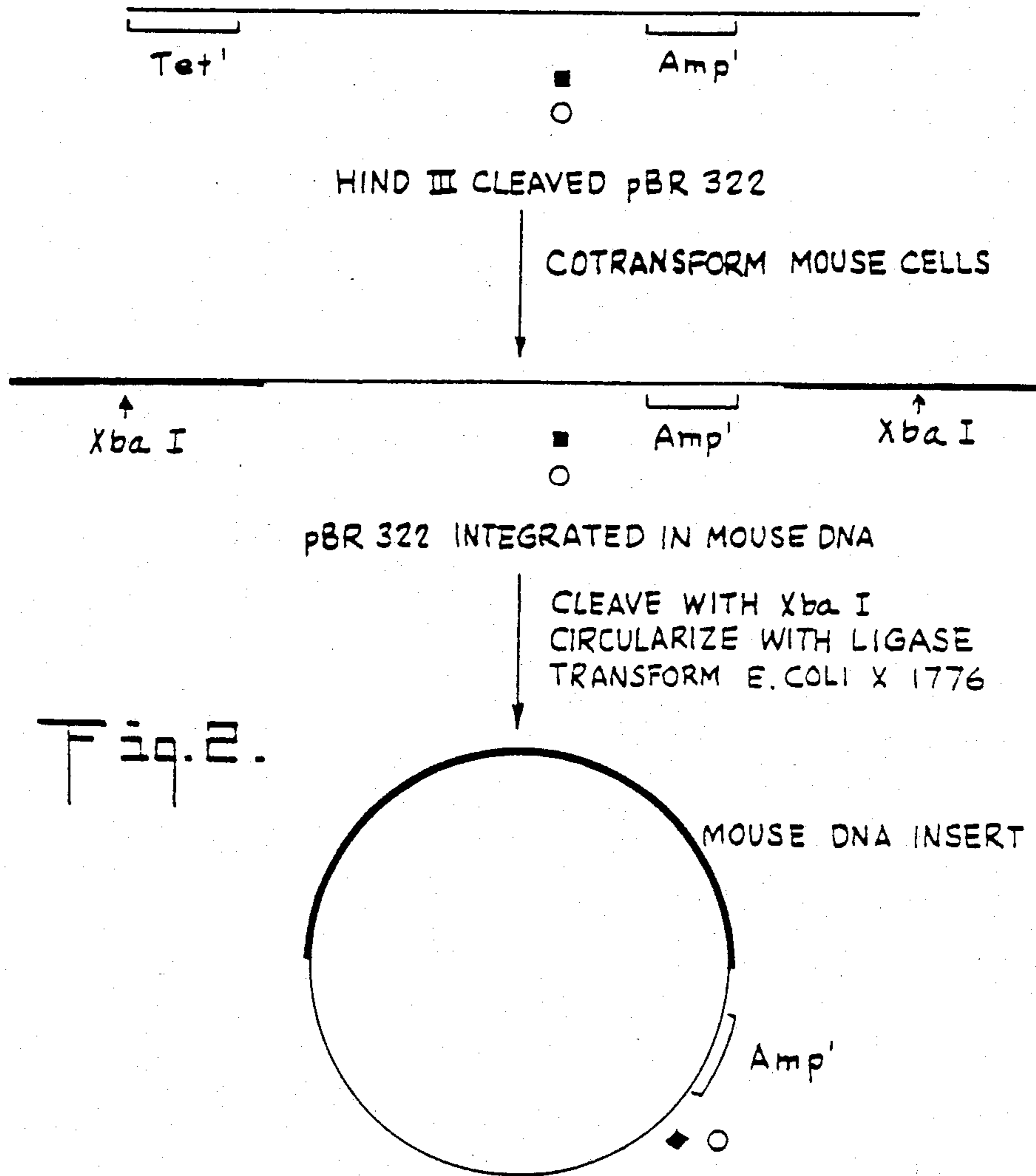
SCHEME FOR THE RESCUE OF BACTERIAL PLASMIDS FROM TRANSFORMED CULTURED CELLS USING DOUBLE SELECTION TECHNIQUES.
