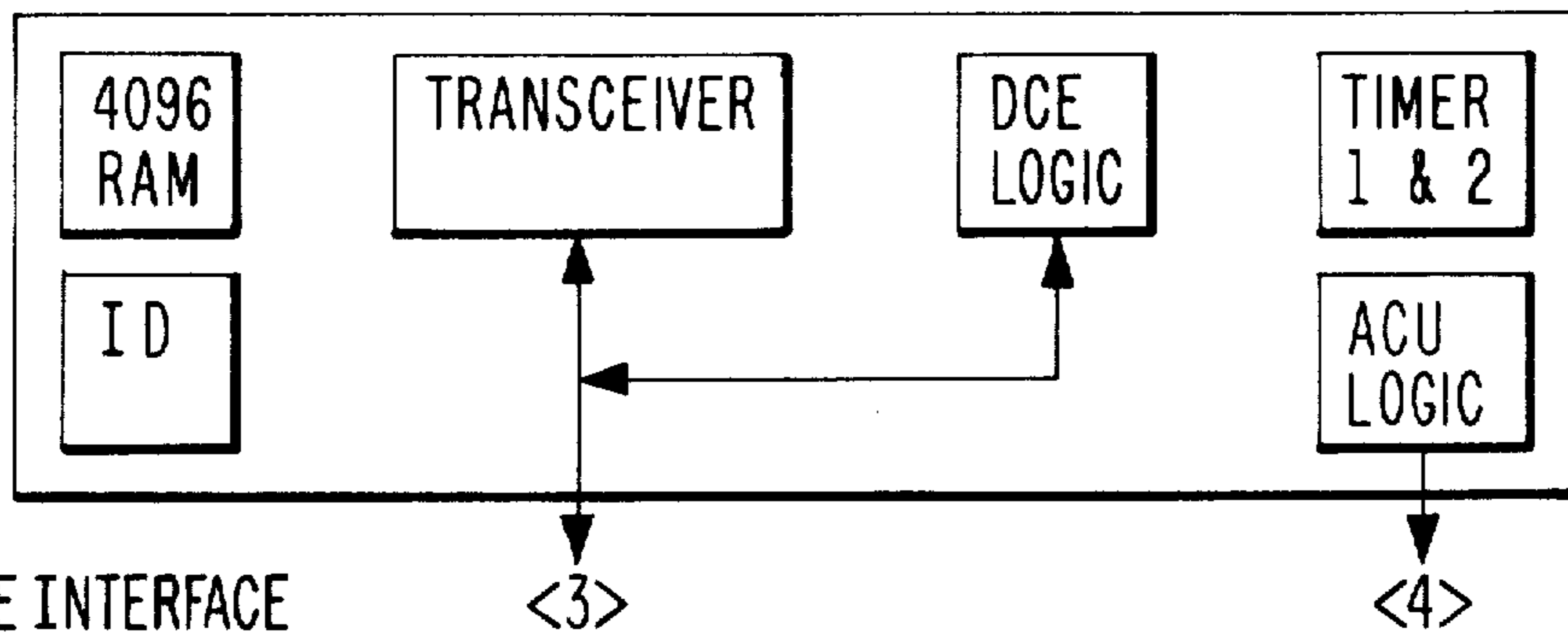
FIG.1C. LINE ADAPTER.
