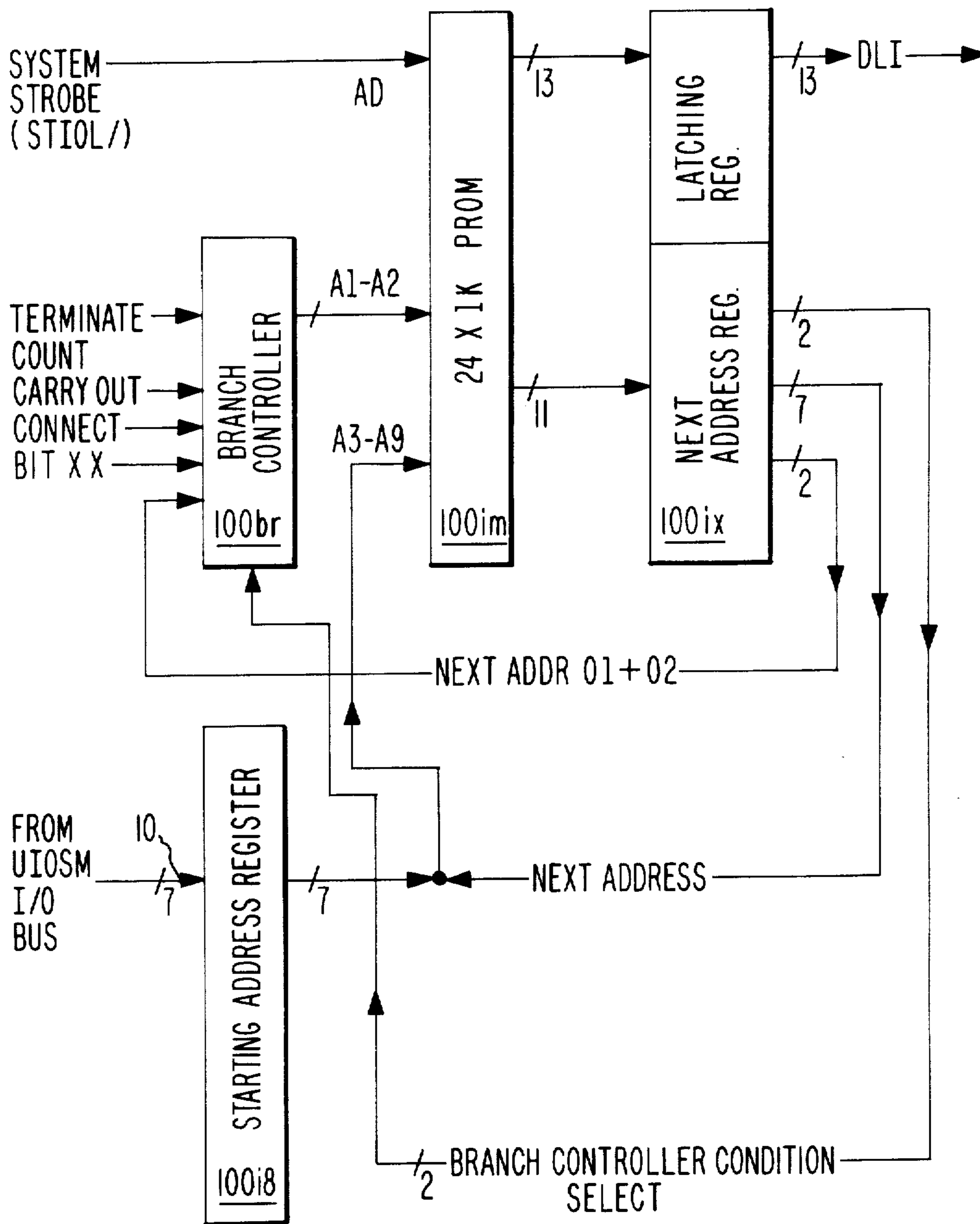
FIG. 8. DLP SEQUENCER BLOCK DIAGRAM.
