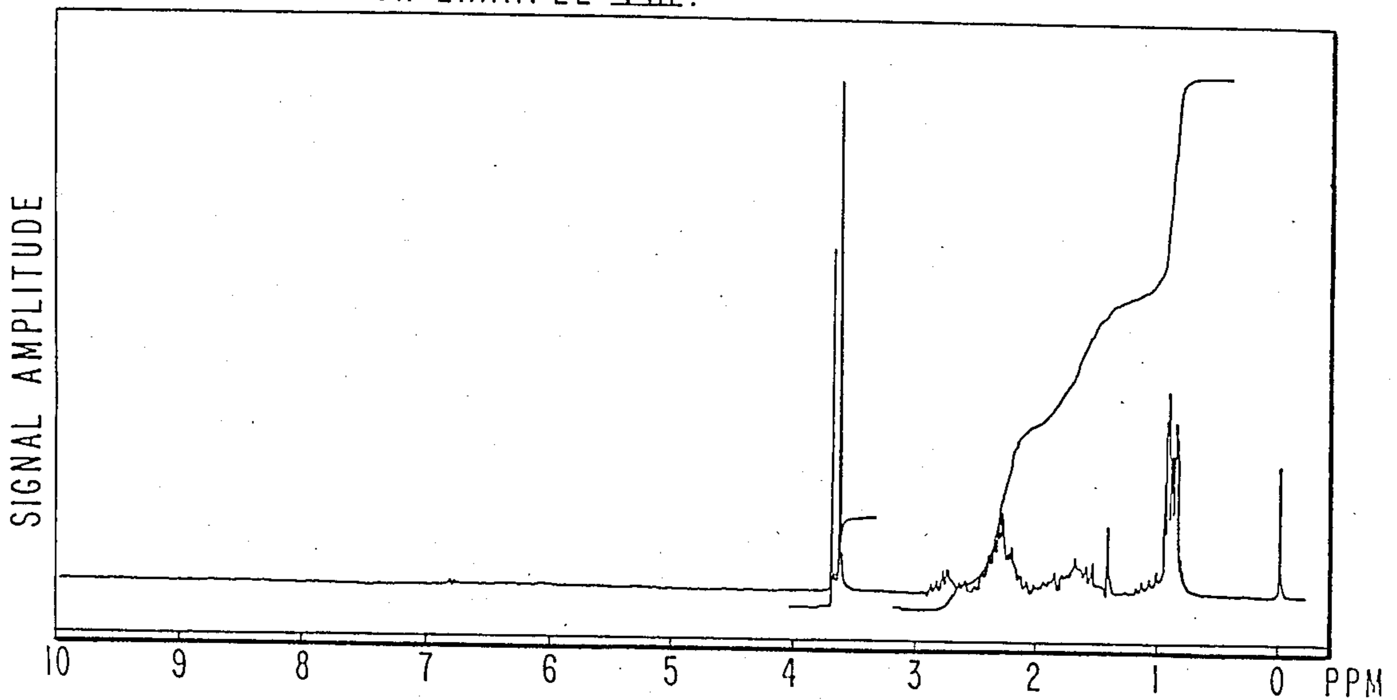
NMR SPECTRUM FOR EXAMPLE VIII.
