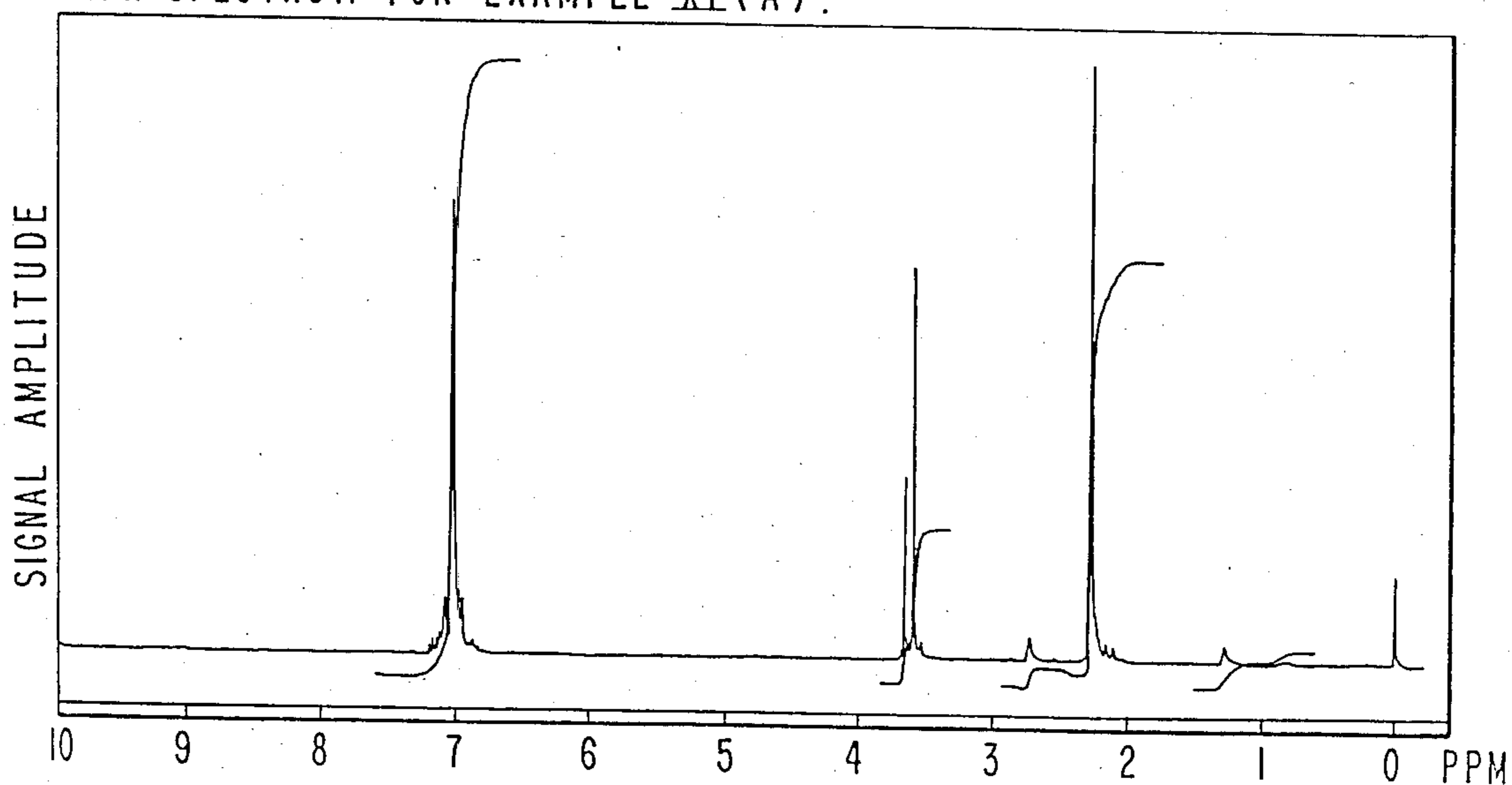
NMR SPECTRUM FOR EXAMPLE XI(A).
