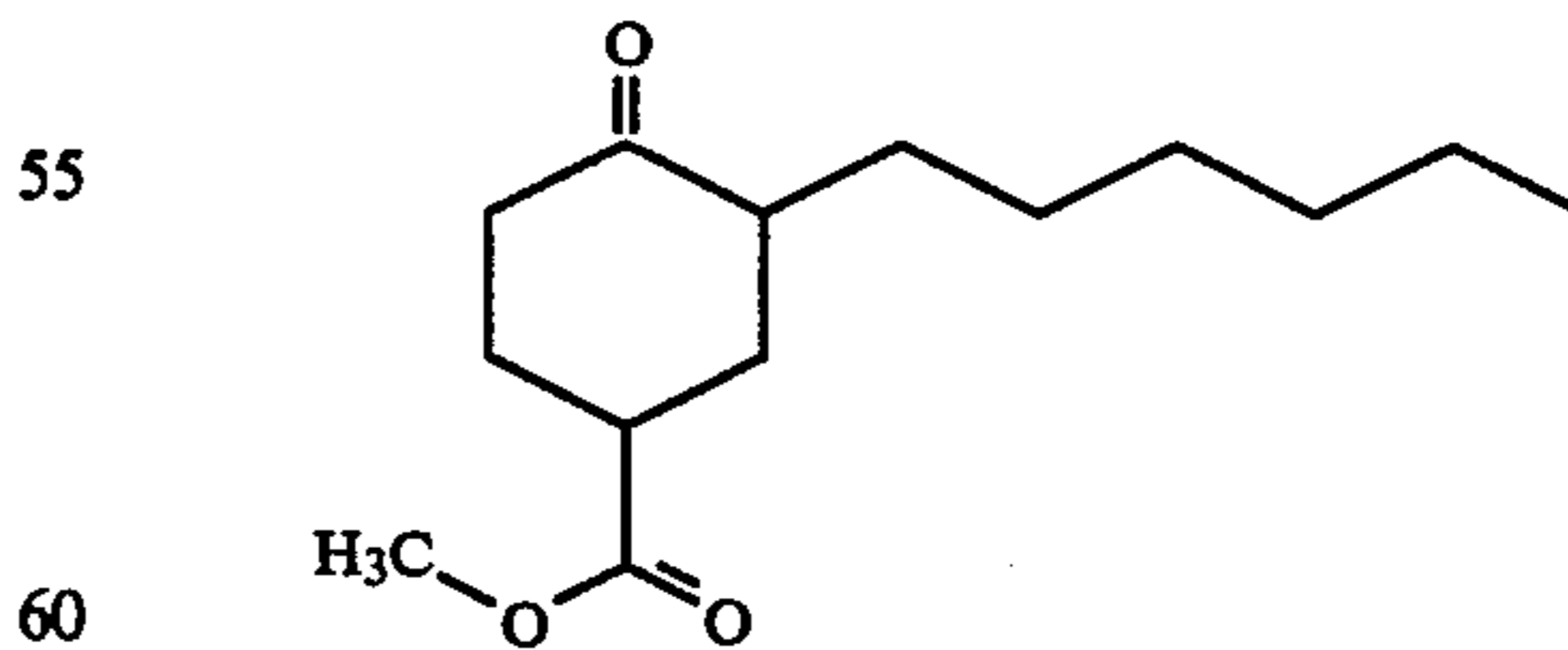
FIG. 13 is the GLC profile for the reaction product of Example V containing the compound having the structure:
