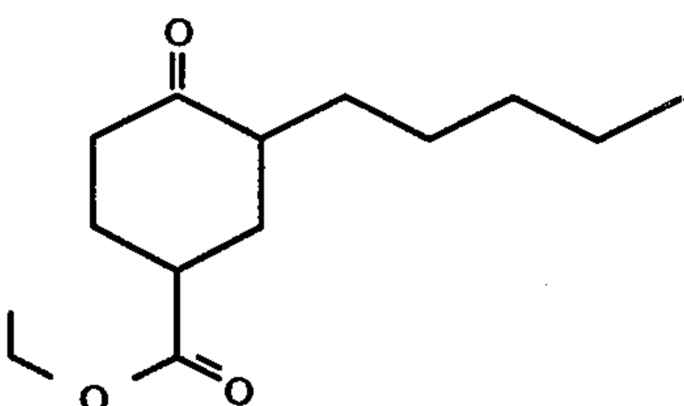
FIG. 13 is the GLC profile for the reaction product of Example V containing the compound having the structure:
