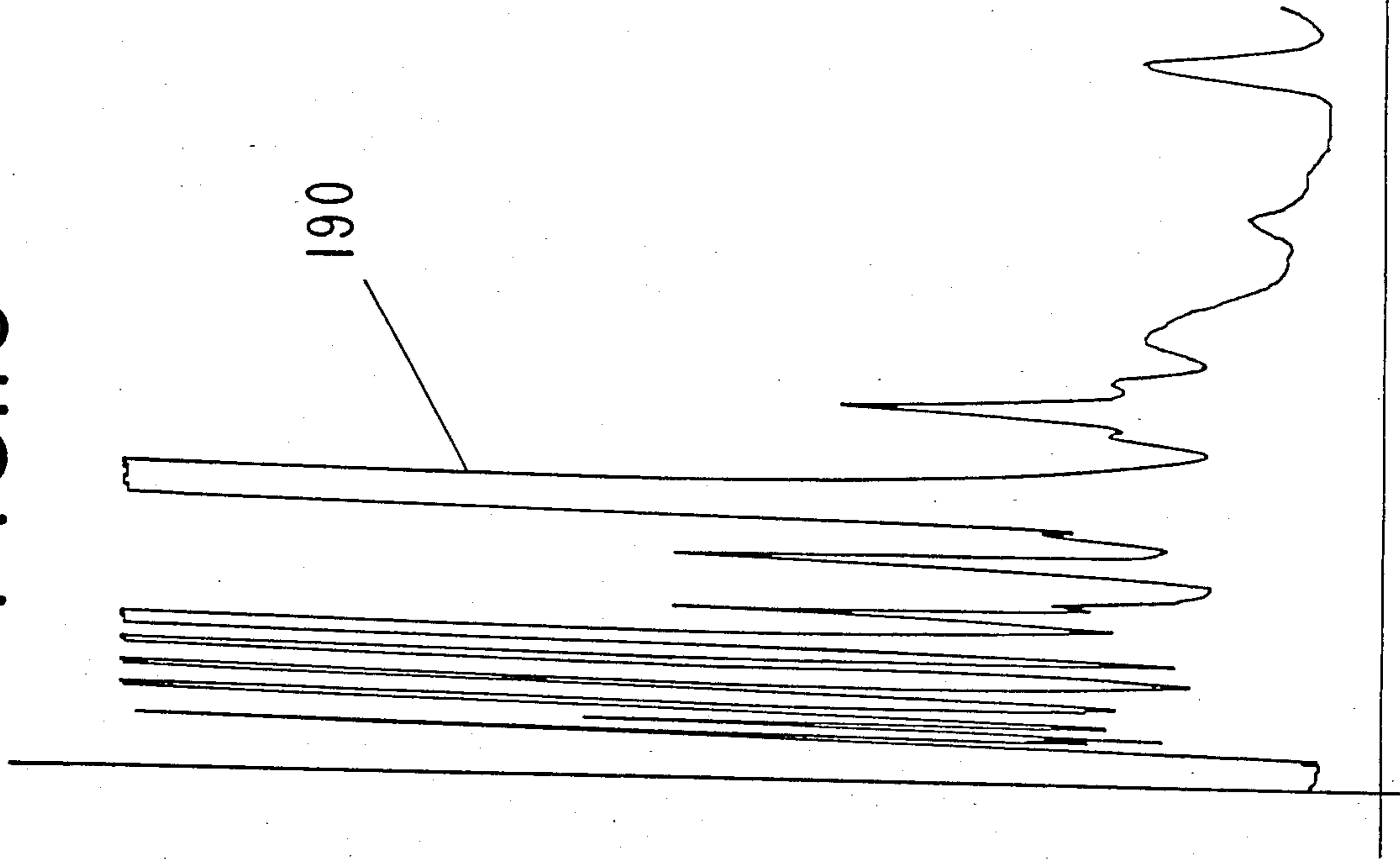
GLC PROFILE FOR EXAMPLE VIII
