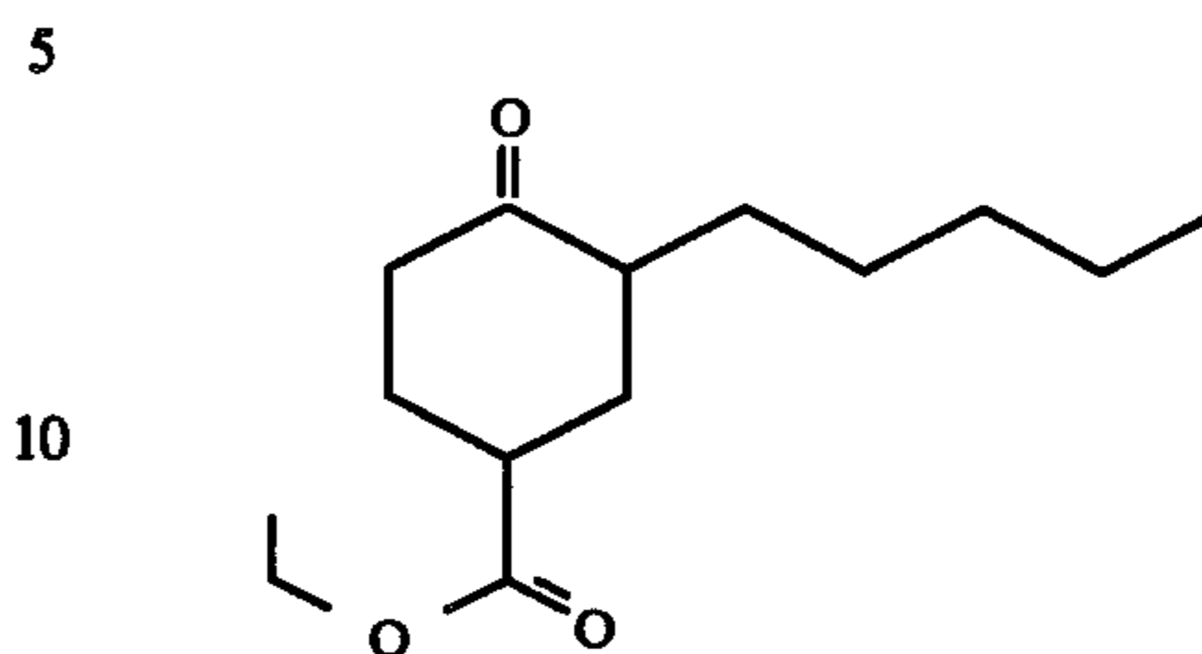
FIG. 10 is the NMR spectrum for the reaction product of Example IV containing the compound having the structure:
