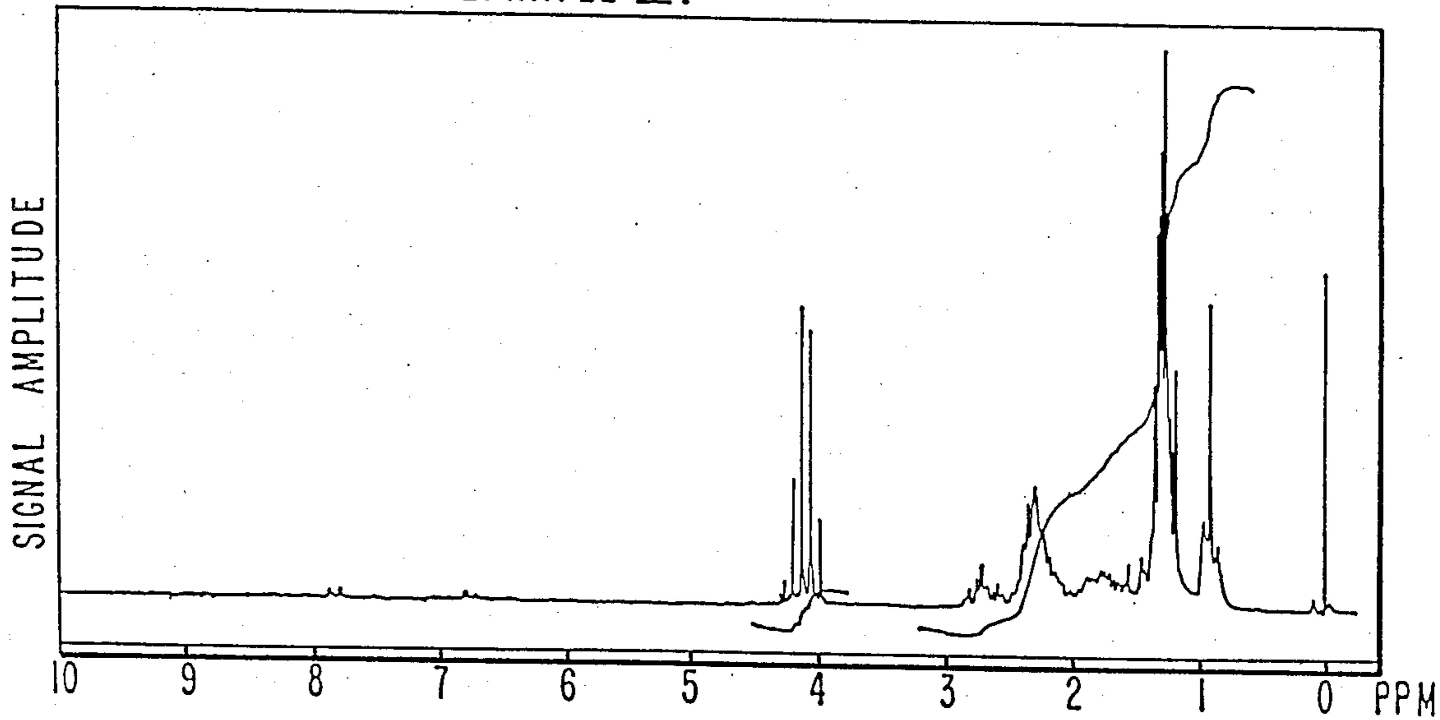
NMR SPECTRUM FOR EXAMPLE V.
