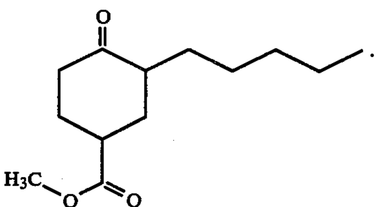
FIG. 12 is the GLC profile for the reaction product of Example V containing the compound having the structure:
