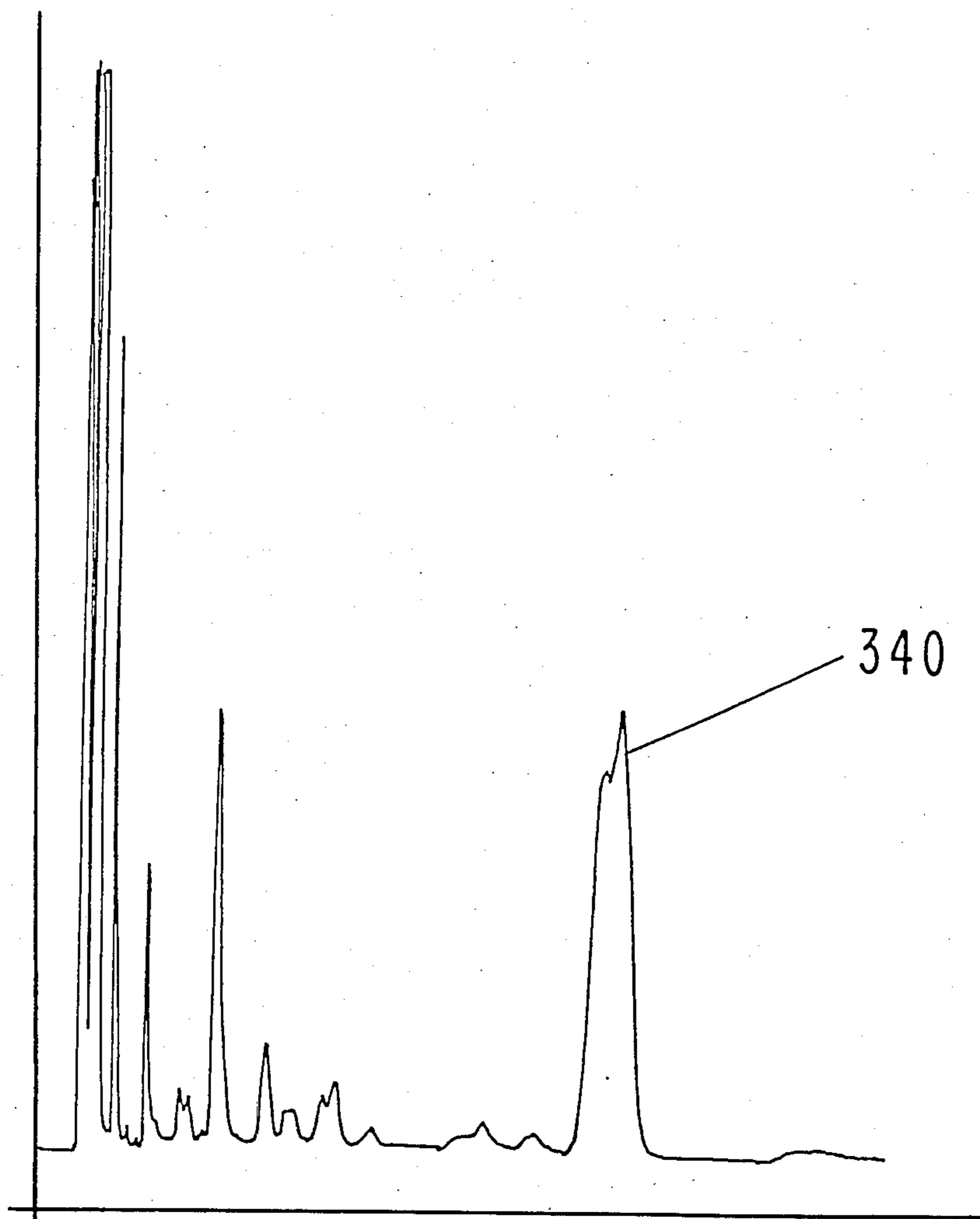
GLC PROFILE FOR EXAMPLE XI (B).
