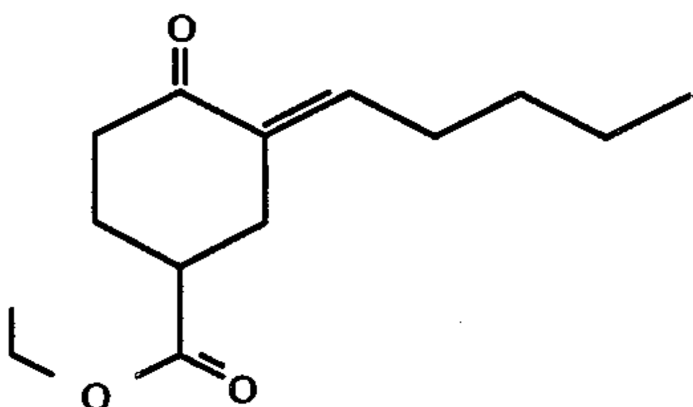
FIG. 12 is the GLC profile for the reaction product of Example V containing the compound having the structure:
