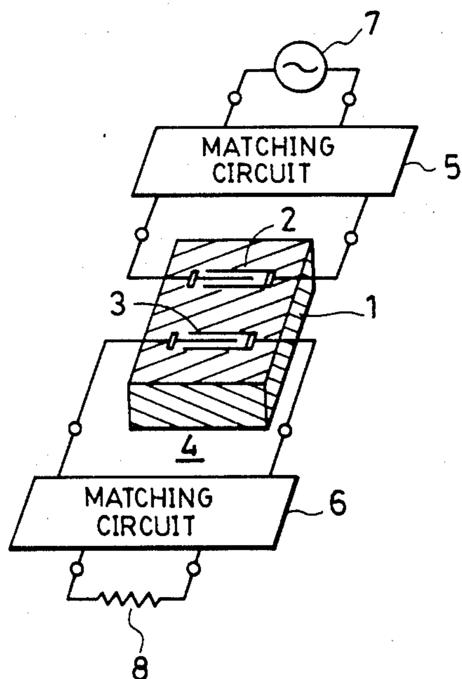
FIG. 1 PRIOR ART
