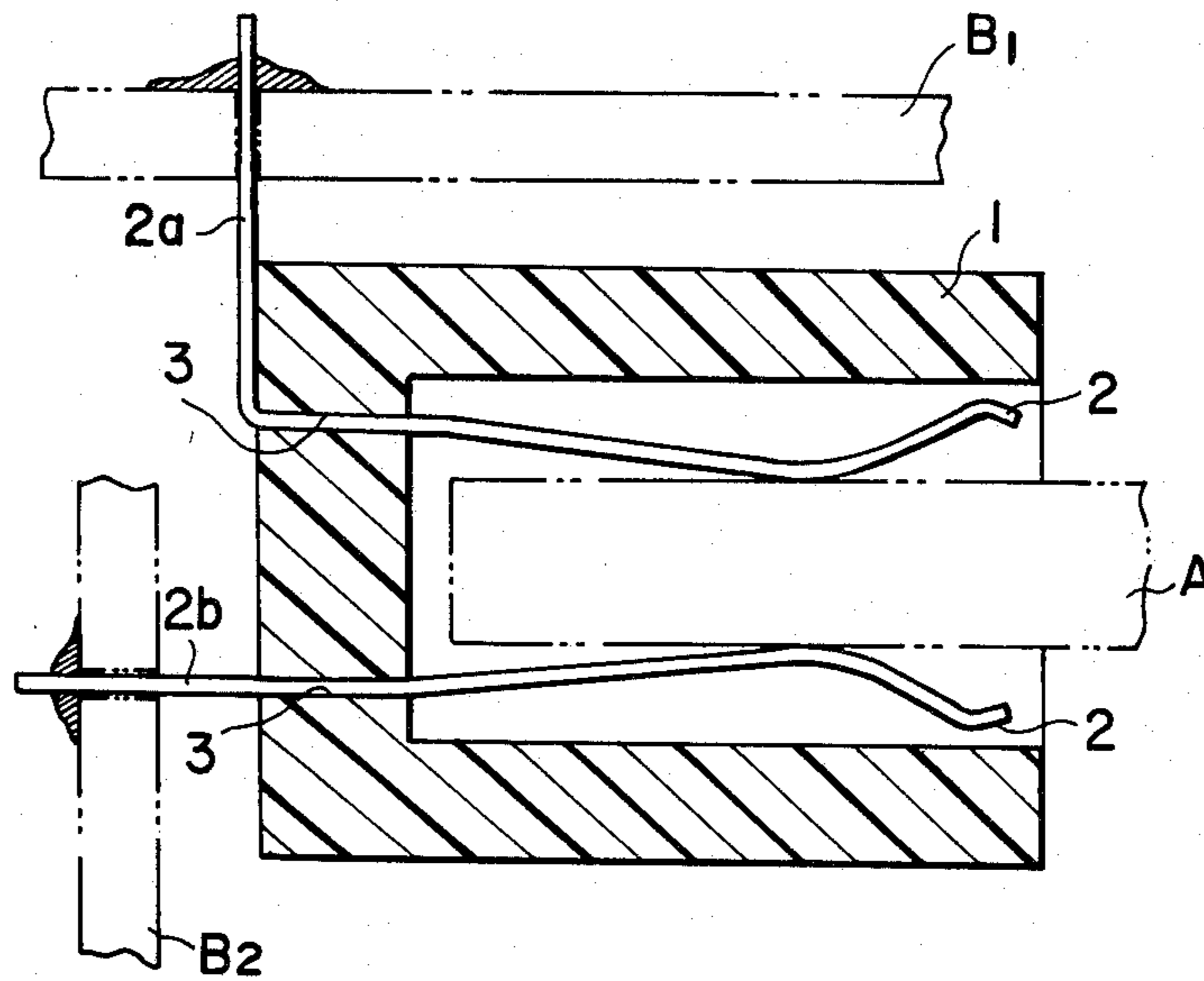
FIG. 1 (PRIOR ART)
