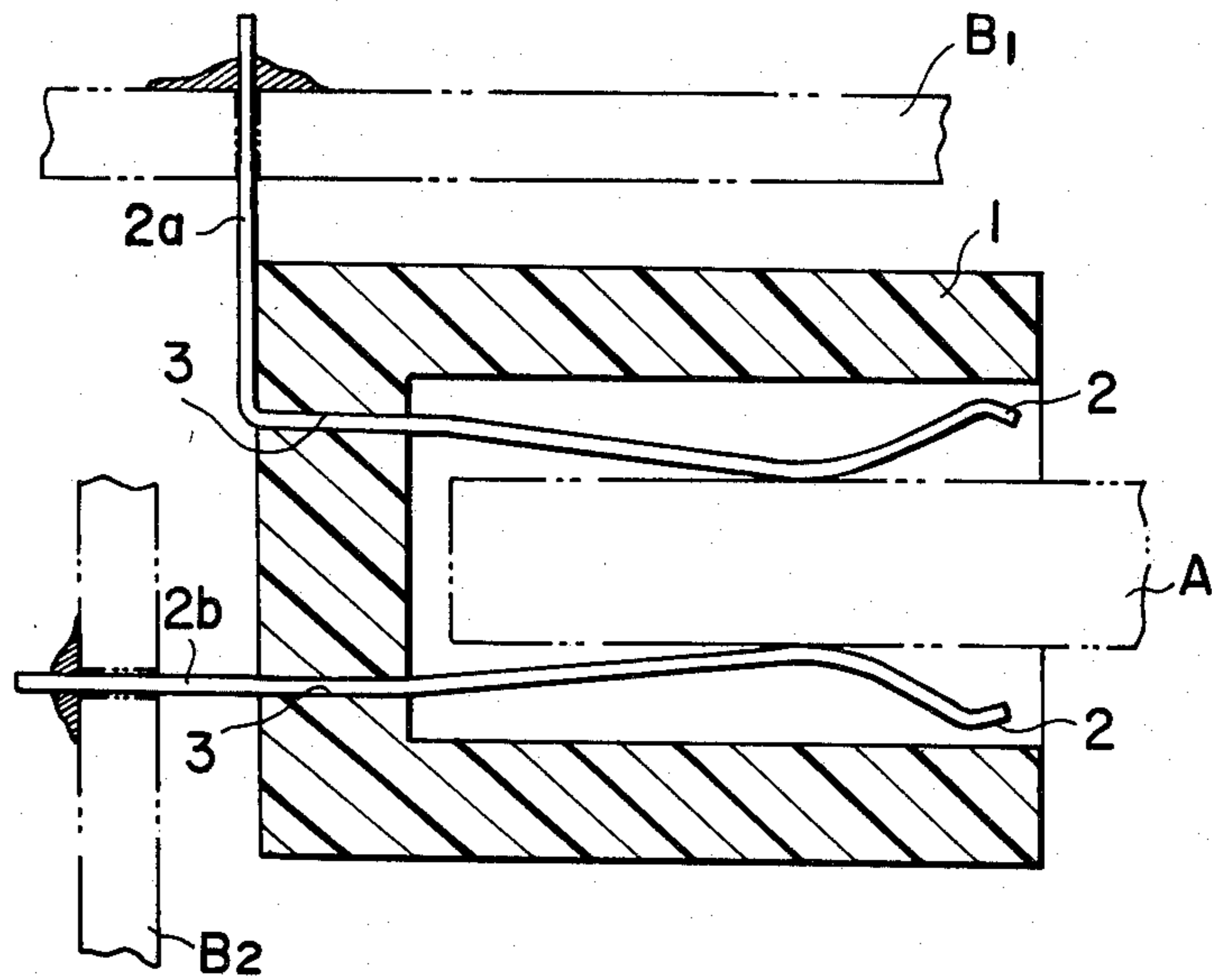
FIG. 1 (PRIOR ART)
