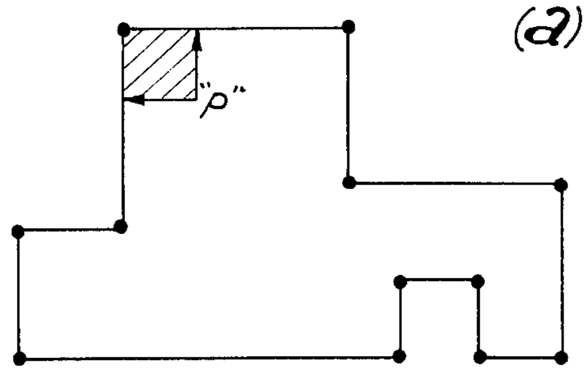
POINT MEMBERSHIP
