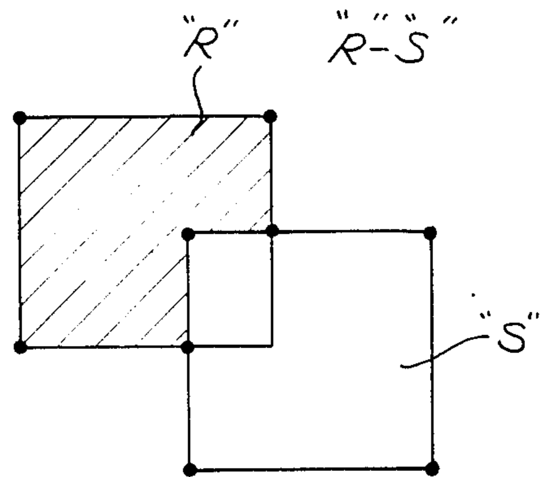
DIFFERENCE
