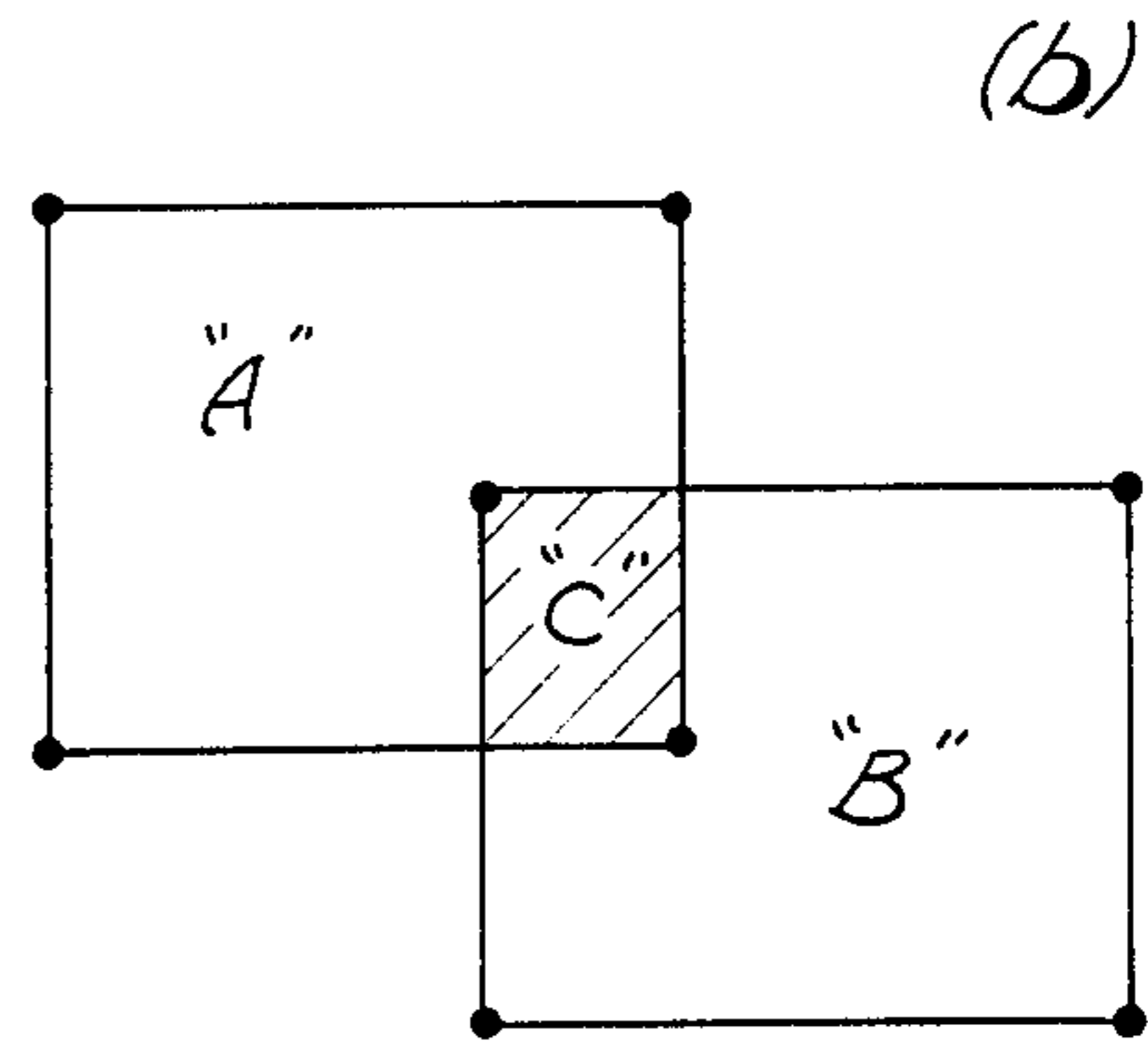
INTERSECTION
