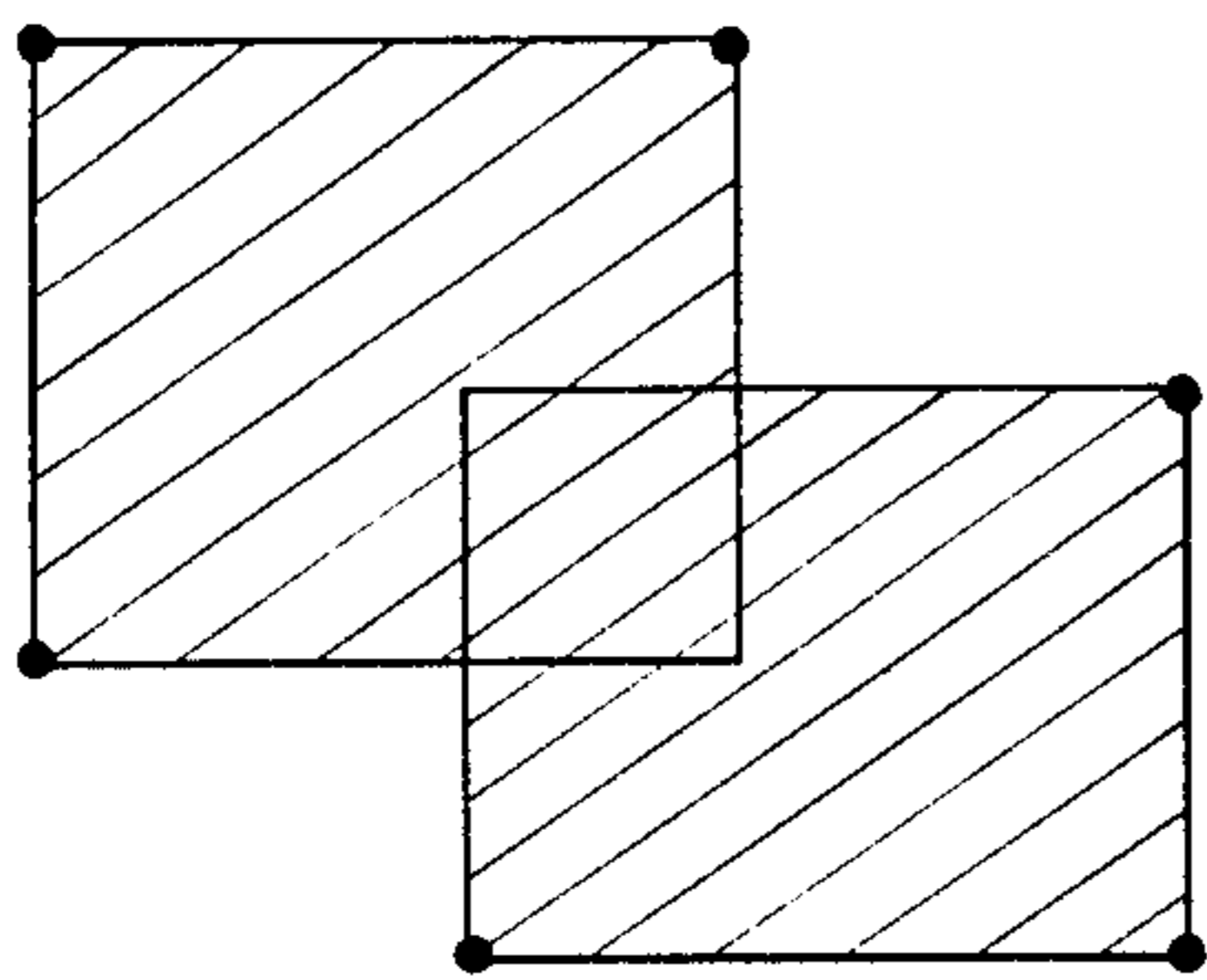
UNION
