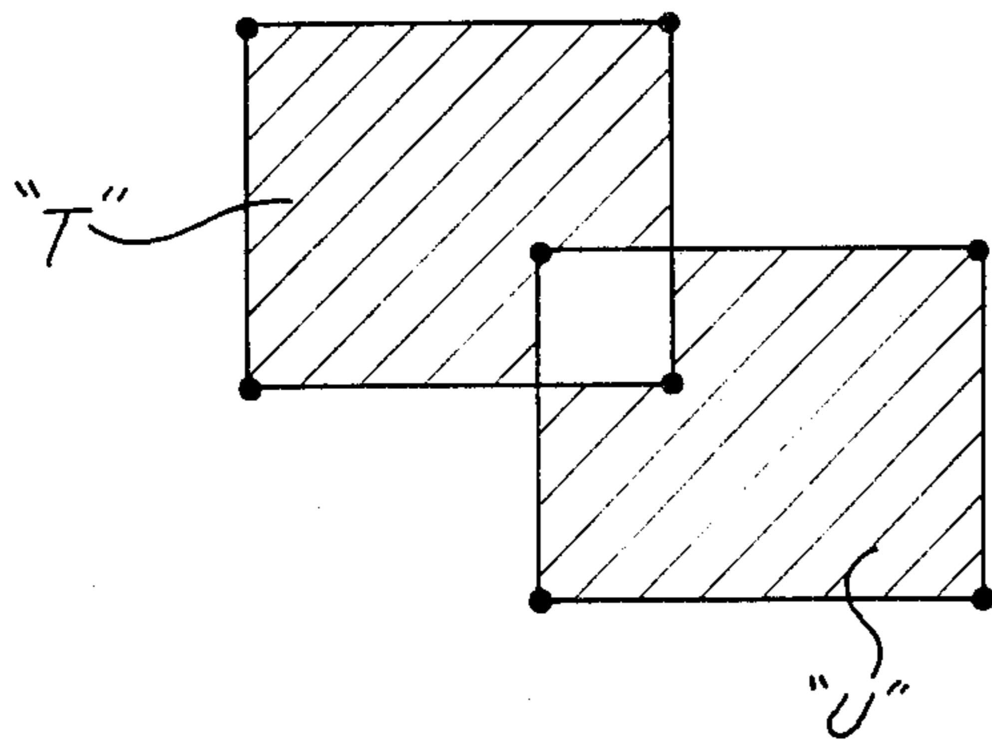
EXCLUSIVE - OR
