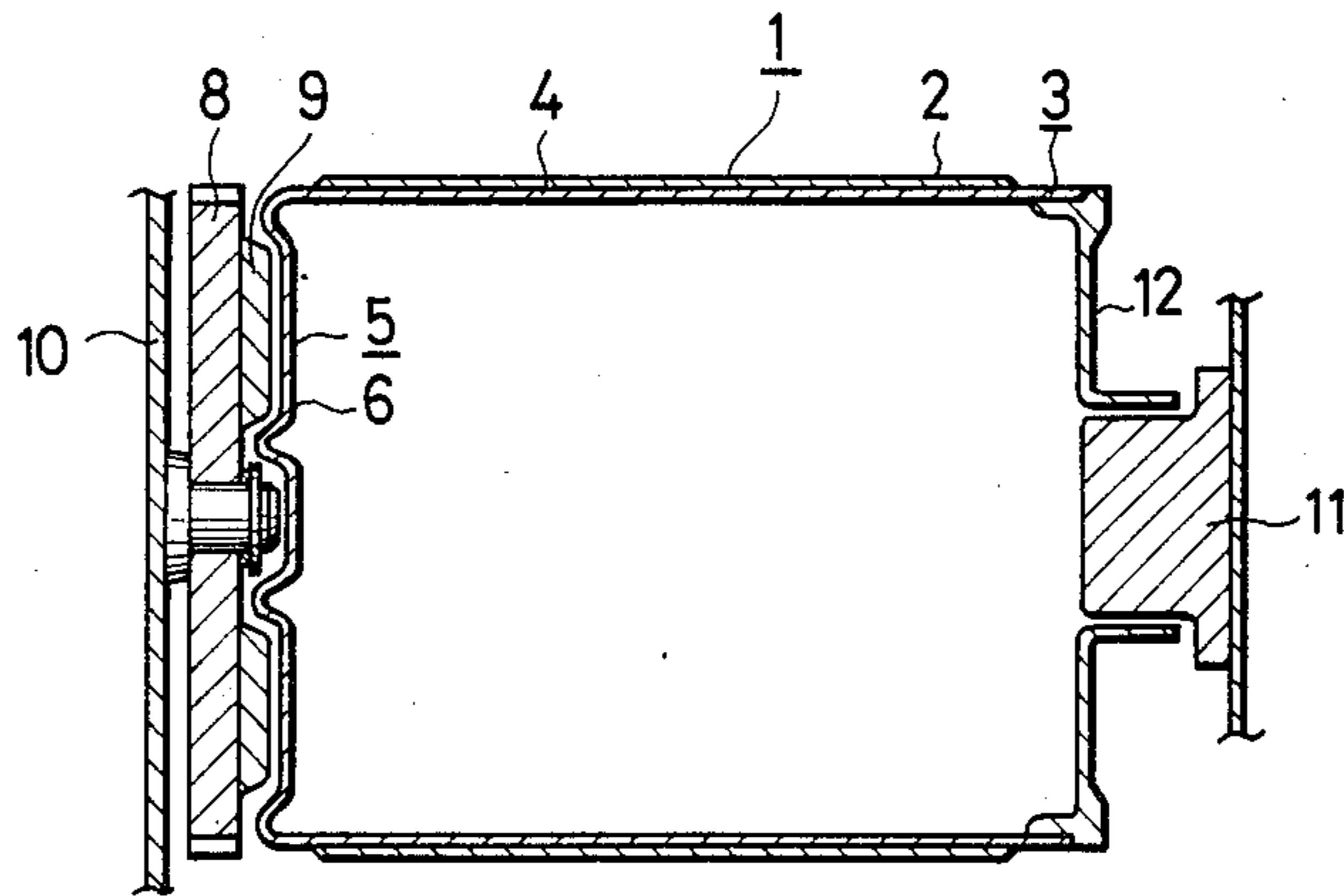
FIG. 1 PRIOR ART
