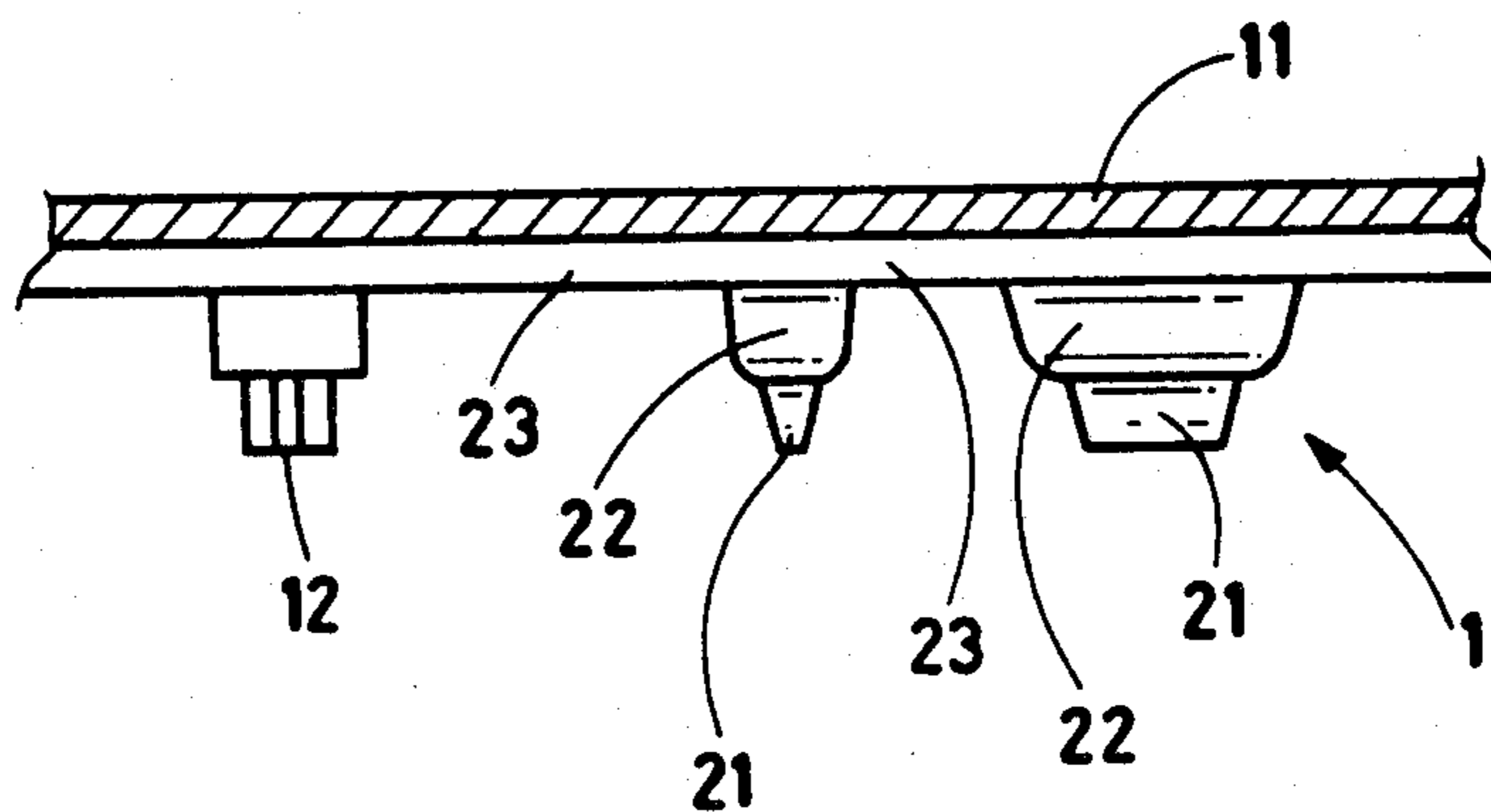
FIG. 11 PRIOR ART
