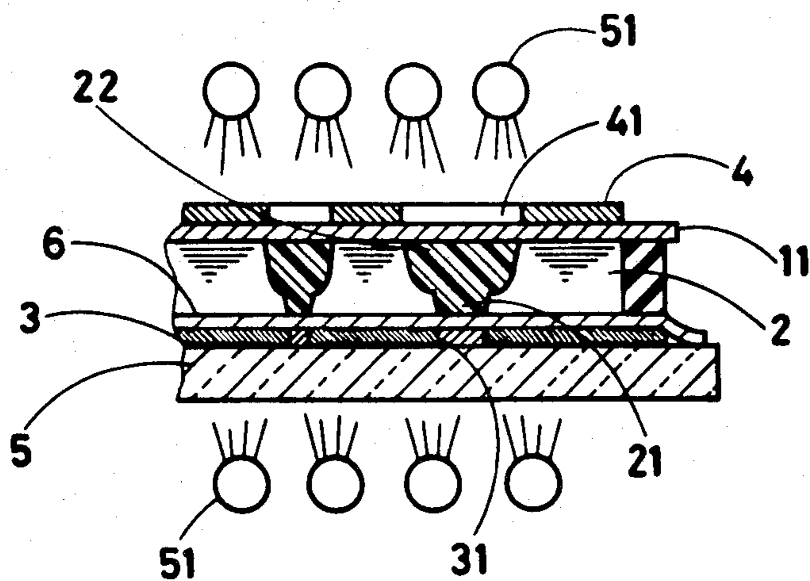
FIG. 9 PRIOR ART
