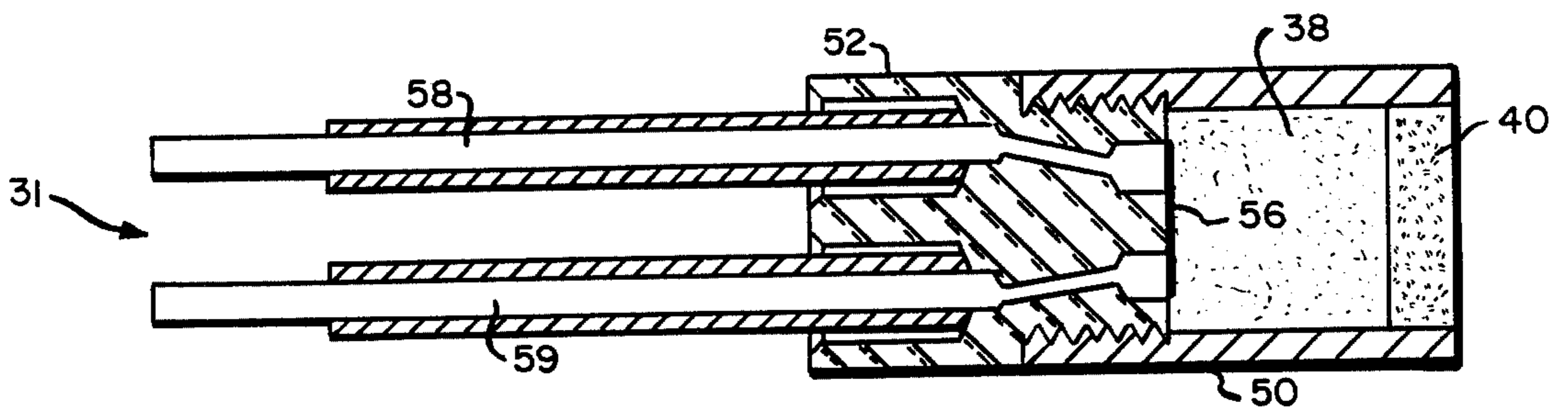
FIG. 3 (PRIOR ART)
