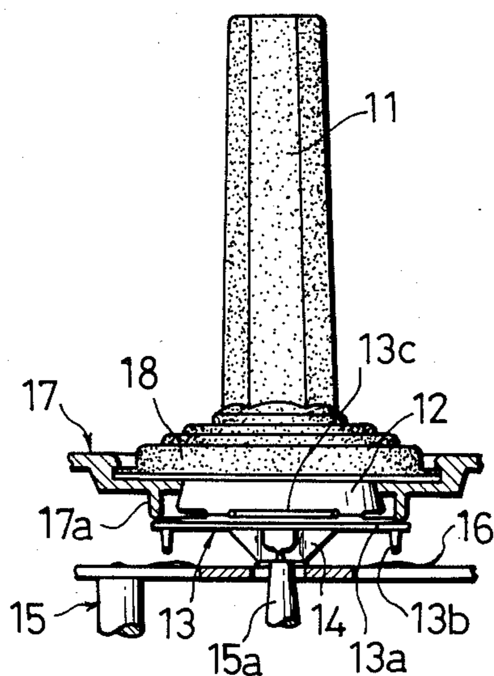
Fig. 5 PRIOR ART
