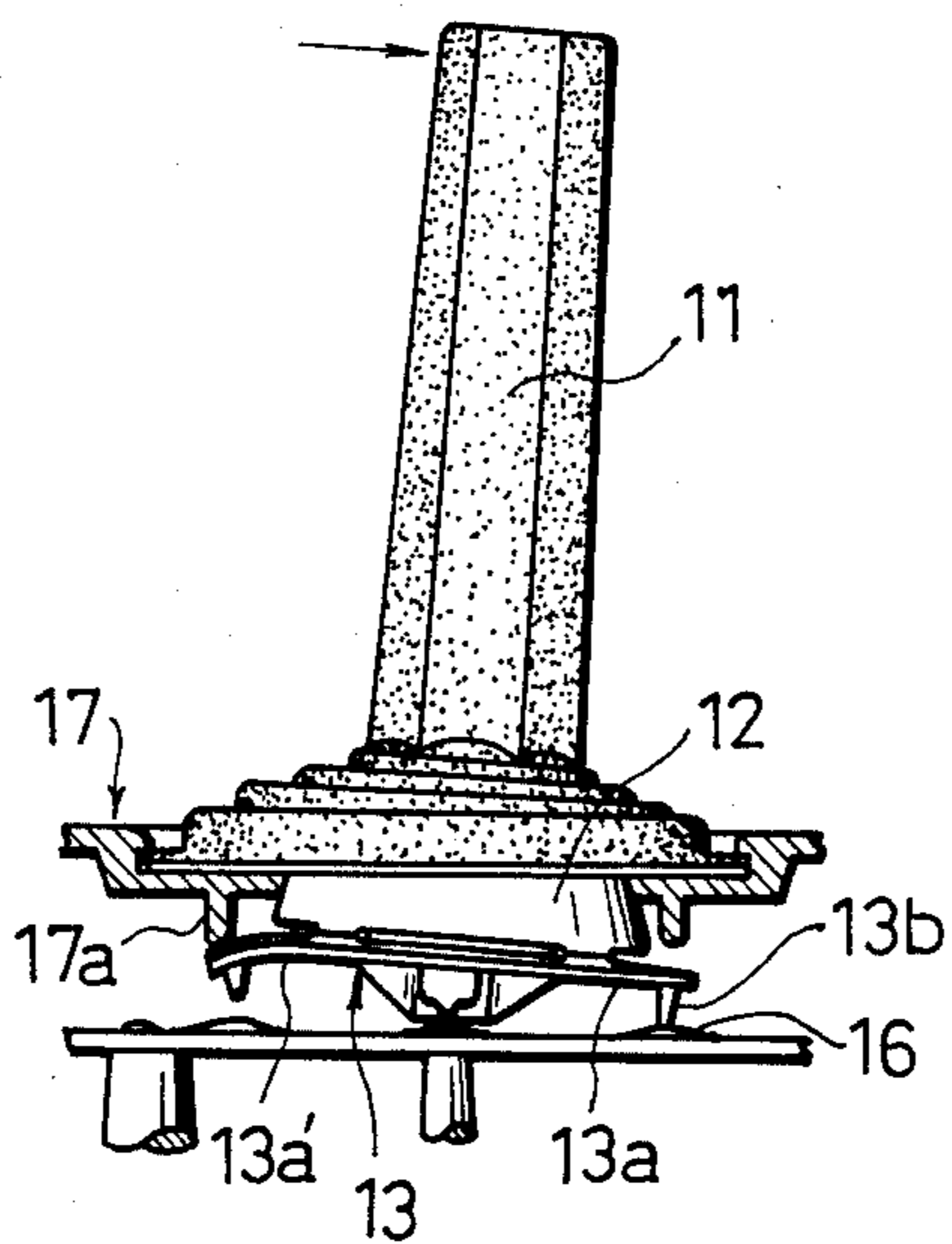
Fig. 5 PRIOR ART
