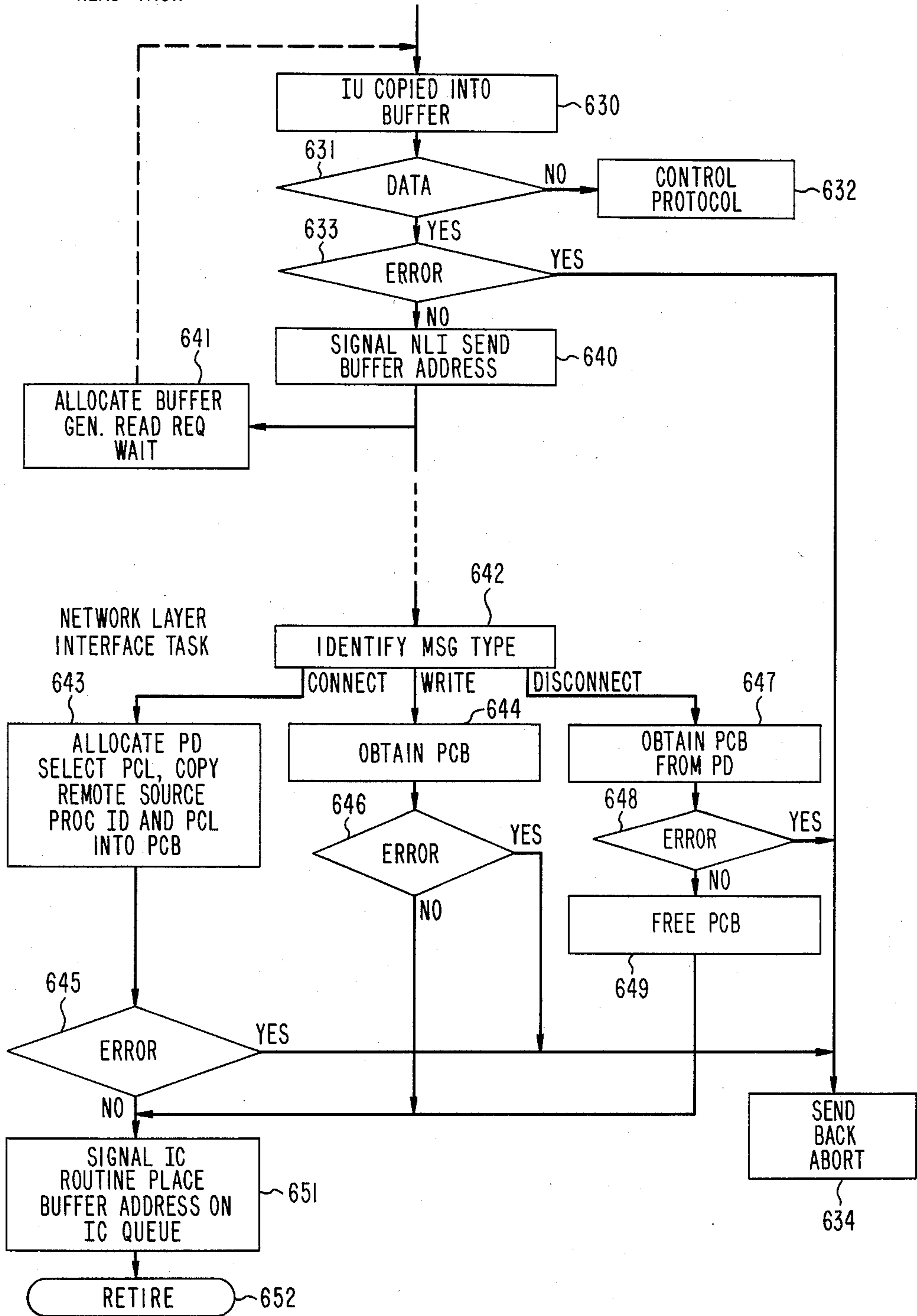
FIG. 38 INTERPROCESSOR INTERFACE PROCESS READ TASK FROM PCL
