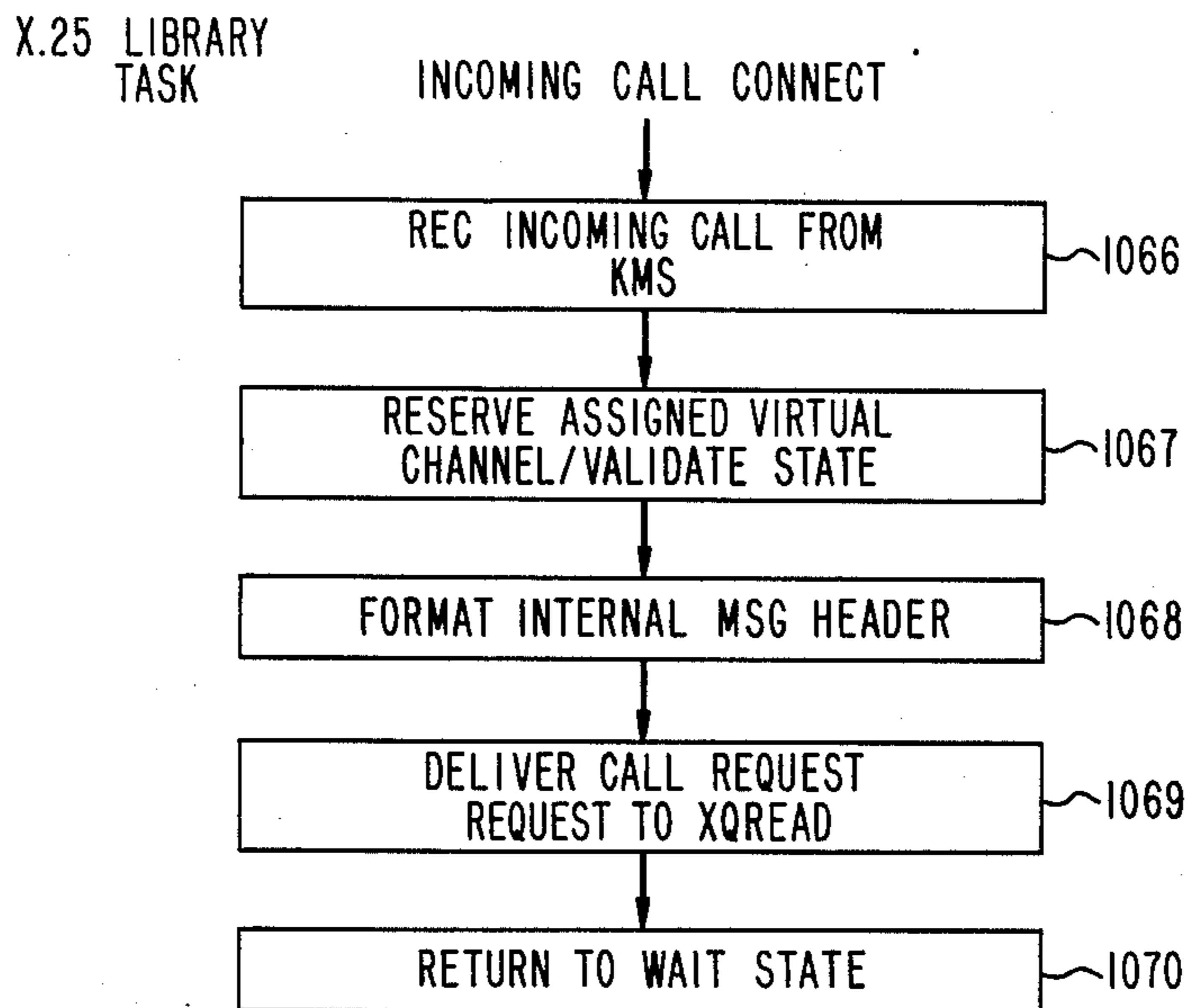
FIG. 45 TRANSPORT NETWORK INTERFACE PROCESS
