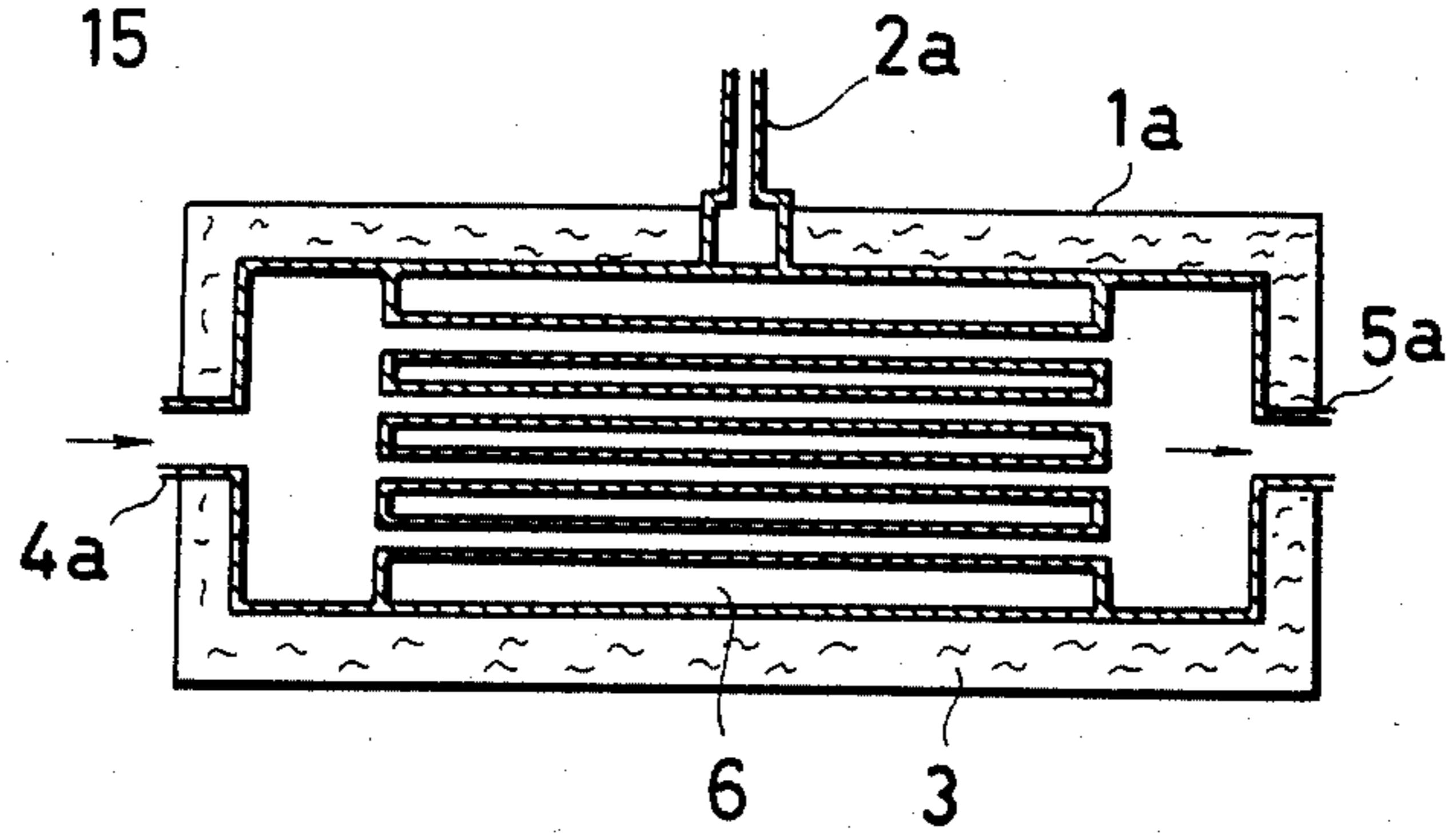
FIG. 12 (PRIOR ART)
