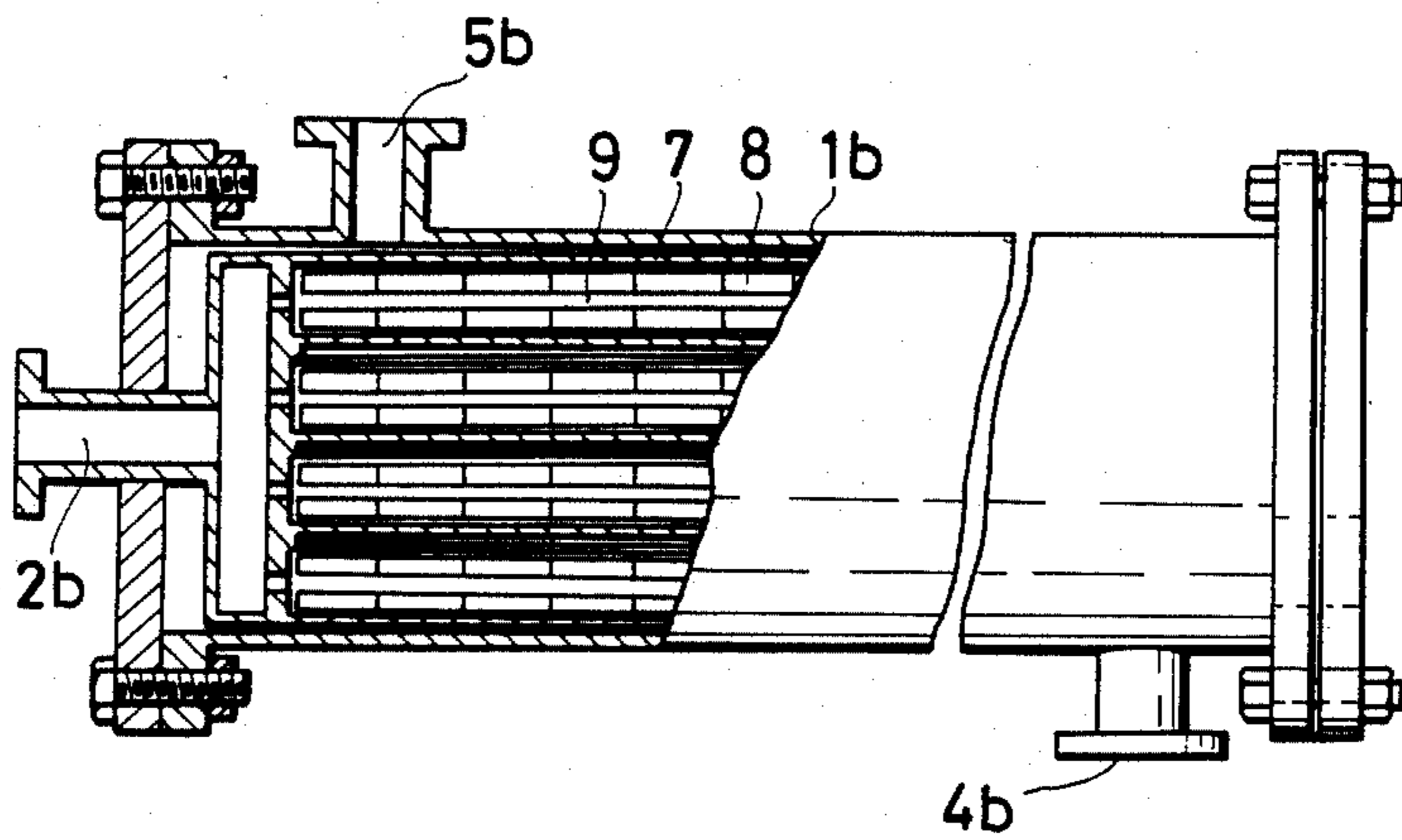
FIG. 13 (PRIOR ART)
