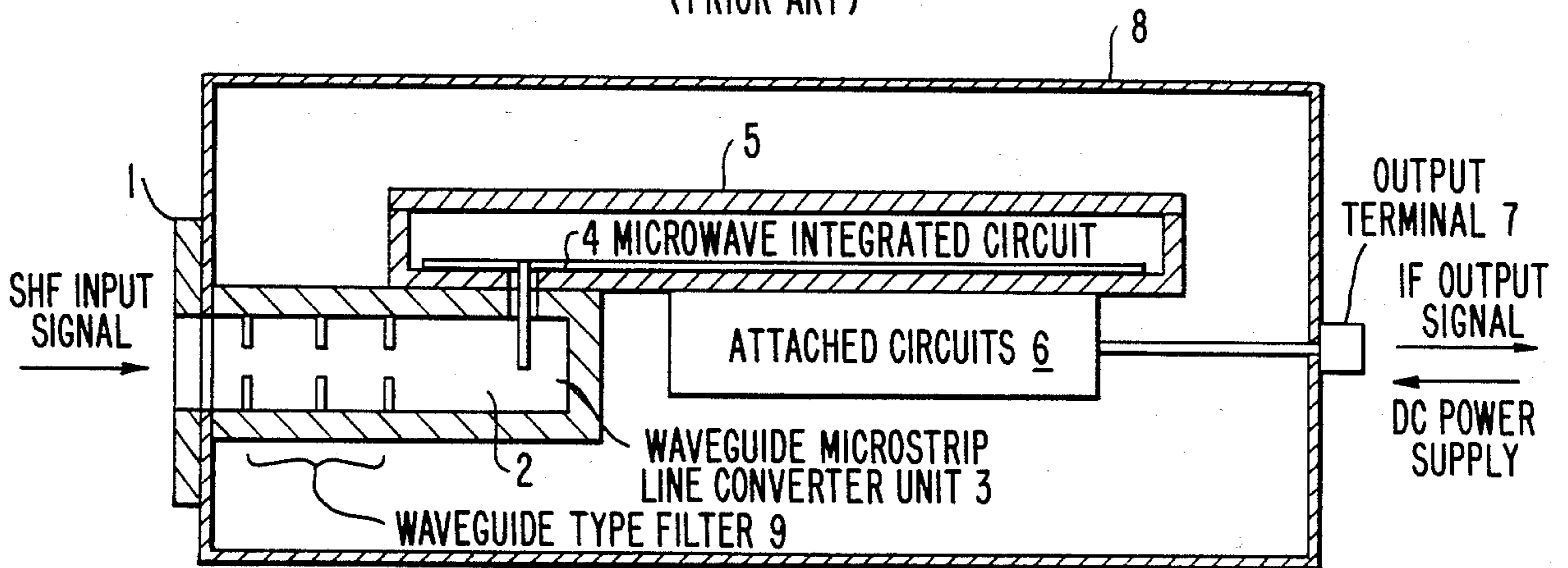
FIG. 2. (PRIOR ART)
