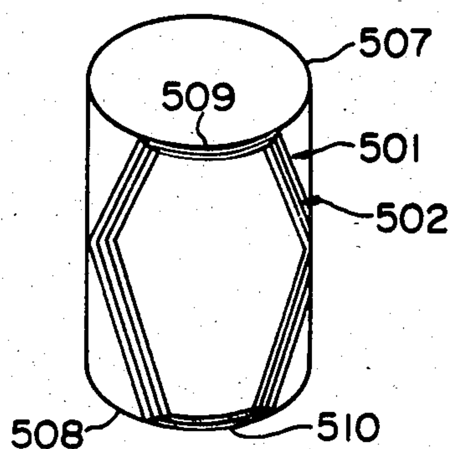
FIG. 38 PRIOR ART
