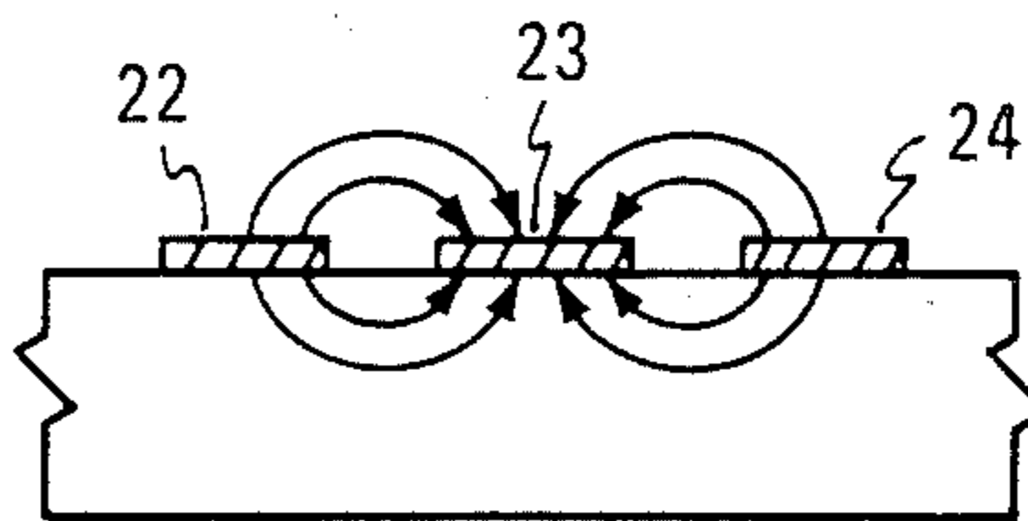
FIG. 3B COPLANAR LINE
