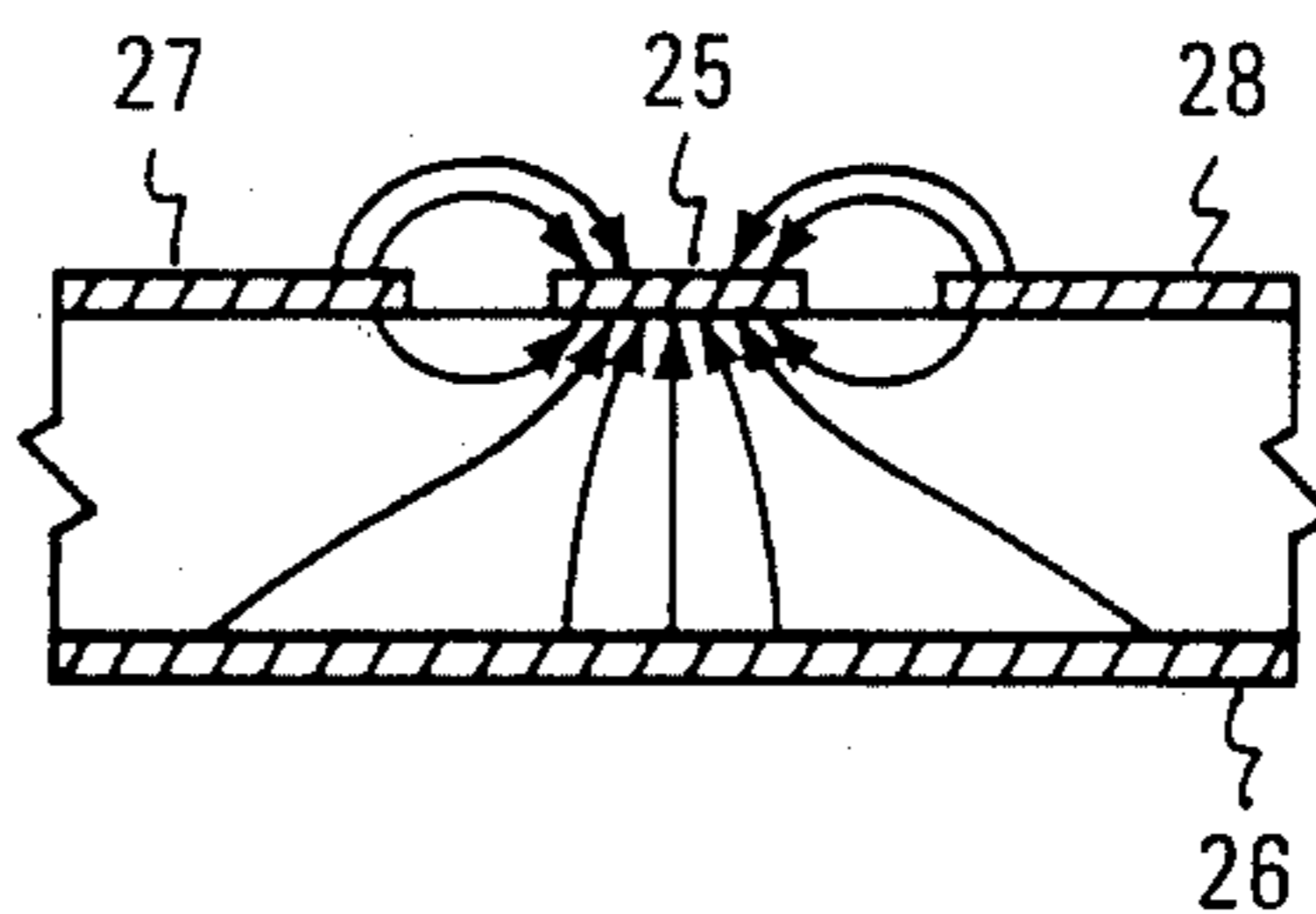
FIG. 3C COPLANAR LINE TO MICROSTRIP TRANSITION
